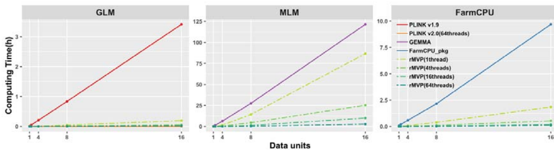
Figure 2. Comparison of computing speed of PLINK, GEMMA, FarmCPU_pkg, and rMVP (“Speed” mode)
