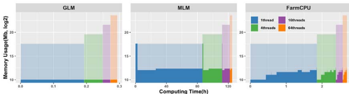
Figure 1. Comparison of memory usage in response to number of threads used for parallel computation under “speed” mode of rMVP.
