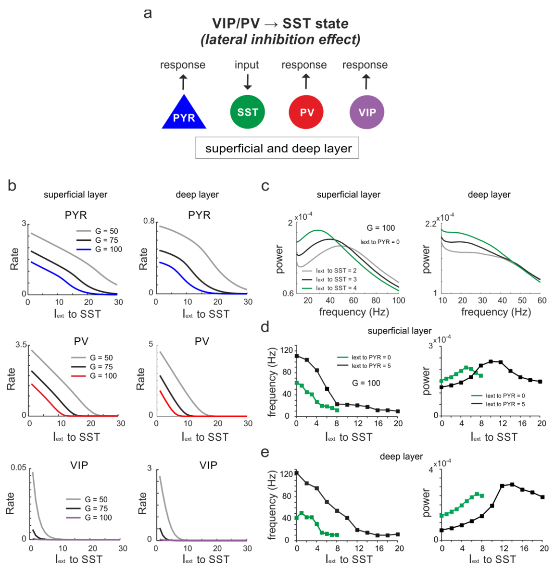
Figure 5. Lateral inhibition switches dynamics from VIP/PV to SST dominated states. a) Schematic showing input to SST cells in both layers and measuring response in all other cell types. b) Response curves of PYR, PV and VIP cells as a function of SST drive for superficial and deep layers, and three different values of G . c) Power spectra of superficial and deep layers for different levels of SST input. d) Peak frequency and power as a function of SST input for two levels of PYR drive. e) Same as in d) for the deep layer.
