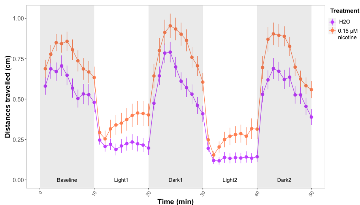
Figure 5. Forced light/dark test in wild type zebrafish exposed to 0.15 µM nicotine. Sample size: n=48 for each dose group. Each dot represents mean of the total distance travelled per minute. Error bars represent \pm SEM.
