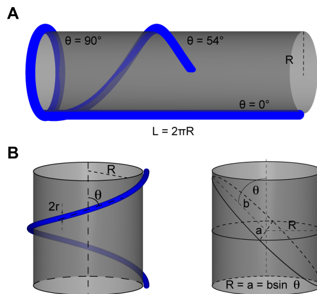
Fig S4. Tubular structure elliptical profile approximation.
