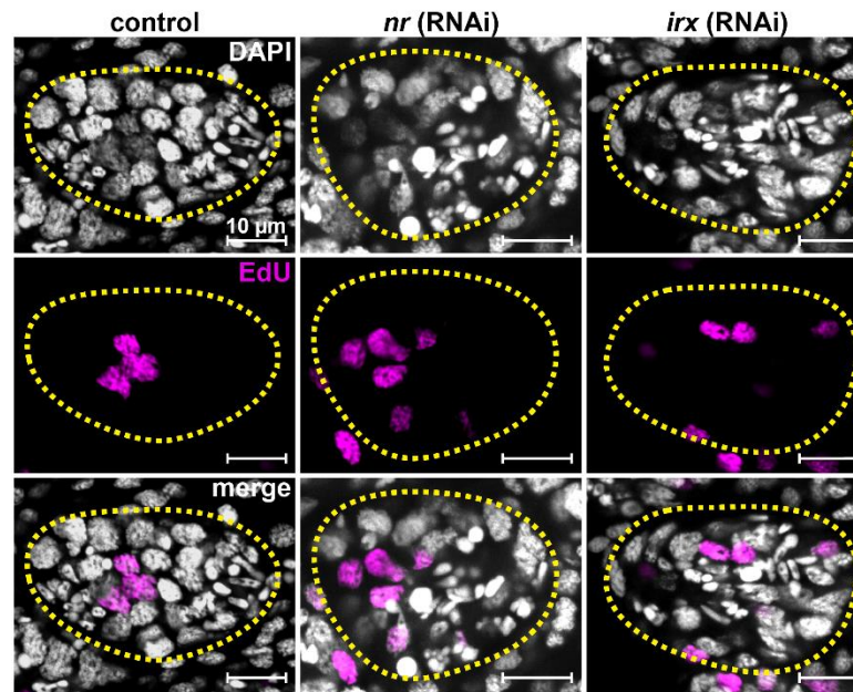
Supplementary Fig. 4: RNAi of irx and nr did not cause any noticeable phenotype.
