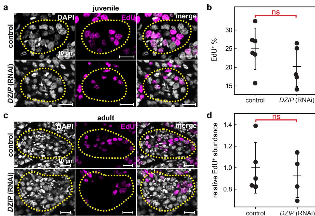
Supplementary Fig. 5: DZIP RNAi did not cause any noticeable phenotype in either juvenile or adult parasites.
