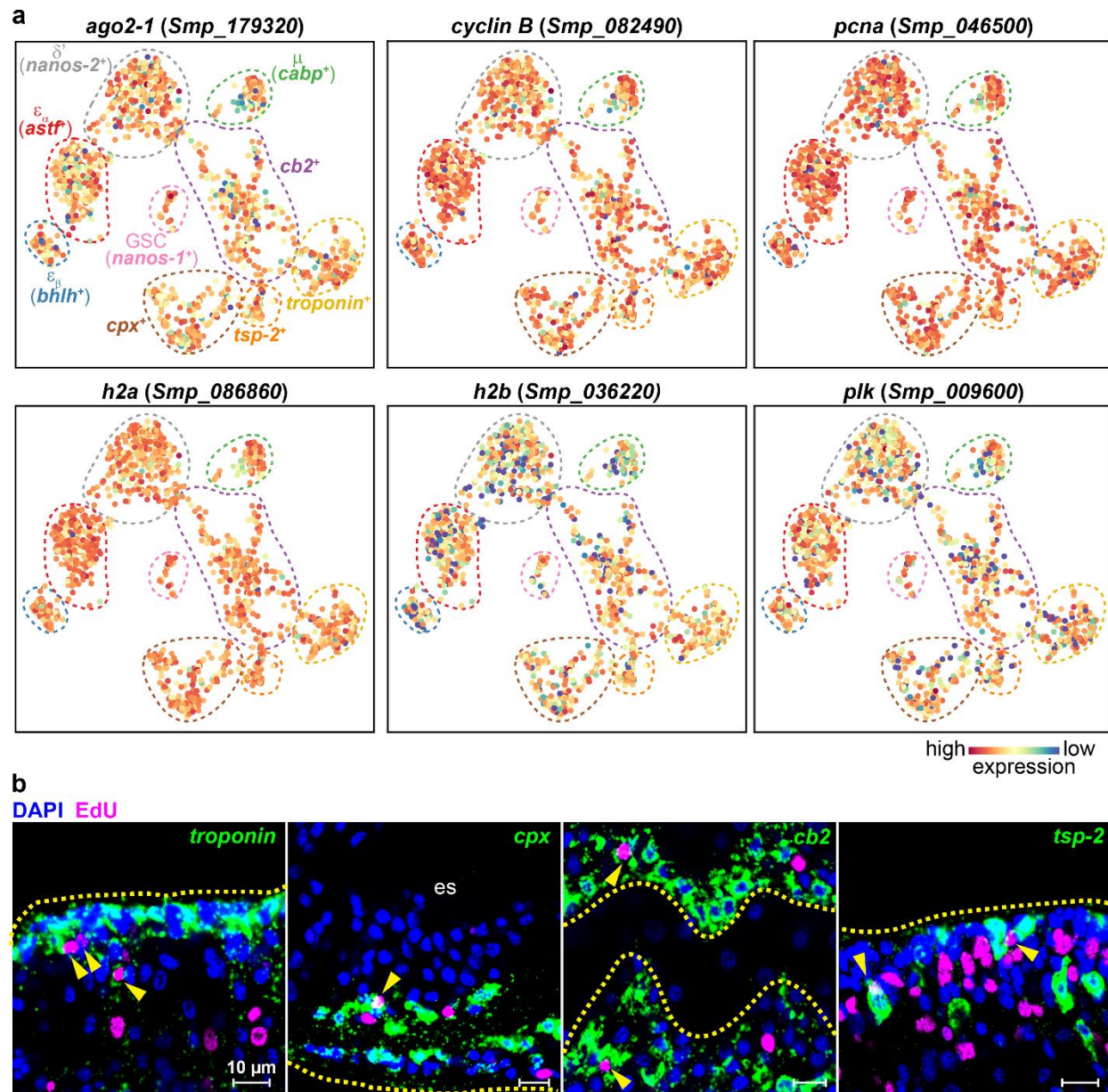
Supplementary Fig. 1: Characterization of presumptive progenitor populations.
