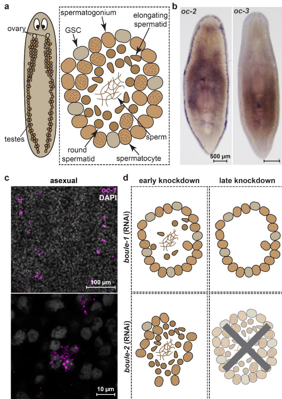
Supplementary Fig. 7: Expression of planarian oncut homologs.
