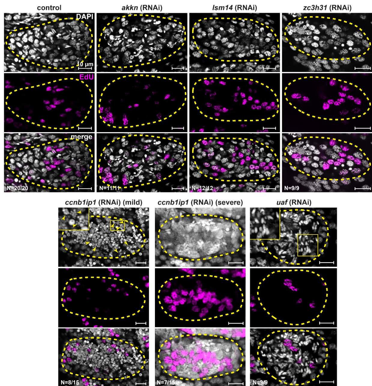
Supplementary Fig. 6: RNAi phenotypes of GSC regulators in adult parasites.
