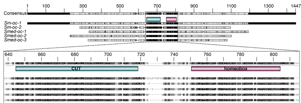
Supplementary Fig. 2: Sequence alignment of onecut transcription factors identified in the S. mansoni and S. mediterranea genomes.
