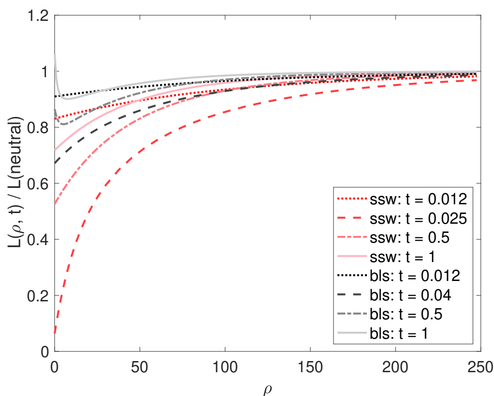
Figure S8: Comparing recent balancing selection with the corresponding sweep model with respect to their effects on diversity levels in surrounding genomic regions. The models and their parameters are the same as those in Figure 9, except that n = 20 .
