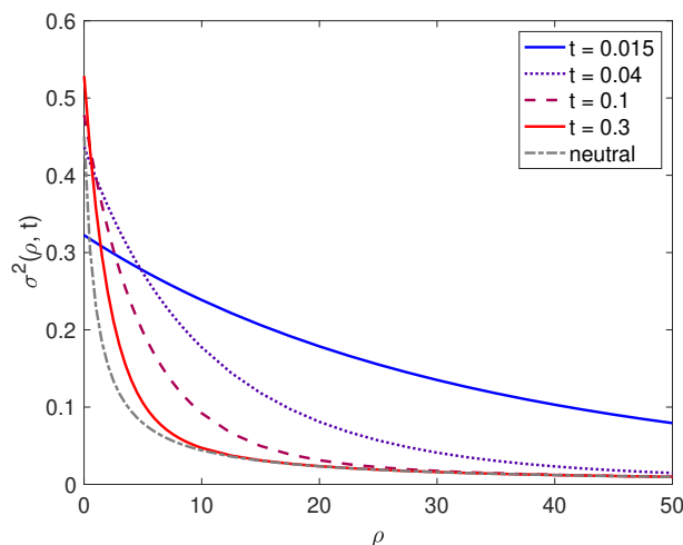
Figure 8 Nucleotide site diversity and LD in genomic regions surrounding a recently-emerged variant under balancing selection. The parameters are \gamma_1 = 500 and \hat{p}_2 = 0.75 (as in Figure 6). The discretisation scheme has H = 76 bins. In (a), the expected total branch length for a sample of n = 2 alleles is calculated for various value of t , the time since the frequency of A_2 reaches \epsilon . To make the effects more visible, L is divided by its neutral expectation. \sigma^2 in (b) measures the level of LD between the selected locus and a linked neutral site. For comparison, the neutral expectation of \sigma^2 is also included.
