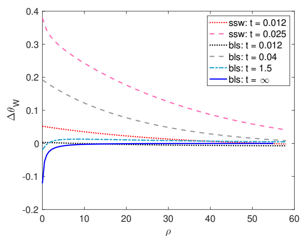
Figure 11 \Delta\theta_W as a function of \rho and t . The two selection models are the same as those considered in Figure 10. "bls: t = \infty " corresponds to the equilibrium under balancing selection. The sample size is 10.
