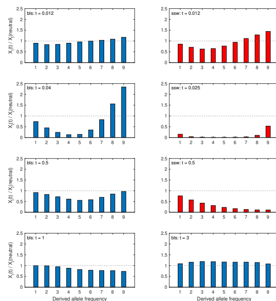
Figure 10 The SFS at various time points after the arrival of the selected variant for a random sample of 10 alleles. The balancing selection (bls) and selective sweep (ssw) models are the same as those shown in Figure 9. The scaled distance between the focal neutral site and the selected site is \rho = 2 . The reduction in diversity reaches its maximum at t \approx 0.04 and 0.025 (fixation) under the balancing selection and selective sweep models, respectively. The SFS under selection is expressed relative to its neutral expectation.
