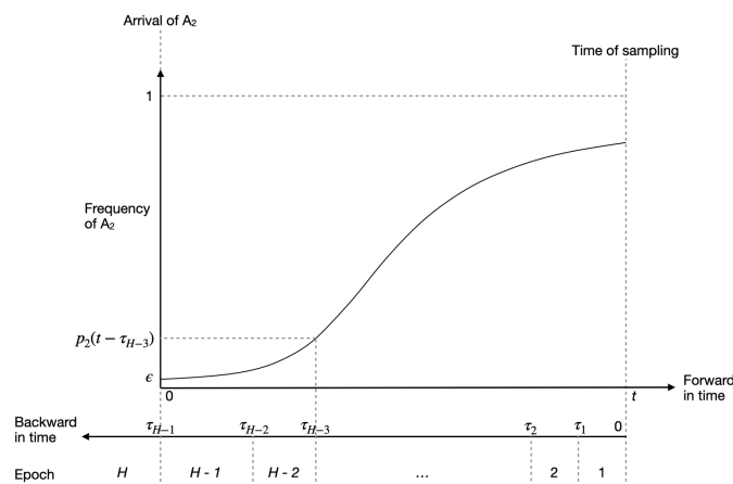
Figure 7 A diagram showing the discretisation scheme used to obtain the expected total branch length and the site frequency spectrum under the model of recent balanced polymorphism.
