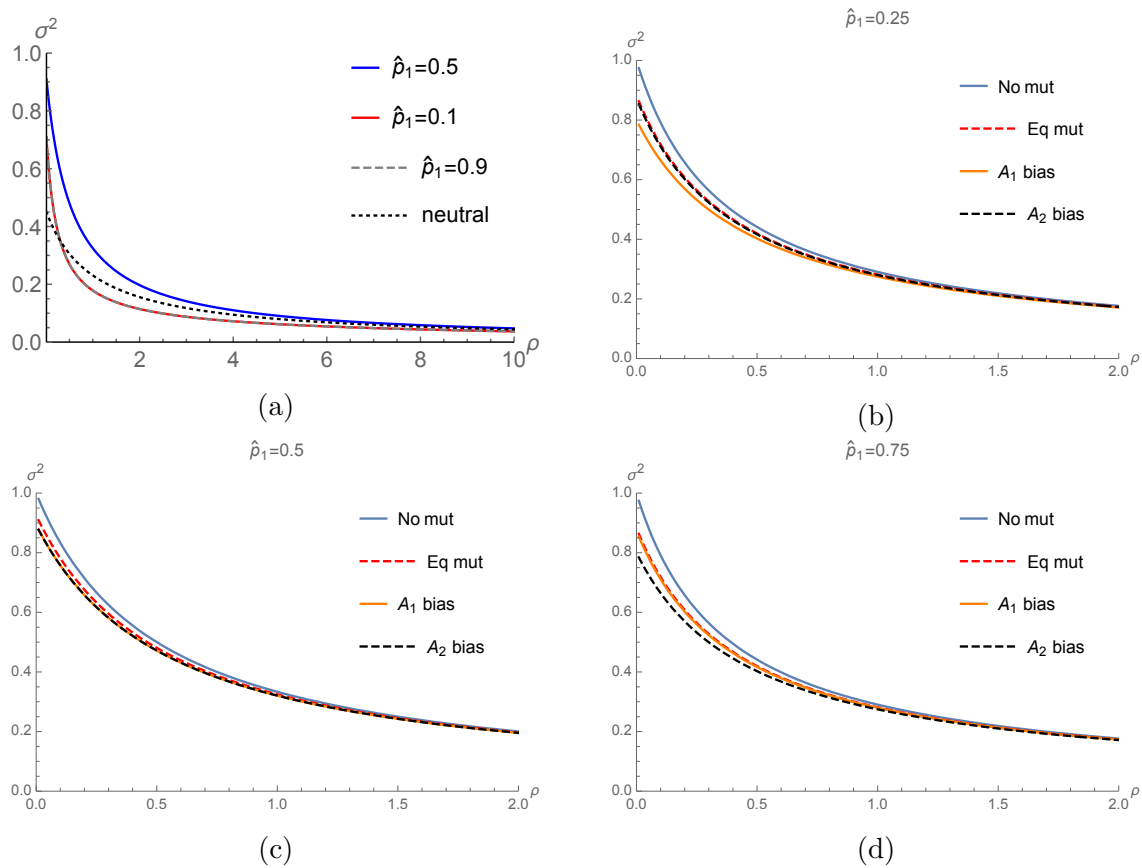
Figure S3: The level of LD between the selected and neutral loci as a function of \rho . In (a), the mutation rates between A_1 and A_2 are \mu_{12} = \mu_{21} = 0.02 . In (b) - (d), for a given \hat{p}_1 , different mutation rates are considered. “No mut” means \mu_{ij} = 0 . “Eq mut” means \mu_{ij} = 0.02 . “ A_1 bias” means \mu_{12} = 0.01 and \mu_{21} = 0.05 . “ A_2 bias” means \mu_{12} = 0.05 and \mu_{21} = 0.01 .
