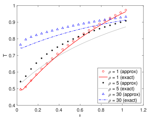
Figure 12 Comparing expected pairwise coalescence times obtained by phase-type theory (exact) and an approximation assuming low recombination rates. The model of recent balancing selection model has the following parameters: \gamma_1 = 500 and \beta_2 = 0.75 (i.e., the same as in Figures 8 - 11). t is the time since the arrival of A_2 . The discretisation scheme has H = 76 epochs. Details of the approximation are given in Supplementary Text S.5.
