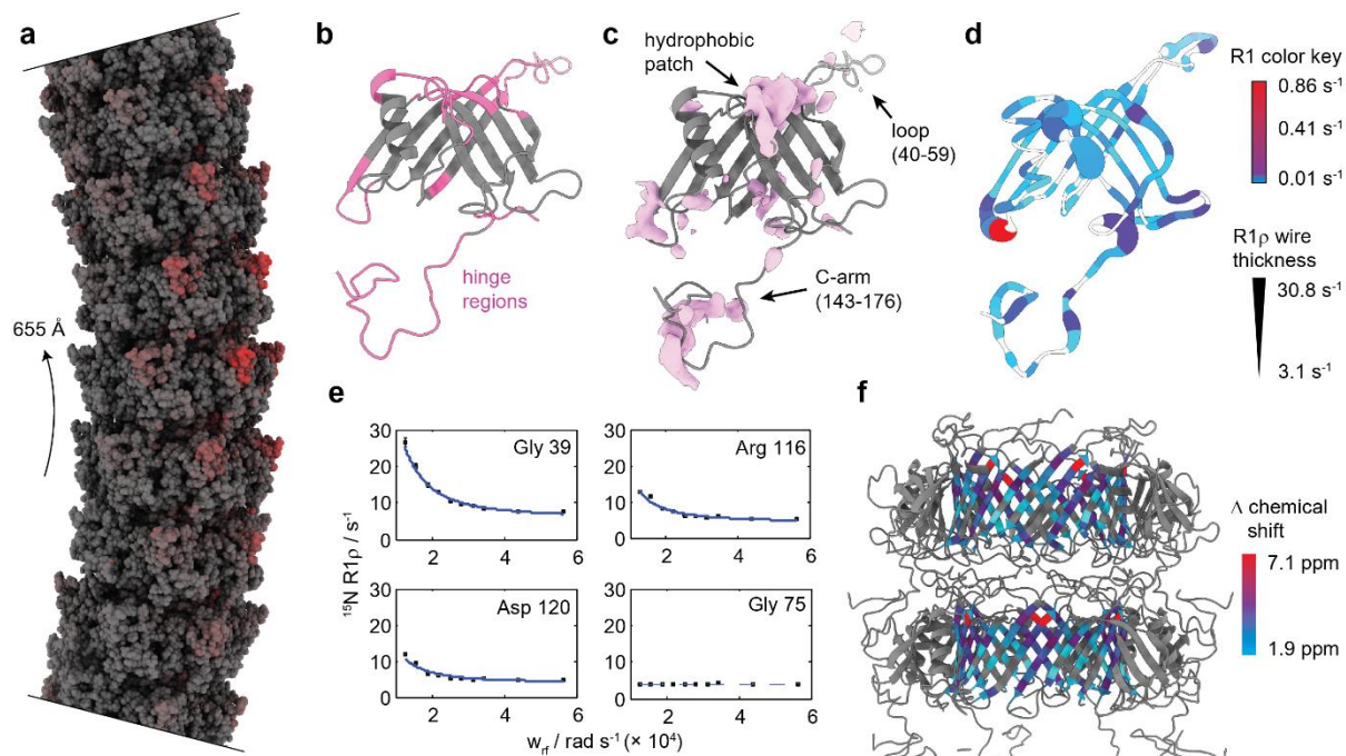
Fig. 4. Bending of the tail tube is mediated by flexible hinge regions. a , Model of a bent SPP1 tail tube with a curvature radius of 655 Å. The model is based on the structure of straight tubes and 2D class averages of bent tubes. Most structural changes are found on the outside of the curve (red) which implies that the bending process is mediated by stretching. b , Regions that act as hinges during bending of the tube are colored in pink. c , Variances in the cryo-EM map (pink) match the hinge regions. d , Also, hinge regions are associated with highest ^{15}\text{N} R_1 (color key) and R_{1\rho} (thickness of wire) relaxation rates. White coloring represents missing values. e , Decaying relaxation dispersion profiles indicate the presence of slow motions. f , Relaxation dispersion profiles of the inner \beta -barrel can be fitted in a correlated manner to a two-state exchange process. Smallest chemical shift changes correlate with middle regions of the \beta -barrel which are furthest away from the hinge regions (color key).
