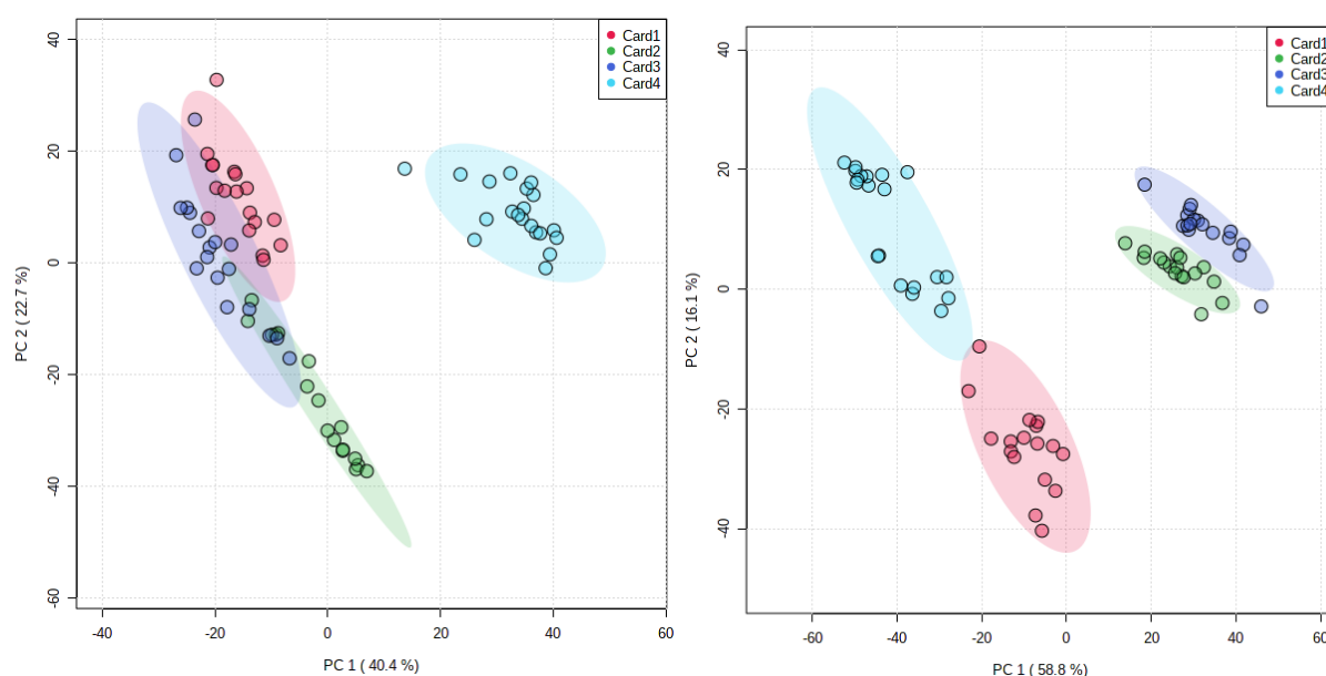
Fig. 2. Principal component analysis of dried blood spots prepared from fresh blood from three healthy volunteers (Cards 1-3) and synthetic human blood (Card4). Panel A, positive ionisation mode ( n = 203 variables); B, negative ionisation mode ( n = 316 variables). Only variables that have 75% or more non-zero values were used. n = 20 measurements per group.
