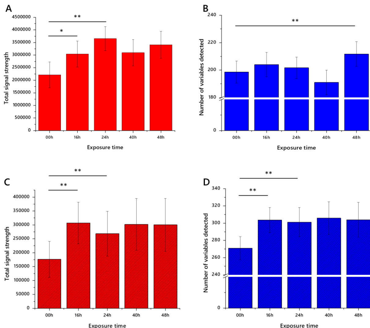
Fig. 1. Signal strength and number of variables identified in lipid extracts of dried blood spots exposed to a guanidine-thiourea buffer. Panel A, total signal strength of QCed variables; B, number of QCed variables. Error bars show standard deviation. n = 16 measurements per group. * p < 0.01 , ** p < 0.001 . The control (00h) time point represents the present method used (no chaetropes, exposure to water shortly before exposure to organic solvents).
