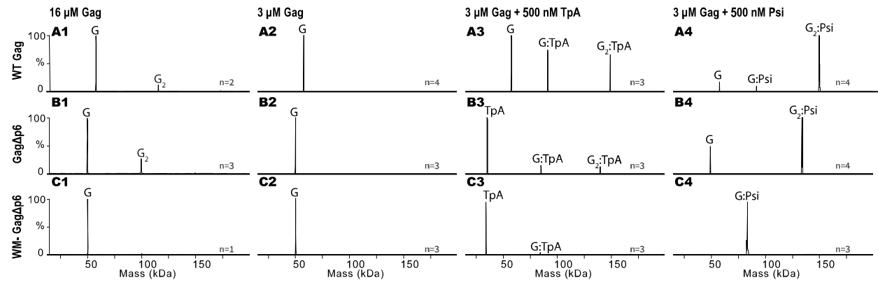
Figure 2. Zero-charge mass spectra of: WT Gag (A1), GagΔp6 (B1) and WM-GagΔp6 (C1) at 16 μM; WT Gag (A2), GagΔp6 (B2) and WM-GagΔp6 (C2) at 3 μM; 500 nM TARpolyA in the presence of 3 μM WT Gag (A3), GagΔp6 (B3) and WM-GagΔp6 (C3); 500 nM Psi in the presence of 3 μM WT Gag (A4), GagΔp6 (B4) and WM-GagΔp6 (C4). Notation is as follows: G=Gag, G 2 =two Gag, TpA=TARpolyA. Molecular masses for all analytes are listed in Table S1. The number of replicates (n) per experiment are indicated on each spectrum with additional repeats shown in Supplemental Figures S1-S6.
