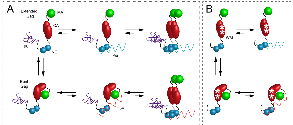
Figure 6. Model for WT (A) and mutant (B) WM-GagΔp6 binding to Psi RNA (top) and non-Psi RNA (bottom). In the absence of RNA, WT Gag is a monomer in equilibrium between bent and extended conformations. Gag binds Psi in a dimerization-competent extended conformation and dimerizes. Gag binds TpA in the dimerization-incompetent bent conformation and must undergo a rate-limiting extension before dimerization occurs.
