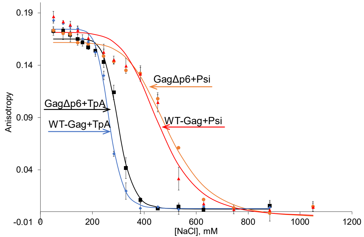
Figure 3. Fluorescence anisotropy results for WT Gag and GagΔp6 binding to Psi and TARPolyA RNAs as a function of NaCl concentration (n=3, error bars reflect the standard deviation of three independent measurements).
