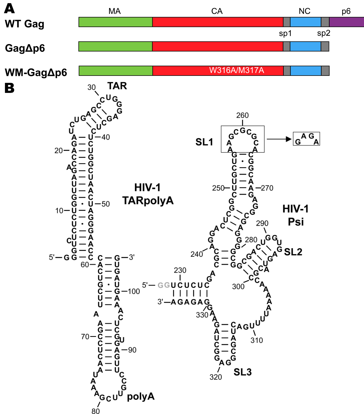
Figure 1. (A) Domain structure of WT and mutant Gag proteins investigated in this work. (B) Sequence and predicted secondary structures of TARpolyA ( left ) and Psi ( right ) RNAs. To ensure a monomeric state, the SL1 loop of Psi was mutated to a GAGA tetraloop as indicated. The gray nucleotides at the 5' end of Psi (GG) are not encoded by HIV-1 but were added to improve the yield of in vitro transcription.
