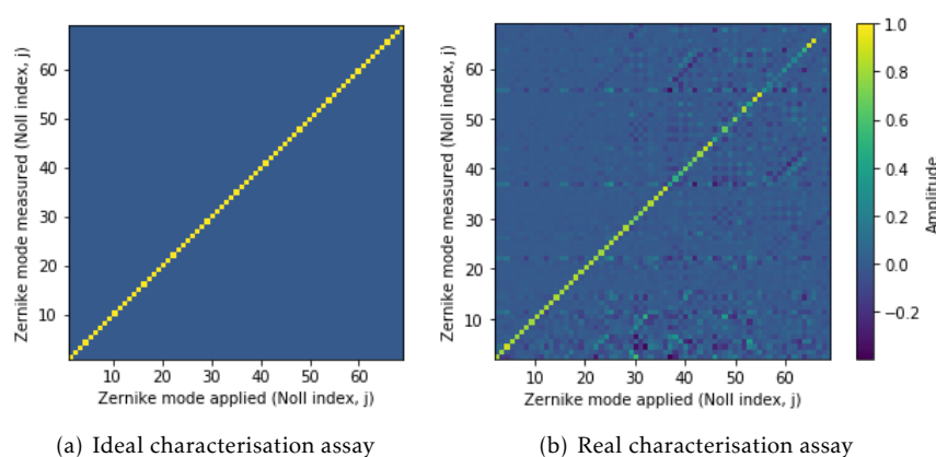
Figure 4: (a) An ideal characterisation assay, measuring the recreation accuracy of 68 Zernike modes with applied amplitude of 1 for each (b) A realistic characterisation assay obtained from a calibrated Alpao-69 actuator deformable mirror, measuring the recreation accuracy of 68 Zernike modes with applied amplitude of 1 for each
