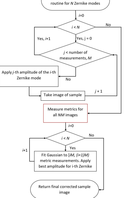
Figure 8: Flowcharts depicting the sensorless correction routine options (a) An image for each amplitude of the i -th Zernike mode is taken and the image quality metric is immediately evaluated. Once all the images for the i -th Zernike mode have been taken, the best Zernike amplitude is found as described in Figure 7 and applied (b) All M images are taken, then the quality metric is obtained for all M images, the best Zernike amplitude is found and applied (c) All the images for all the N Zernike modes are obtained with no correction applied in between modes. The image quality metric then measured for every image and the best amplitude for each Zernike mode is found. The correction for all modes is applied simultaneously at the end of the workflow.
