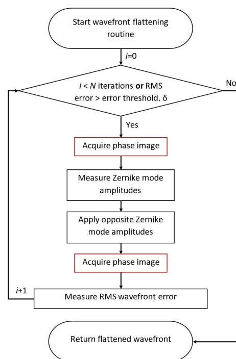
Figure 5: Flowchart depicting the process for flattening directly measured wavefront as implemented in Microscope-AOtools
