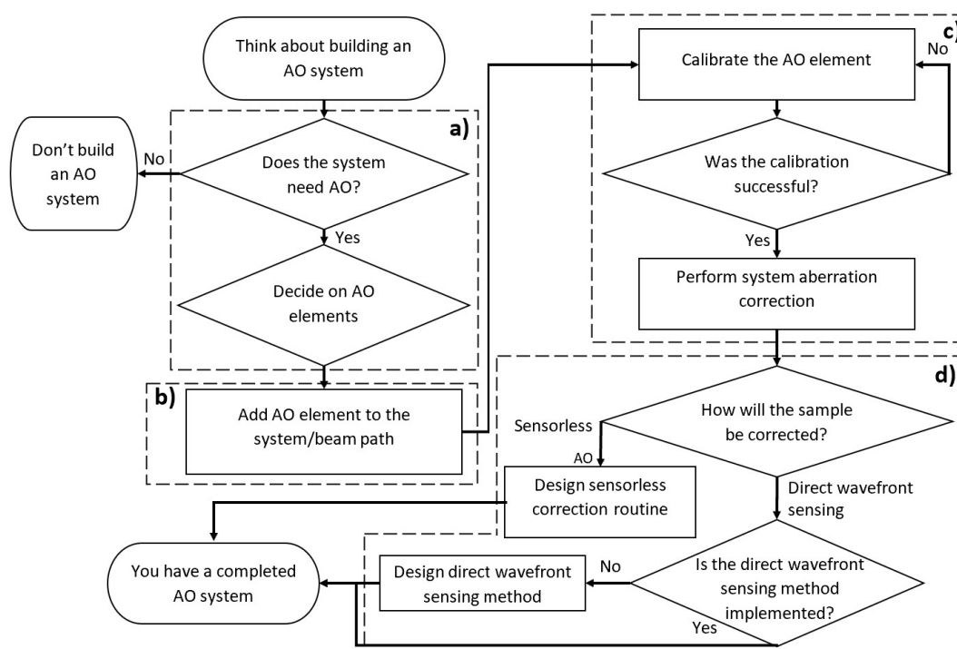
Figure 1: Flowchart depicting the general process for building a system utilising AO. a) System Design Phase. User decides whether the system needs AO and, if so, what type. b) Installation Phase. The chosen AO elements are added to the system. c) Set-up Phase. The chosen AO element is calibrated. Typically this involves mapping the variable elements of the AO element (e.g. deformable mirror actuators) to a useful set of basis functions which represent optical aberrations. d) Sample Correction Phase Here the user designs the methods to be used for correcting their desired sample.
