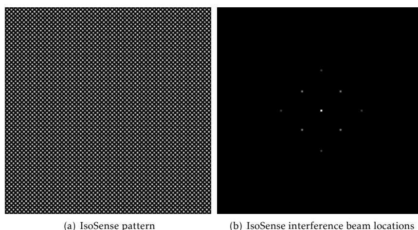
Figure 9: (a) A simulated IsoSense pattern created with a 4-beam interference. A pattern similar to this is applied to the SLM (b) A diagram of a 4 beam interference pattern in Fourier space.
