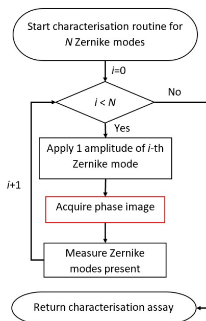
Figure 3: Flowchart depicting the process for characterising an adaptive element as implemented in Microscope-AOtools
