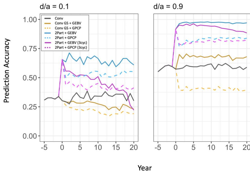
Figure 7 Prediction accuracy for the total genetic value of the seedlings under different dominance degrees (d/a). In each panel, prediction accuracy is plotted in the seedling stage for the entire burn-in breeding phase and the future breeding phase. Each line shows the mean prediction accuracy for the 10 simulated replications. The different types of breeding program are shown in different colours. The conventional breeding program (Conv) is gray. The conventional breeding program with genomic selection (Conv GS) is yellow. The two-part breeding program with genomic selection (2Part) is shown in blue with one crossing cycle per year and in purple with three crossing cycles per year. The two types of parent selection were shown in different line-styles. Selection based on Genomic Estimated Breeding Value (GEBV) is shown by continuous lines. Selection based on Genomic Prediction of Cross Performance (GPCP) is shown by dashed lines.
