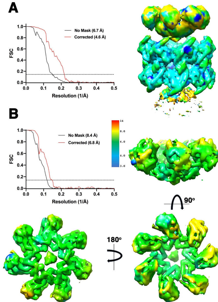
Figure S1. Resolution of Rep68-ssDNA DOC.
