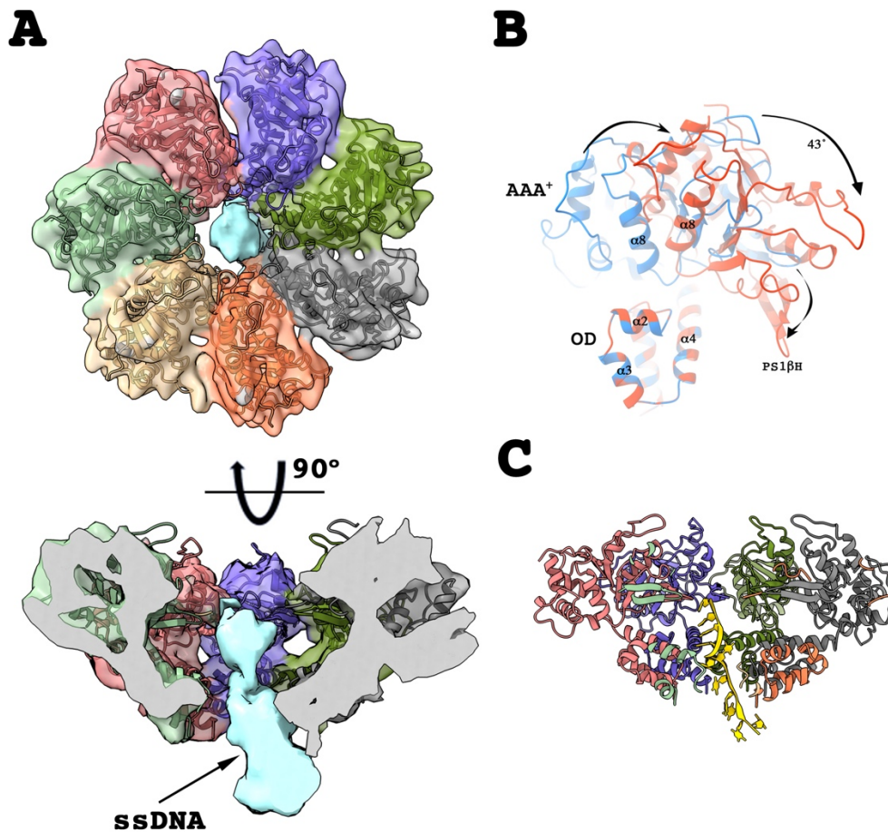
Figure 6. Effect of ATP \gamma S on DOC complex.
