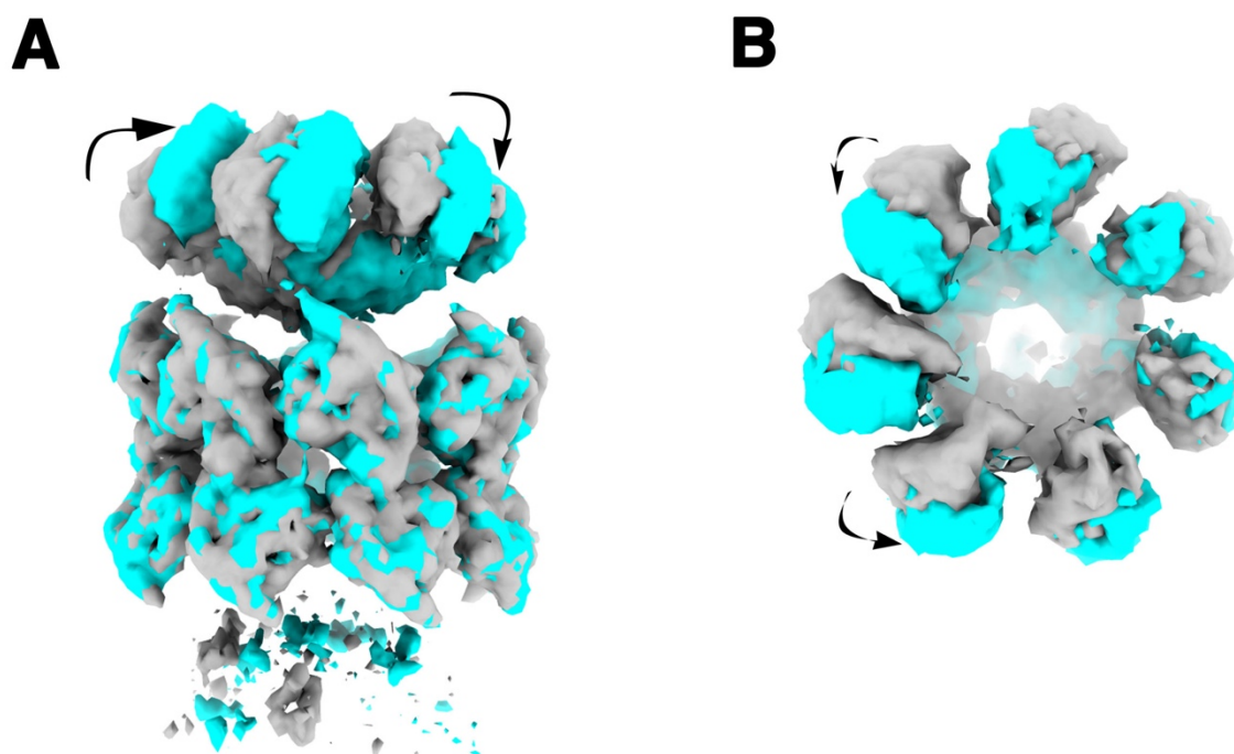
Figure S4. 3D variability analysis of DOC.
