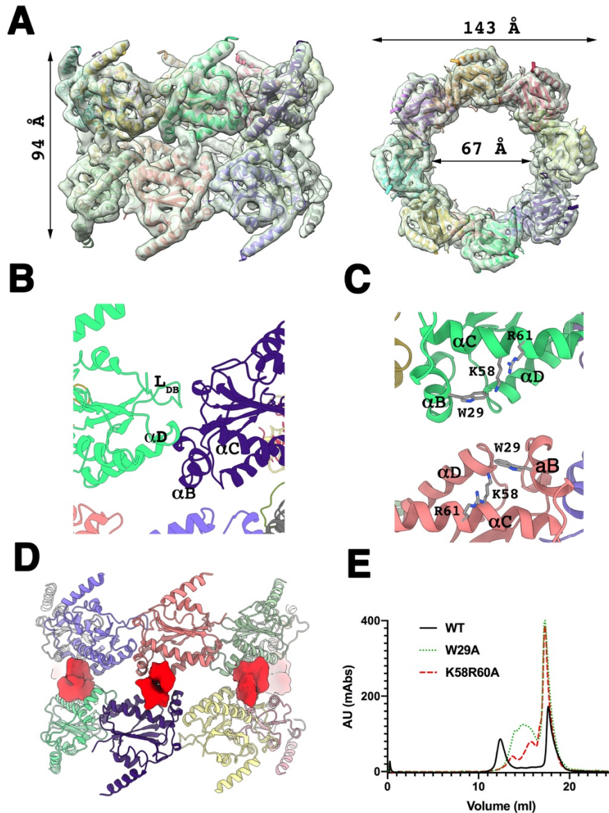
Figure 2. Structure of OBD Double-octamer.
