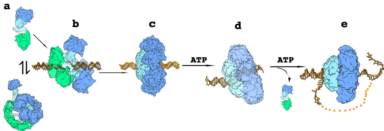
Figure 9. Model for assembly and DNA melting on dsDNA by AAV Re proteins.
