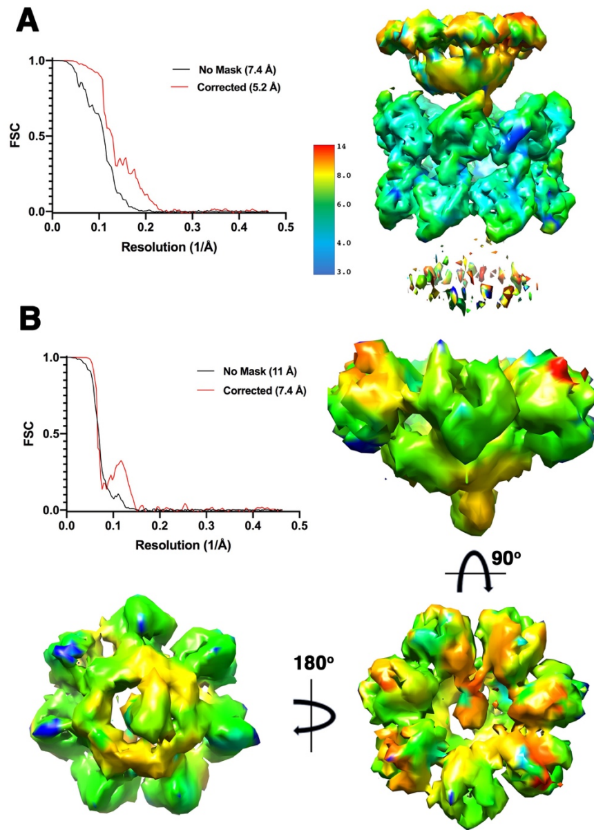
Figure S5. Resolution of Rep68-ssDNA-ATP \gamma S DOC.
