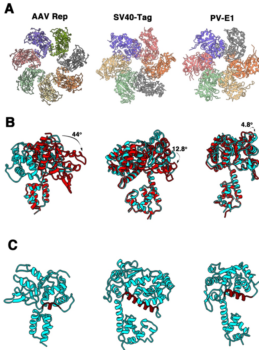
Figure S8. Comparison SF3 Helicases.
