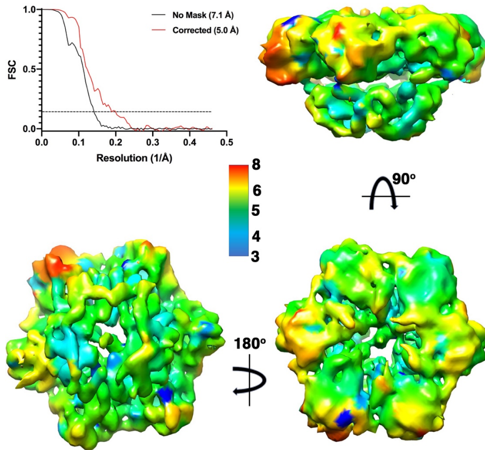
Figure S7. Resolution of Rep68-ssAAVS1-ATP \gamma S hexameric complex.
