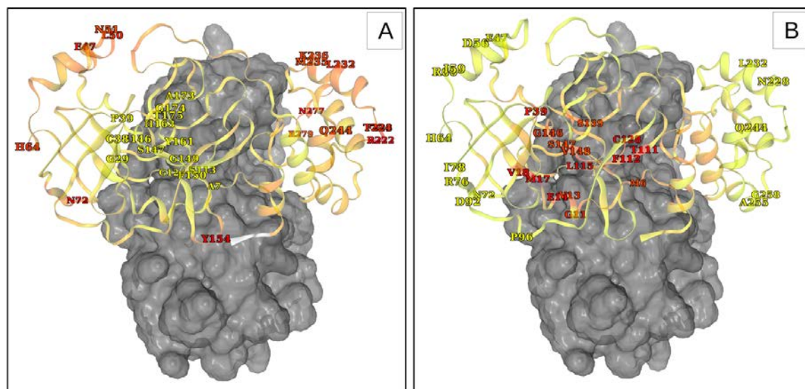
Fig. 5. 3D mapping of averaged values for (A) RMSF and (B) the average BC, computed across all M^{pro} samples. Only the extremes (top and bottom 5% of the ECD values across all samples) of averaged values are labelled for each metric. The lowest averaged values are in yellow while the highest ones are in red. The last three C-terminus residues (in white) were not mapped by RMSF as their high values would mask other values. While only one protomer is detailed, the data is applicable to both protomers. The other protomer is represented as a grey surface.
