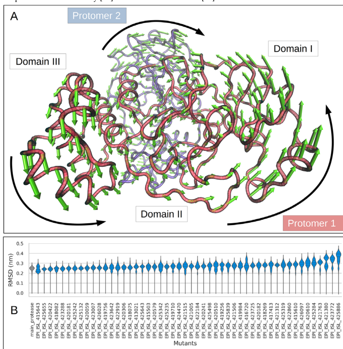
Fig. 3. (A) The general twisting motion of the protomers observed across M pro samples, inferred from the reference protease using ANM. (B) Violin plots of C α RMSD values for the reference (in grey) and the mutant (coloured in blue) M pro , showing the 25 th , 50 th and 75 th percentiles in dotted lines inside the kernel density plots. Distributions are scaled by counts, and have been sorted by median RMSD for the mutants.
