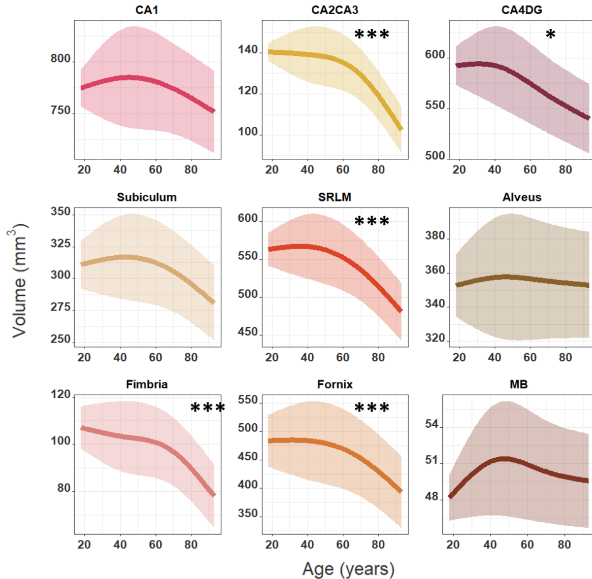
Supplementary figure 7: Best fit models showing the relationships between age and the volume of the left hippocampal subfields. Best fit models displayed for each subfield covaried by ICV and sex as fixed effects and dataset, sequence, and subject as random effects. Significant monotonic decreases were found for the left CA2CA3 ( p=4.5 \times 10^{-6} ), CA4DG ( p=0.012 ), SRLM ( p=3.60 \times 10^{-6} ), fimbria ( p=6.16 \times 10^{-7} ) and fornix ( p=2.20 \times 10^{-5} ). * p < 0.05 ; ** p < 0.01 and *** p < 0.001 after Bonferroni correction.
