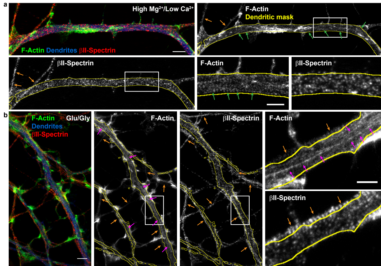
Figure 3: Two-color STED nanoscopy of F-actin and \beta\text{II} -spectrin in dendrites. (a) Low-activity high \text{Mg}^{2+} /low \text{Ca}^{2+} condition and (b) Glutamate/Glycine neuronal stimulation. (a) Top-Left and (b) Left : Overlay of two-color STED nanoscopy of F-actin (green) and \beta\text{II} -spectrin (red) with confocal imaging of MAP2 (blue) to identify the dendrites. Insets show the magnified regions identified in the full single-color STED images of F-actin and \beta\text{II} -spectrin. Arrows indicate the detected F-actin and \beta\text{II} -spectrin patterns: dendritic rings (green), axonal rings (orange), and longitudinal fibers (magenta). Scale bars (a, b) 2 \mu\text{m} , insets 1 \mu\text{m} .
