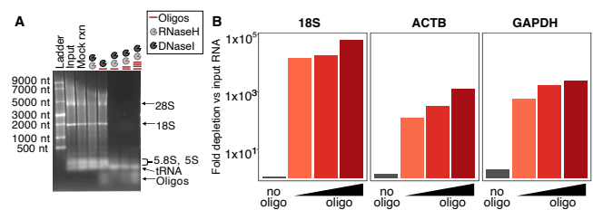
Fig. 2. RNaseH-mediated rRNA and non-specific mRNA depletion. A) Non-denaturing 1.2% agarose gel depicting the following lanes from left to right: 1) ssRNA ladder; 2) total RNA input; 3) input with mock incubations; 4) RNaseH treatment and DNaseI treatment without oligos; 5) DNaseI and oligos only; and 6-8) increasing oligo:RNA mass ratio (1:1, 2:1, and 4:1; total RNA fixed at 1 µg) with RNaseH and DNaseI treatment. B) Fold depletion of 18S rRNA, ACTB, and GAPDH transcripts normalized to input total RNA by RT-qPCR performed on the RNA samples in panel A. Total RNA samples incubated with RNaseH and DNaseI without oligos (grey bar) or increasing oligo:RNA ratio (red bars) with RNaseH and DNaseI treatment. NEB E.coli RNaseH treatment for 1 hour at 37°C and NEB E.coli DNaseI treatment for 30 minutes at 37°C used for samples in this experiment.
