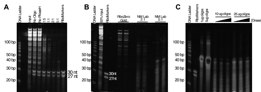
Fig. S2. RNaseH-mediated rRNA depletion for Ribo-Seq. All samples were run on a 15% Denaturing PAGE gel. 30nt and 27nt RNA markers were spiked into input material. A) 1μg ribosome footprinting input material at various ratios of oligo:RNA concentration. B) 5μg ribosome footprinting input material depleted of rRNA using Illumina RiboZero Gold or NM Lab's method at 2:1 and 5:1 oligo:RNA concentration. C) 10μg or 25μg rRNA depletion oligos treated with increasing concentration of TurboDNase (5, 15, and 30U).
