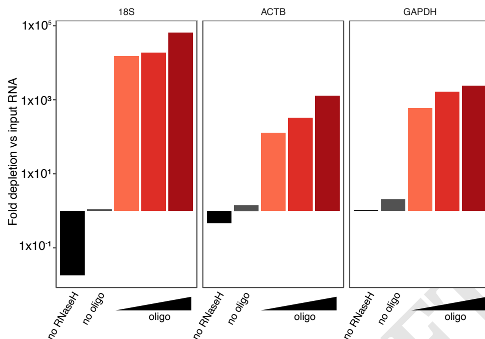
Fig. S1. Control without RNaseH enzyme shows increase by qPCR likely due to priming of leftover DNA oligos. Fold depletion of 18S rRNA, ACTB, and GAPDH transcripts normalized to input total RNA by RT-qPCR performed on the RNA samples in Figure 2A. Total RNA samples incubated with oligos and DNase but without RNaseH (black bar), RNaseH and DNaseI without oligos (grey bar), or increasing oligo:RNA ratio with RNaseH and DNaseI treatment. NEB E.coli RNaseH treatment for 1 hour at 37°C and NEB E.coli DNaseI treatment for 30 minutes at 37°C used for samples in this experiment.
