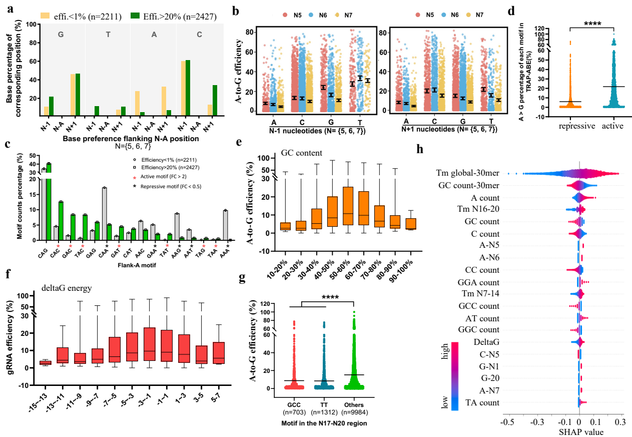
Figure 4 Characterization of nucleotide features affecting ABE efficiency
