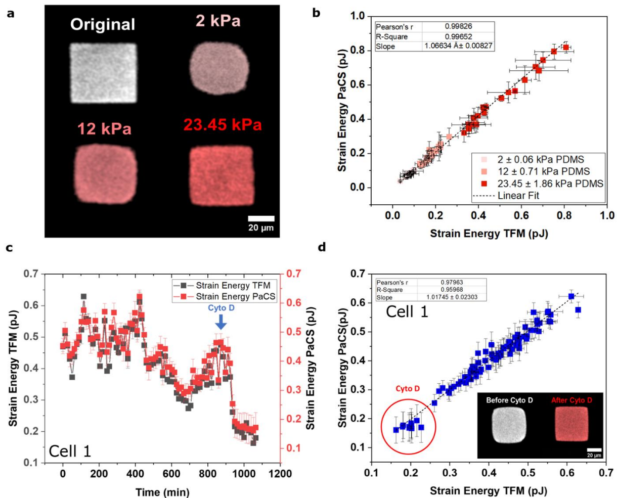
Figure 3: PaCS resolves time dependent contractile work and cytoskeletal activity as a function of substrate stiffness. a , Pattern deformations by 3T3 fibroblast cells on PDMS substrates of different Young's moduli (2, 12 and 23.45 kPa) b , Total strain energy calculated with pattern deformations strongly correlates with strain energy calculated with TFM (n=60). c , Time-dependent relation between strain energy calculated with PaCS and TFM (cell 1), blue arrow represents the time of addition of Cyto D (Time interval 12.83mins) (n=84 timepoints). d , Strain energy calculated with pattern deformations with time strongly correlates with strain energy calculated with TFM, red circle represents the strain energy values after Cyto D (n=84 timepoints).
