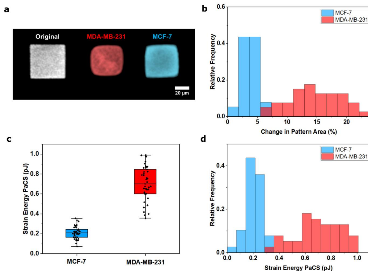
Figure 4: PaCS reveals contractile differences between low metastatic and highly metastatic breast cancer cells.
