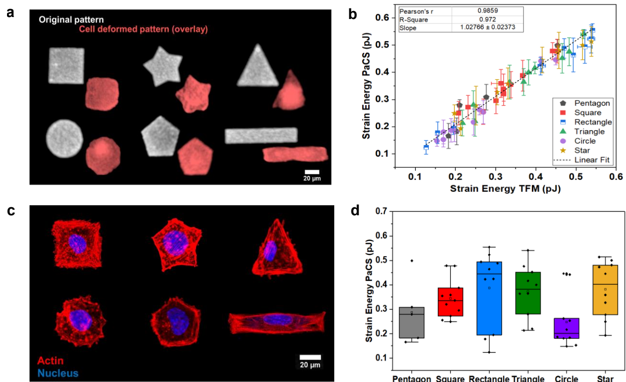
Figure 2: PaCS accurately measures cell contractile work across diverse cell shapes: a , Fluorescent BSA-fibronectin patterns of various shapes deformed by 3T3 Fibroblast cells on 12 kPa PDMS substrates. b , Total strain energy calculated with PaCS strongly correlates with strain energy calculated with TFM ( n=56 ). c , 3T3 Fibroblast cells fixed and stained with phalloidin (actin) and DAPI (nuclei), imaged on Leica SP8 confocal (63X/1.4NA objective). d , PaCS strain energy for 3T3 Fibroblast cells indicate cells confined in circular shape to apply the least strain energy.
