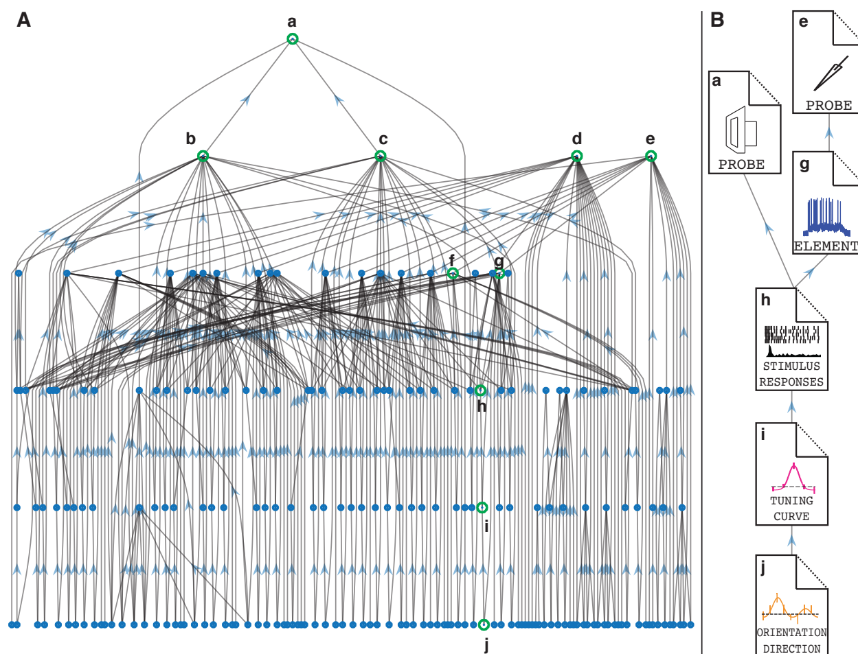
Figure 11. Graph structure of the database documents of an example experiment in NDI. A) Full graph of documents from an experimental session from Roy et al. (2020). Documents are denoted by nodes (blue or green circles), and arrows point from dependent documents to the documents that they depend upon. In this graph, a is a visual stimulus monitor probe, and b and c are stimulus presentation documents that describe the presentation of sinusoidal gratings in different directions. d and e are sharp electrode probes corresponding to 2 recordings of different impled cells. f and g are documents describing the ndi_element objects of probe e where spikes are removed ( f ) and where spike times are extracted ( g ). h is a document containing the stimulus responses of the spikes in g to the stimulus presentation in c . In i , these stimulus responses have been collated into a tuning curve. Finally, these responses have been examined to extract orientation and direction index values and to perform a double Gaussian fit, which are all stored in document j . B) Zoomed in view of the document pipeline a-j .
