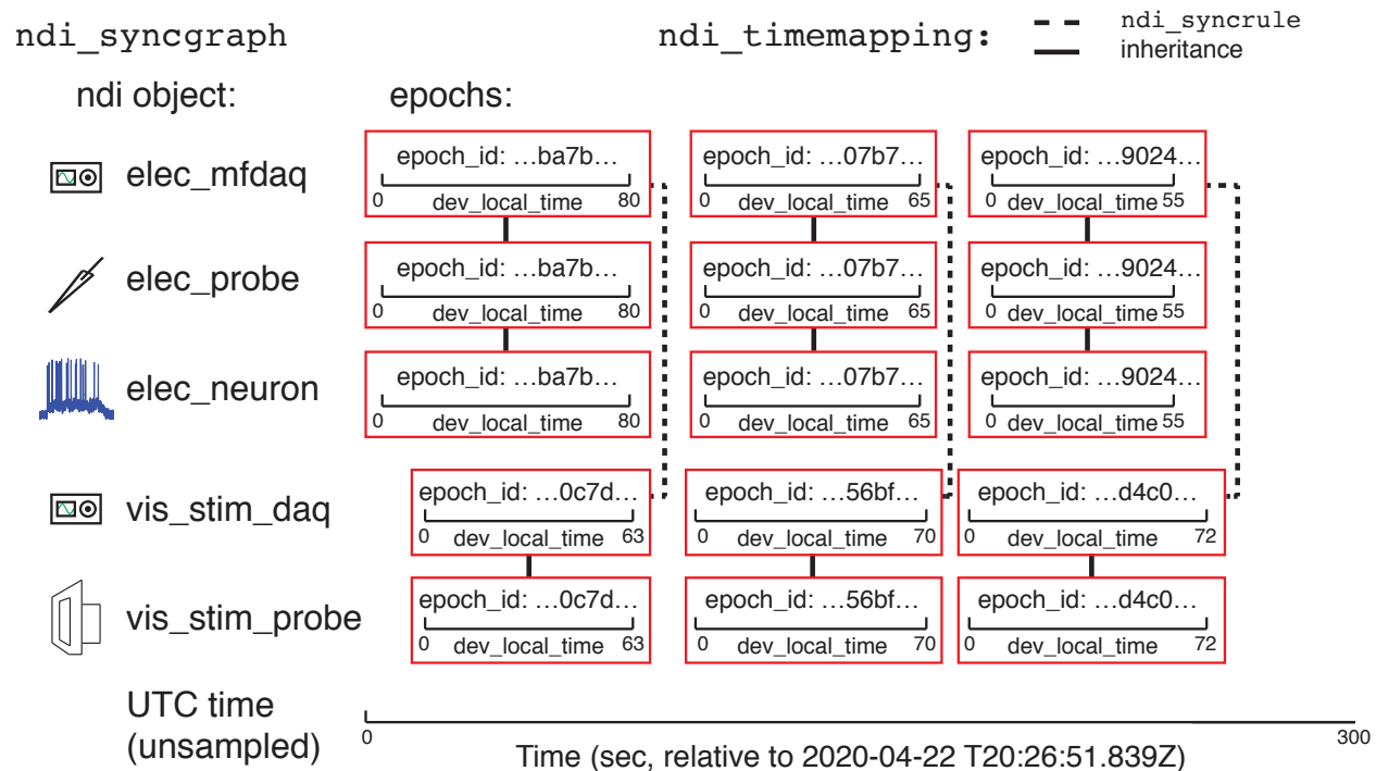
Figure 6. Epochs and ndi_syncgraph. Illustration of an example experiment with 2 ndi_daqsystm objects ( elec_mfdaq and vis_stim_daq ) that are each connected to a probe ( elec_probe and vis_stim_probe , respectively). The DAQ systems have their own clocks that are not linked to any global time system. 3 epochs have been recorded by each DAQ system. The electrode probe has been analyzed and an ndi_element object (a neuron, elec_neuron ) has been created from it. The clock and time of each of the epochs for the neuron is inherited from its underlying probe, which is in turn inherited from the underlying DAQ system. The 2 DAQ systems each record the same set of digital triggers, and ndi_syncgraph has used its list of ndi_syncrule objects to compute a mapping ( ndi_timemapping ) between epochs of those DAQ systems. Time can be converted between epochs that are recorded simultaneously on the 2 DAQ systems, but we do not know how the other epochs are related to each other, or how any epoch is related to a global time system like universal controlled time (UTC), shown below.
