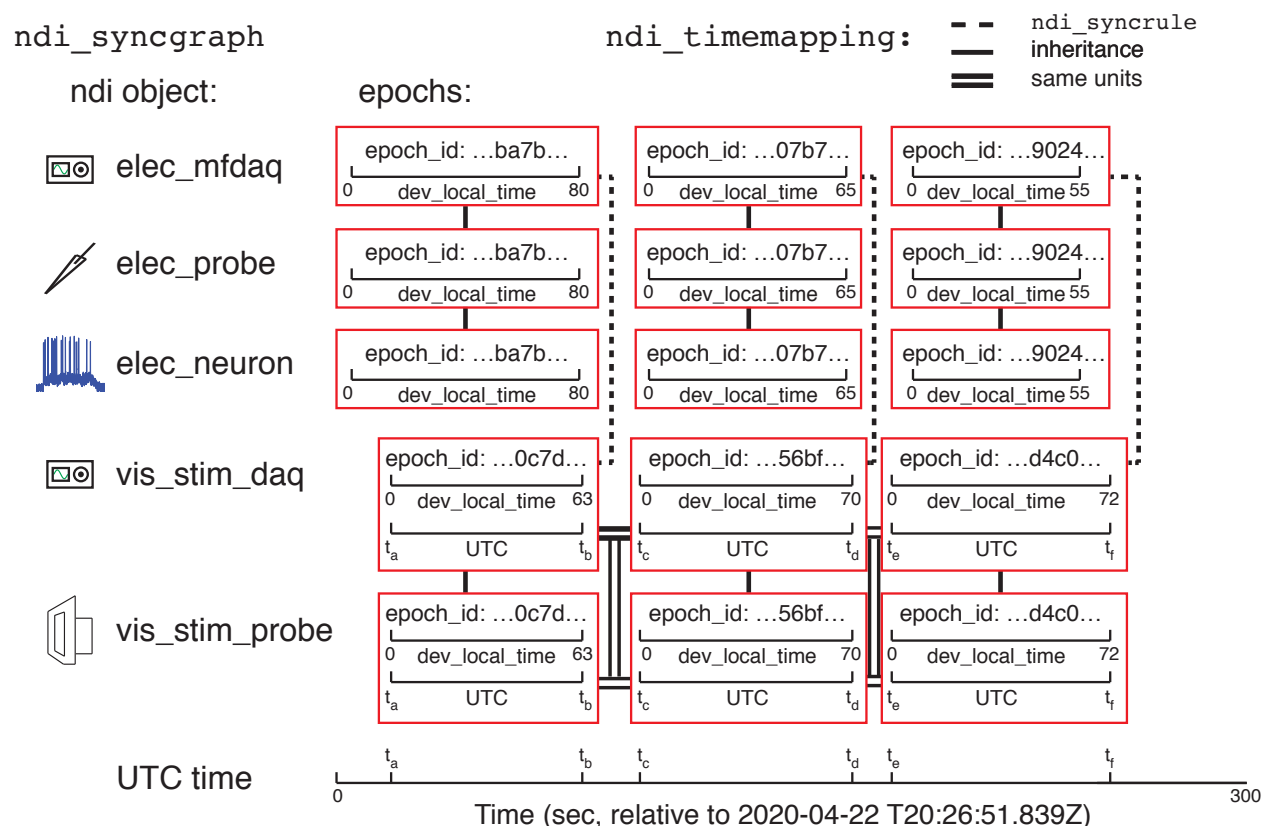
Figure 7. Epochs and ndi_syncgraph. Illustration of an example experiment similar to that in Figure 6, except that the vis_stim_daq DAQ system also keeps UTC time in addition to its own local clock. Here, time can be converted among any epoch because there is a mapping between the epochs of vis_stim_daq and UTC, and there are ndi_timemapping mappings between the DAQ system. The time in any epoch can be computed according to the clock of any other epoch, by solving the transformations in the syncgraph. The mappings shown are ndi_timemapping objects built by a) an ndi_syncrule, b) inheritance (e.g., a probe inherits the epoch information of the DAQ system that acquired it); and c) same units (UTC is a global time system).
