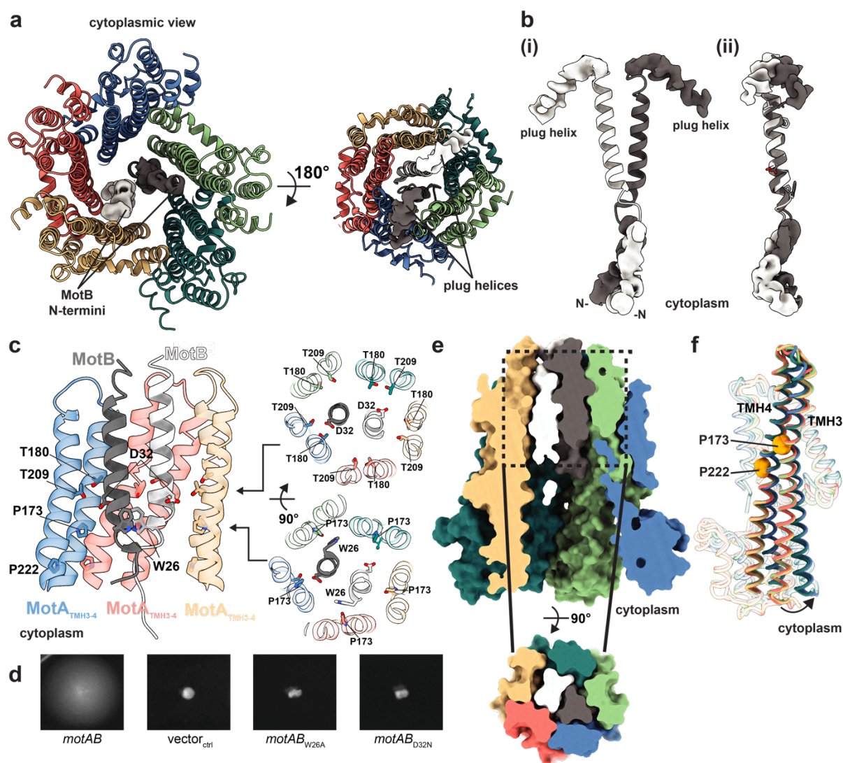
Figure 3. Functionally critical regions of the stator complex. a , Structure of the C. sporogenes stator shown as cartoon representations coloured as in Figs. 1 and 2 with the unmodeled density for the MotB N-terminal extensions (Left) and plug helices (Right) shown. b , (i) Isolated MotB dimer extracted from the C. sporogenes stator and (ii) superposition of the TMHs of the two MotB chains showing the relative rotation of the N-terminal extensions and plug helices. c , The environment around MotB D32 within the membrane. (Left) Only the core MotA helices within the transmembrane region are shown and the two copies of MotA at the front of the view are removed. (Right) Slabs through the stator core at the indicated heights. Residue numbering is that of the E. coli MotAB stator but displayed on the C. sporogenes stator structure. d , Motility in soft agar of E. coli RP6894 ( \Delta motAB ) complemented with plasmids expressing motAB with the indicated mutations or the vector control (vector ctrl ). e , Surface representation of the model shows close packing. (Top) Side view with front of complex removed. (Bottom) Top-down view of the slab indicated by dashed lines. f , Overlay of the five copies of the C. sporogenes MotA chain reveals they fall into two conformational classes which differ in the degree of flexing at the highlighted prolines.
