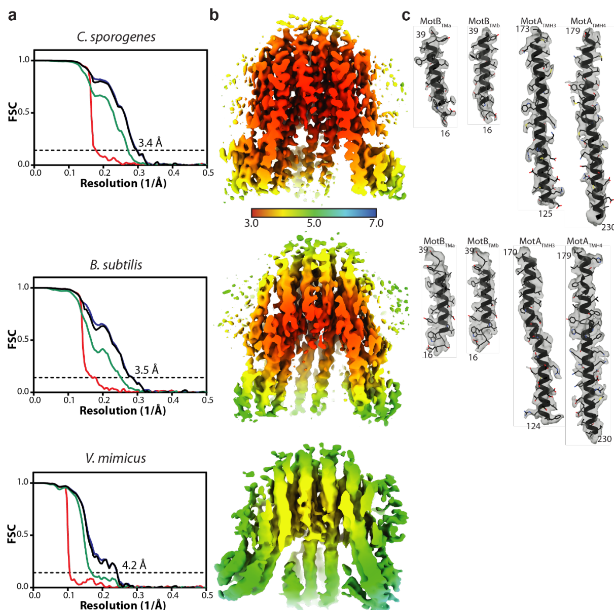
Extended Data Fig. 2. Cryo-EM map quality and resolution estimates of stators. a , Gold-standard Fourier shell correlation (FSC) curves of RELION-postprocessed stator volumes. Resolution at the gold-standard cutoff (FSC = 0.143) is indicated. Curves: red, phase-randomized; green, unmasked; blue, masked; black, MTF-corrected. b , Local resolution estimates (in Å) of the sharpened volumes. c , Representative modelled densities.
