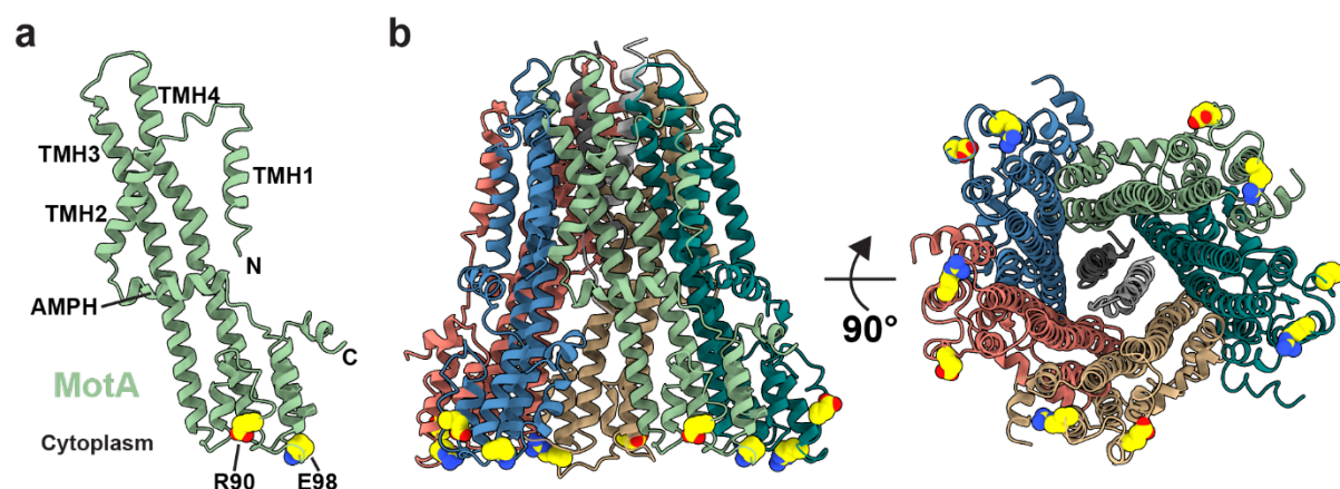
Extended Data Fig. 4. Residues that interact with the flagellar C-ring form a charged ring on the cytoplasmic face of MotA. a , An isolated MotA subunit with the essential torque-generating charged residues R90 and E98 24 displayed in yellow spheres representation. b , The full C. sporogenes stator complex viewed from the side (Left) or from the cytoplasm (Right), coloured as in Figs. 2-3, and with the torque-generating charged residues represented as in (a) using E. coli MotAB numbering scheme.
