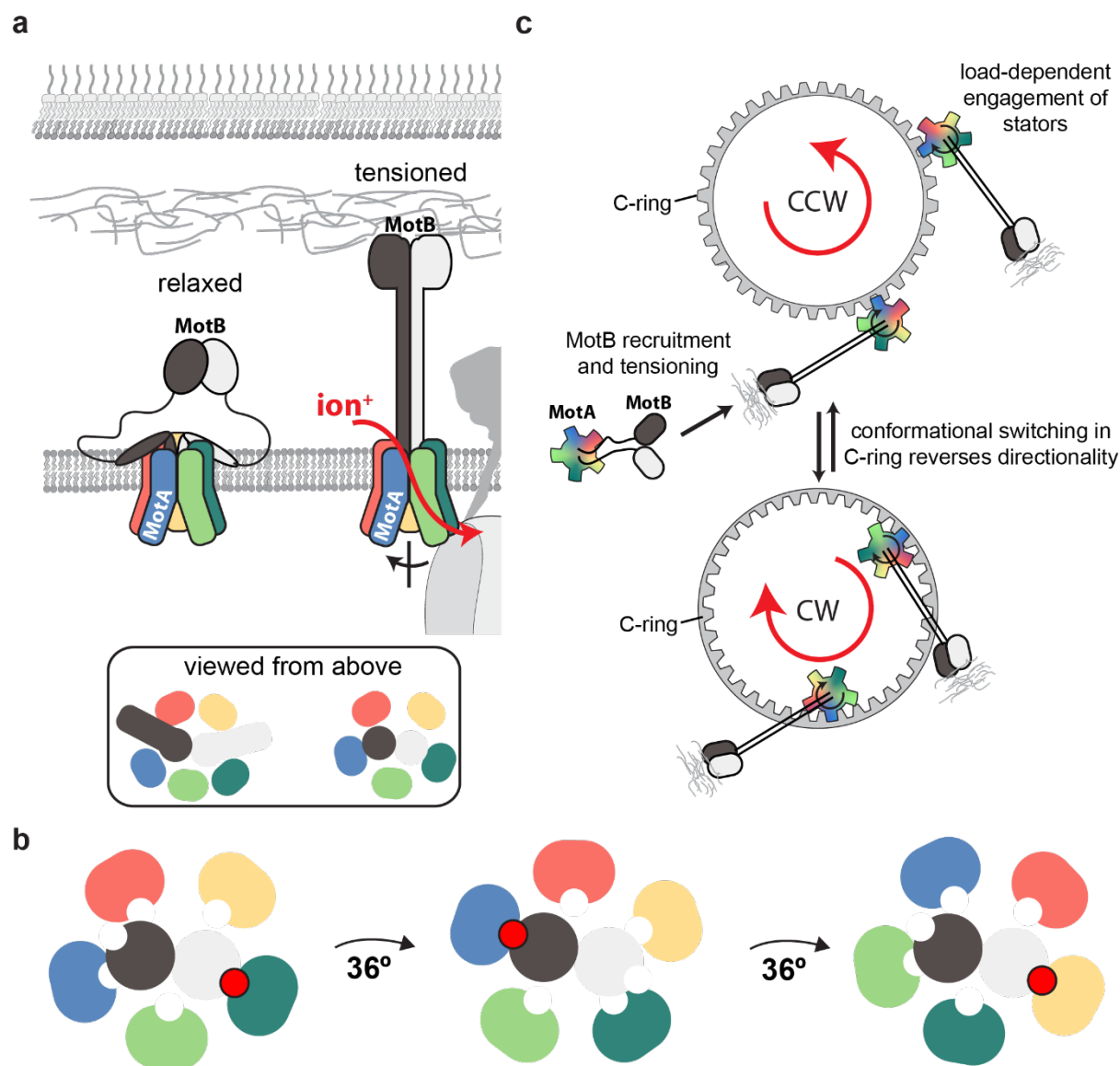
Figure 4. Mechanistic model for the generation of bi-directional flagellar torque. a , Activation of the stator complex from the structurally resolved state (here termed ‘relaxed’) to form a ‘tensioned’ state permissive to ion-flow. This conformational change is likely driven by interactions between the C-terminal peptidoglycan binding domains (black and white ovals) of MotB and the peptidoglycan layer, as well as interactions between the stator and the C-ring complex. b , Cartoon showing top views of the intra-membrane core of the stator complex with five MotA chains surrounding two MotB subunits. Bound ions are shown as red spheres. Ion flow leads to rotation of the MotA ring through alternating formation of MotB-ion-MotA interactions by the two MotB chains that processes around the surrounding MotA subunits. c , Model describing how a stator that rotates in one direction can drive either clockwise (CW) or counterclockwise (CCW) rotation of the flagellum depending on the conformational state of the C-ring.
