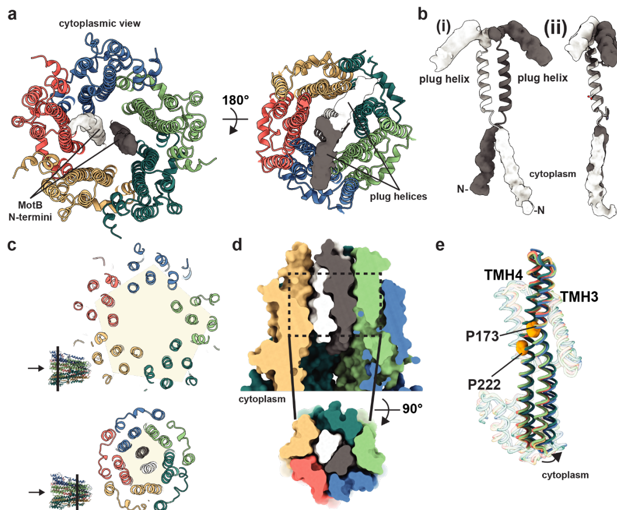
Extended Data Fig. 5. Structural elements of the B. subtilis stator. a , Structure of the B. subtilis stator depicting unmodeled density for the MotB N-terminal extensions (Left) and plug helices (Right). b , (i) Isolated B. subtilis MotB dimer represented as in (a), and (ii) superposition of the TMHs of the two MotB chains showing the relative rotation of the plug helices. c , Slabs at the heights indicated through B. subtilis MotAB show distortion from a regular pentagon (arrow indicates the cytoplasmic side of the complex) as viewed from the cytoplasm). d , Surface representation of B. subtilis MotAB showing tight packing. (Top) Side view with the front of the complex removed. (Bottom) Top-down view of the slab indicated by dashed lines. e , Structural alignment of the five B. subtilis MotA chains reveal they fall into two conformational classes which differ in the degree of flexing at the highlighted prolines.
