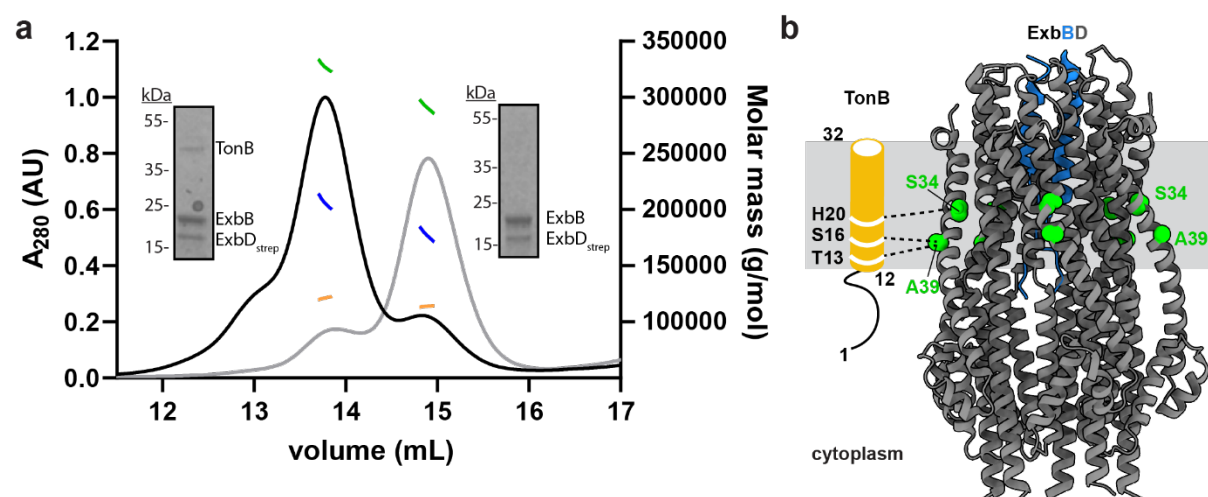
Extended Data Fig. 9. TonB recruitment to the ExbBD complex. a , SEC-MALS profile of purified Pseudomonas TonB-ExbBD (black absorption curve) and ExbBD (grey absorption curve) with SDS-PAGE analysis of each sample inlayed. Total protein-detergent complex molar mass (green) and deconvoluted protein (blue) and detergent (orange) molar masses are shown. A ~30 kDa difference in molar mass is observed between the complexes consistent with the the TonB-ExbBD complex containing one TonB subunit. b , Evolutionary co-variation of residues between TonB and ExbB displayed on the E. coli ExbBD structure 35 (PDB 6tyi). For clarity, a topological model of the TMH of TonB is shown in orange with TonB-ExbB contacts indicated as dashed lines. Covarying residues decorating the periphery of ExbB are displayed in green. ExbB (grey) and ExbD (blue) are displayed as ribbon cartoons. Contacts shown were generated by Gremlin 5 and have a probability score of > 0.9.
