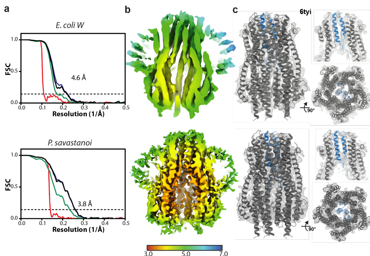
Extended Data Fig. 7. Cryo-EM map quality and resolution estimates of ExbBD complexes a, Gold-standard Fourier shell correlation (FSC) curves of RELION-postprocessed ExbBD maps. Resolution at the gold-standard cutoff (FSC = 0.143) is indicated. Curves: red, phase-randomized; green, unmasked; blue, masked; black, MTF-corrected. b, Local resolution estimates (in Å) of the sharpened maps. c, Structure of the 5:2 ExbBD complex from E. coli 35 (PDB 6tyi) fit into the E. coli W (top) and P. savastanoi ExbBD (bottom) maps. ExbB is coloured dark grey and ExbD is coloured blue. Top right panels have three ExbB subunits removed to demonstrate density for the two TMHs of ExbD. Bottom right panels reveal the 5:2 ExbB:ExbD arrangement as viewed from the cytoplasm.
