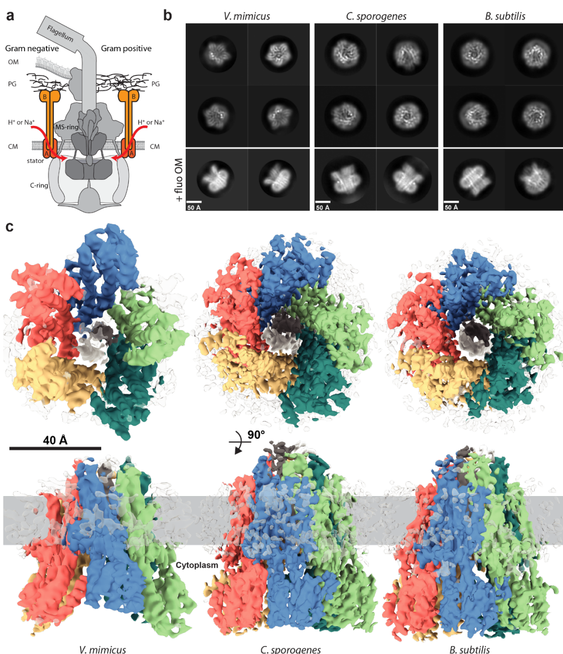
265 Figure 1. Stators from multiple organisms have a MotA 5 MotB 2 stoichiometry. a , Composite 266 cartoon showing the general organisation of bacterial flagellar complexes in Gram-negative 267 (left side) and Gram-positive (right side) bacteria with major components labelled. Stators are 268 orange and rotor components, MS- and C-ring, are grey. OM, outer membrane; CM, 269 cytoplasmic membrane; PG, peptidoglycan. b , 2D class averages of cryo-EM particles of 270 stators from the bacterial species indicated. Upper panels are representative ‘top’ views of 271 the 5:2 complexes. Lower panels are ‘side’ views from data collected in the presence of 272 fluorinated octyl maltoside. c , Cryo-EM volumes of stators from the three bacterial species. 273 The MotA subunits are coloured pink, blue, green, teal, and yellow, and the centrally-located 274 MotB subunits white and dark grey. Bound detergent is shown as transparent density at the
