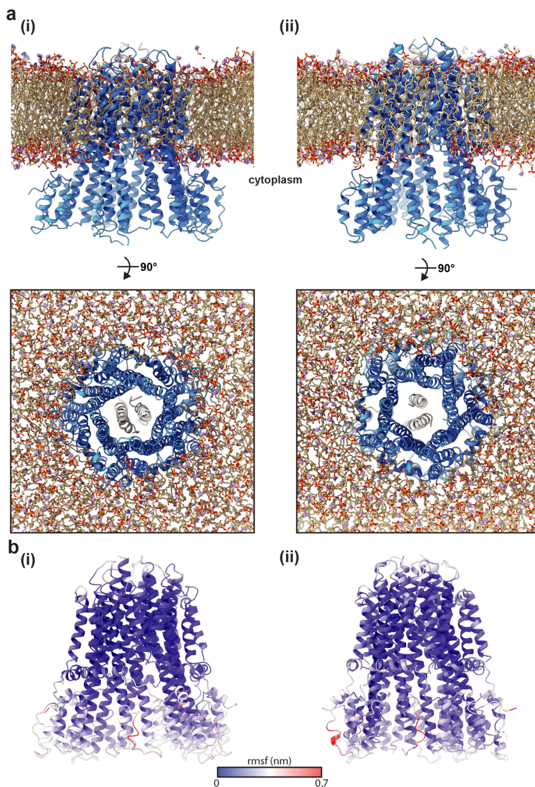
Extended Data Fig. 6. Molecular dynamics simulations of stator structures in lipid bilayers. a , Side ( top ) and top-down ( bottom ) views of (i) C. sporogenes and (ii) B. subtilis MotAB inserted within a lipid bilayer after extended simulations (coarsegrain for 1 \mu s then atomistic for a further 200 ns). b , Cartoon representation of (i) Clostridium MotAB and (ii) Bacillus MotAB coloured (blue to red) by the average rmsf of the 3 replica simulations performed.
