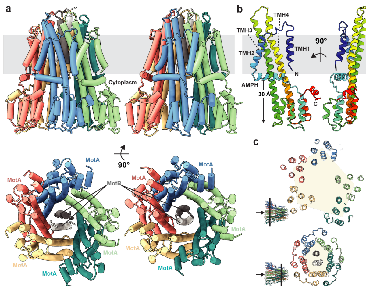
Figure 2. Structures of stators from C. sporogenes and B. subtilis . a , The C. sporogenes (left) and B. subtilis (right) stators are shown as cartoon representations and coloured as in Fig. 1c. Upper panel, side view with membrane indicated in grey. Lower panel, view from the cytoplasm. b , Two views of a single MotA subunit ( C. sporogenes ) coloured from blue at the N-terminus to red at the C-terminus. c , Slabs (viewed from cytoplasm) through the C. sporogenes complex at the indicated positions on the inset structure (arrow indicates the cytoplasmic side of the complex). Distortion of the MotA subunits from a regular pentagon arrangement becomes more extreme in the cytoplasmic regions.
