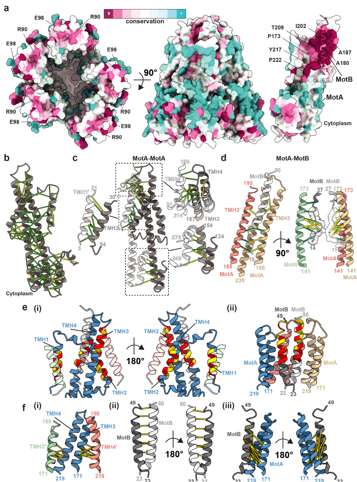
Extended Data Fig. 3. Conservation, covariance, and prior mutagenesis data mapped onto the stator structure. a , Surface conservation as determined by Consurf 48 (maroon high conservation, cyan low conservation). (Left) View from the cytoplasm showing conservation
