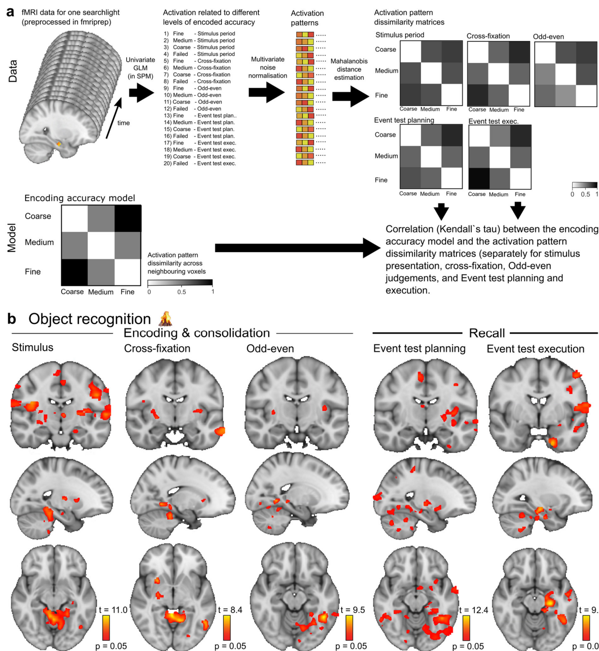
Figure S3. Representation of object identity. a , The activation from each searchlight in the brain was first analyzed voxel-wise using a univariate GLM, followed by multivariate noise normalization of the activation patterns related to different levels of encoded accuracy. Activation pattern dissimilarity matrices were then constructed by estimating the Mahalanobis distances between the activation patterns. Finally, the activation pattern dissimilarity matrices were correlated with a model representing consistent modulation of activation pattern dissimilarity with increasing level of encoded accuracy. b , Voxels in the brain that showed consistent modulation of activation pattern dissimilarity as object recognition representation became more accurate. Results are shown for the Stimulus period (left), Cross-fixation period (mid-left), Odd-even task (mid), and the Event test planning (mid-right) and Event test execution period (right). p = 0.05 represents the cluster mass corrected thresholds.
