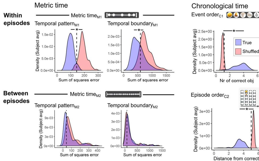
Figure 2. Metric time is only encoded within episodes. The “true” distribution of scores (blue) compared to the “shuffled” distribution of scores (red) (see also Table S1 and Methods). The distributions were based on the average score from each participant. Metric time reflects the degree to which the participant’s response displays the accurate timing between all the events or episodes (temporal pattern) and the accurate timing between the events or episodes and the temporal boundaries (temporal boundary) (see Figure 1 and Figure S1). Recall accuracy of metric time and chronological time were assessed both within episodes (top row) and between episodes (bottom row). The chance level (dotted line) was defined as the cut-off value between the true and the shuffled distribution that showed the most optimal sum of sensitivity (true positive fraction) and specificity (true negative fraction) (see also Figure S2 and Methods). The shuffled distribution of scores was estimated either by comparing the recalled temporal pattern with the correct temporal pattern from all the other episodes (metric measures) (left), or by comparing random sequences of numbers with ordered sequences of numbers (chronological measures) (right) (see Methods). * P < 0.05 (FDR corrected)
