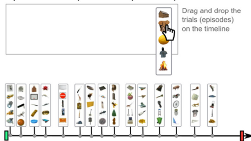
Figure 1. The paradigm and assessment of temporal representation. a , Outline of experiment with the top row showing the number of runs and tests performed after all stimuli had been presented (see also Figure S1d), and the bottom row showing the experimental design within a single run. The encoding part of the paradigm involved episodic learning, followed by a cross-fixation period, and, subsequently, an odd-even judgment task. There were 16 unique episodes presented within each run. b , Each episode consisted of five events (object presentations). A green screen marked the start of the episode and a red screen marked the end ("episode boundaries"). c , After the Odd-even judgment, the participant's recall of the episode was evaluated in the Event test, in which the participant positioned the objects he had seen (i.e., "events") by dragging and dropping them onto an empty timeline representing the entire episode. d , At the end of a run, after having learned 16 event sequences, the participant completed the Episode test and the Object association test (see Figure S1c). In the Episode test, the participant indicated at what point episodes occurred within a run, by dragging-and-dropping the episodes (defined by the objects presented in them) onto an empty timeline representing the entire run. e , Representation of time consists of metric time, which represents the exact onset of specific events and episodes, and chronological time which represents the order of the events and episodes. f , From the Event test, metric and chronological measures within episodes were obtained. The top row shows the actual response from one participant, with colors indicating object identity and the green and red screen indicating the temporal boundaries of the episode. Metric time M1 reflects the degree to which the participant's response preserved the exact timing of the events relative to each other (Temporal pattern M1 ) and the exact onset of the events relative to the temporal boundaries of the episode (Temporal boundary M1 ) (see Methods and Figure S1a for a detailed explanation). Event order C1 reflects how many events were recalled in the correct order (independent of Temporal pattern M1 and Temporal boundary M1 ). g , From the episode test, the participant's recall of the timing and episode order across episodes was assessed. Metric time M2 reflects whether the participant's response preserved the timing of all sixteen episodes in a run, relative to each other, as well as relative to the start- and end of the run. Episode order C2 was estimated
