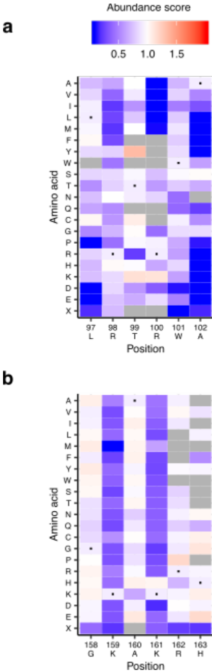
Figure 5—figure supplement 3. VKOR localization motif analysis. a , Heatmap of abundance scores for diarginine ER retention motif. X-axis shows residues and position. Color indicates abundance scores scaled as a gradient between the lowest 10% of abundance scores (blue), the WT abundance score (white) and abundance scores above WT (red). Grey indicates missing data. b , Heatmap of abundance score for dilysine ER retention motif. X-axis shows residues and position.
