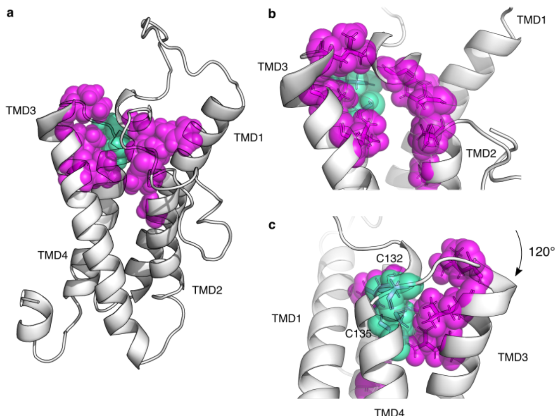
Figure 5. Functionally constrained positions reveal VKOR active site and critical cysteines.
