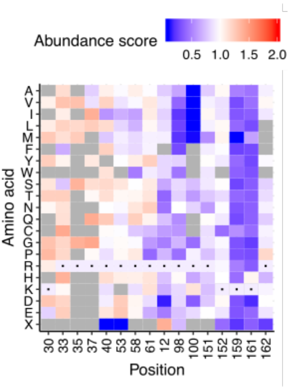
Figure 4—figure supplement 1. TMD1-adjacent positive residues show pattern of increased abundance. Heatmap of abundance scores for all arginines and lysines in VKOR. First four positions (K30, K33, K35, K37) are in or proximal to transmembrane domain 1. Heatmap color indicates abundance scores scaled as a gradient between the lowest 10% of abundance scores (blue), the WT abundance score (white) and abundance scores above WT (red). Grey bars indicate missing variants. Black dots indicate WT amino acids.
