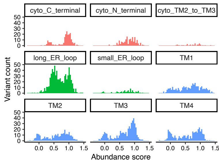
Figure 3—figure supplement 2. Specific domain abundance scores. Histograms of abundance scores for missense variants, grouped by domain and colored by cytoplasmic, ER lumenal, or transmembrane localization.
