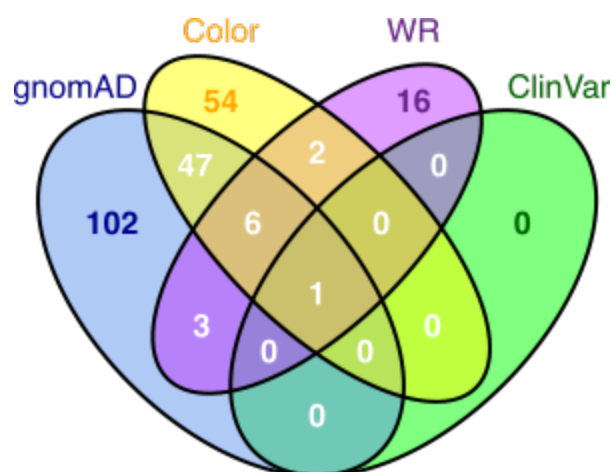
Figure 6—figure supplement 1. Human VKOR variant curation summary. Venn diagram of VKOR missense variants present in gnomAD v2 and v3, ClinVar, Color Genomics, a commercial genetic testing company, and literature-reported warfarin resistant variants.
