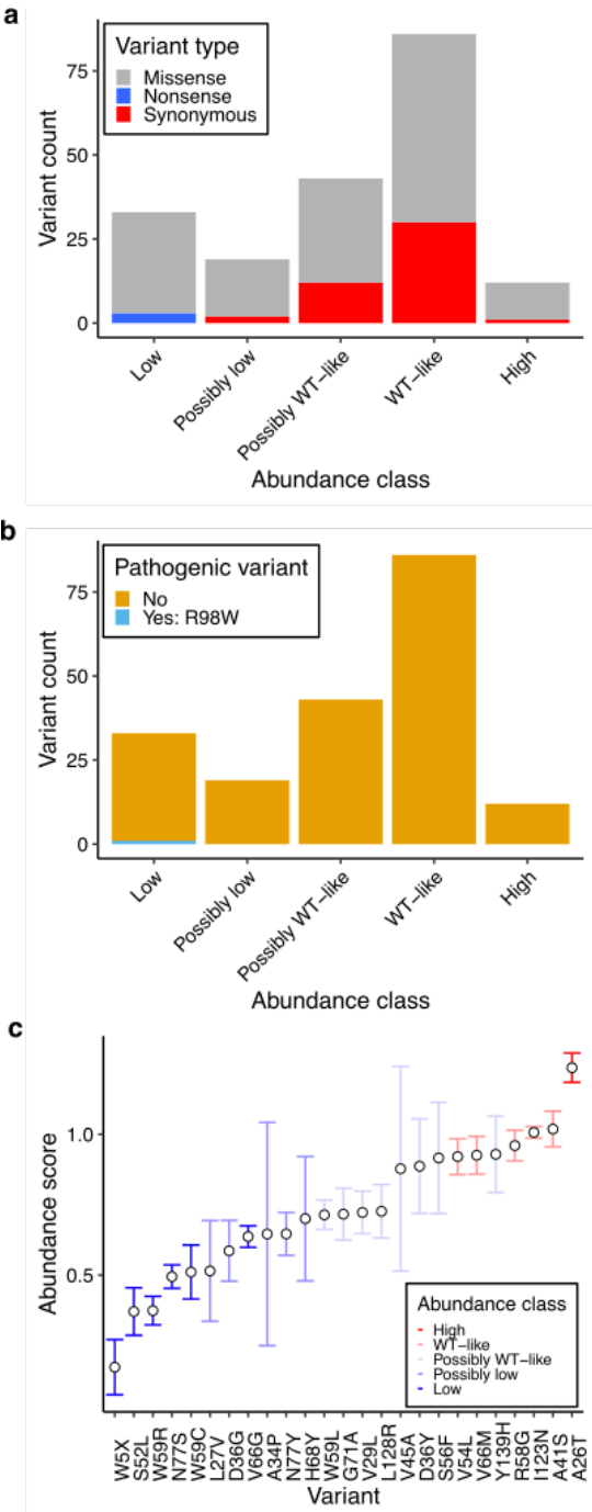
Figure 6. Characterization of human variants using abundance and activity data. a , Histogram of abundance classifications for variants from gnomAD, ClinVar, and Color Genomics. Nonsense variants colored in blue, synonymous in red, and missense in grey. b , Histogram of abundance classifications for same variants in a , colored by pathogenicity. The only variant known to cause disease, R98W, is colored in blue. All other variants shown in yellow. c , Scatterplot
