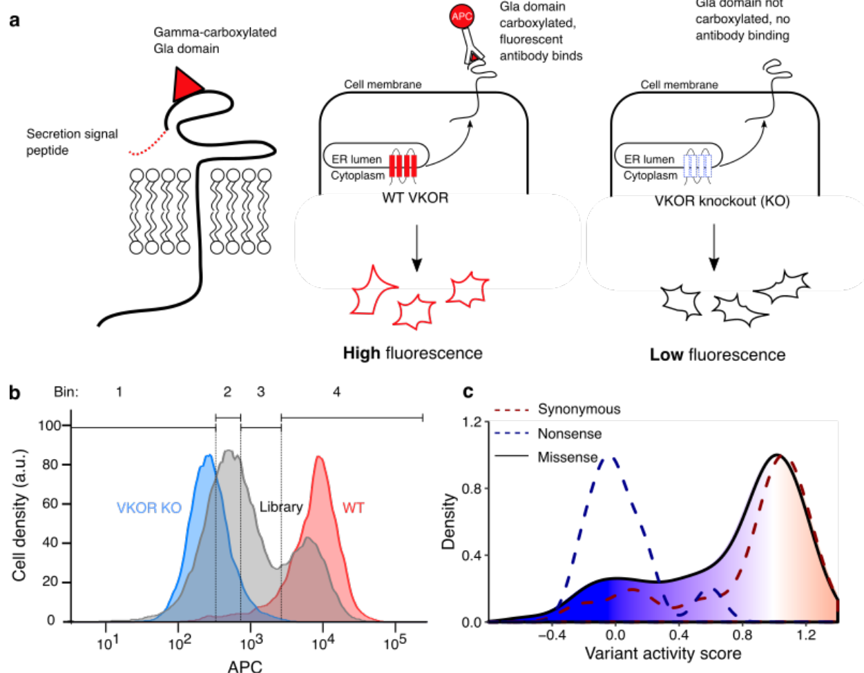
Figure 2. Multiplexed measurement of VKOR variant activity using a gamma-glutamyl carboxylation reporter. a, left panel , a Factor IX Gla domain reporter is expressed in HEK293 cells and consists of a prothrombin pre-pro-peptide which allows for processing and secretion, a Factor IX Gla domain, and Proline rich Gla protein 2 (PRGP2) transmembrane and cytoplasmic domains. middle panel , Cells expressing WT VKOR carboxylate the reporter Gla domain, which, upon trafficking to the cell surface, can be stained using a carboxylation-specific antibody conjugated to the fluorophore APC. VKOR knockout cells do not carboxylate the reporter, so the fluorescent antibody does not bind. b , Density plots of HEK293 activity reporter cells stained with APC-labeled carboxylation-specific antibody expressing no VKOR (blue, n = 7,188 ), WT VKOR (red, n = 4,107 ), or the VKOR variant library (grey, n = 41,418 ). Quartile bins
