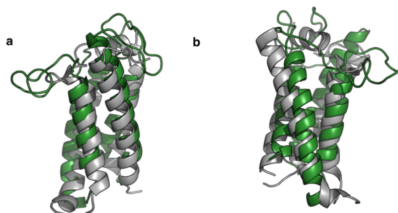
490 491 Figure 3—figure supplement 1. Bacterial VKOR structure and EV-couplings folded model 492 are highly similar. a , Pymol graphic showing overlap between EVcouplings-folded model of 493 VKOR (shown as a cartoon in green) compared to the bacterial structure (PDB: 4NV5, shown 494 as a cartoon in grey). b , shows the same two structures, rotated 120°C.
