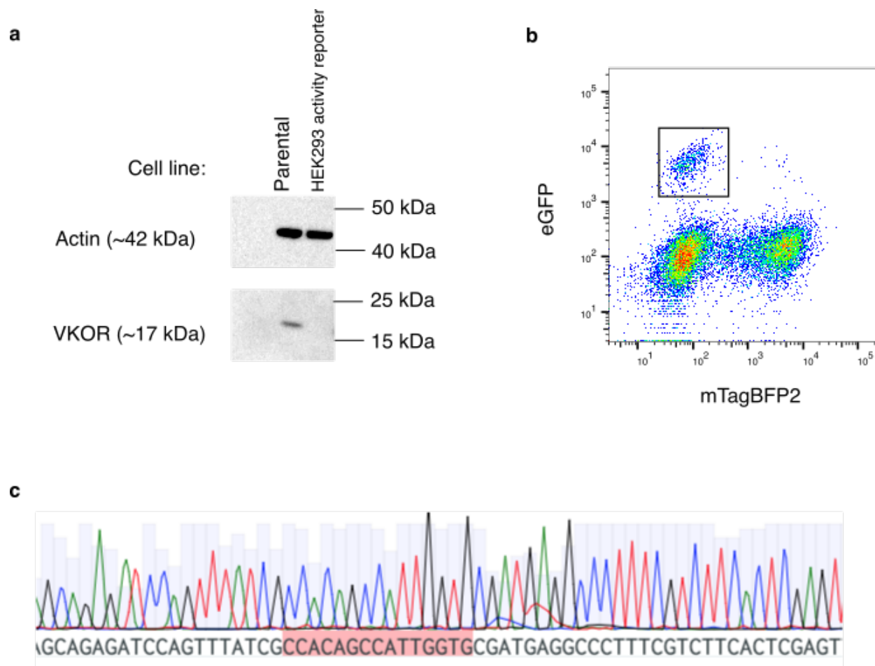
Figure 2—figure supplement 1. HEK293 VKOR activity reporter cell line characterization.
