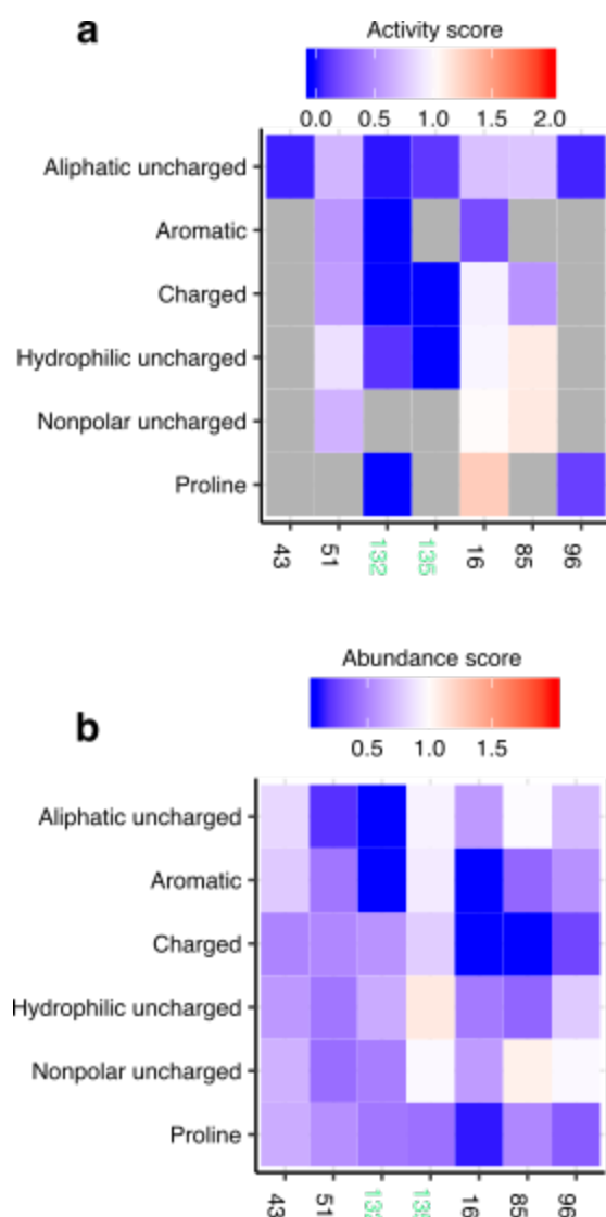
Figure 5—figure supplement 2. Conserved cysteine analysis. a , Heatmap of activity scores for cysteines. Catalytic cysteines C132 and C135 labeled in green. Color indicates activity scores scaled as a gradient between the lowest 10% of activity scores (blue), the WT activity score (white) and activity scores above WT (red). Grey indicates missing data. b , Heatmap of abundance scores for cysteines. Catalytic cysteines C132 and C135 labeled in green. Color legend same as described in a , applied to abundance scores.
