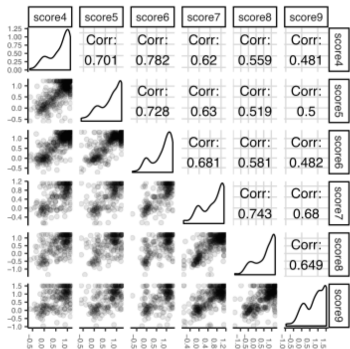
Figure 2—figure supplement 2. Correlations of activity assay replicates. Pairwise score correlations between replicate sorting experiments of VKOR activity. Six replicates of the activity assay were performed. Pearson's correlation coefficients are shown. Score numbers in this panel correspond to replicate numbers shown in Supplementary Table 2.
