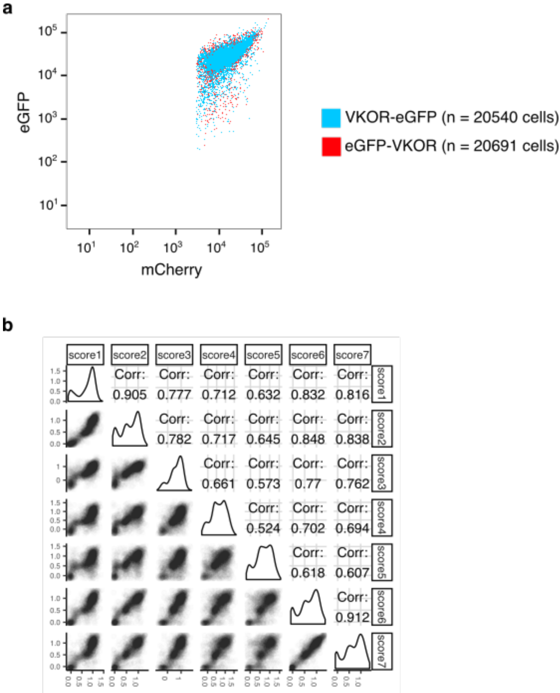
Figure 1—figure supplement 1. VKOR abundance assay pilot experiment and replicate correlations. a , Scatterplot of eGFP vs. mCherry fluorescence for cells expressing either C-terminally eGFP-tagged VKOR (VKOR-eGFP, blue) or N-terminally eGFP-tagged VKOR (eGFP-VKOR, red). b , Pairwise abundance score correlations between replicate sorting experiments.
