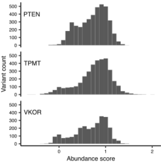
Figure 4—figure supplement 2. Trimodality of missense variant abundance scores is unique to VKOR. Histograms of abundance scores for missense variants for three proteins: PTEN, TPMT, and VKOR.
