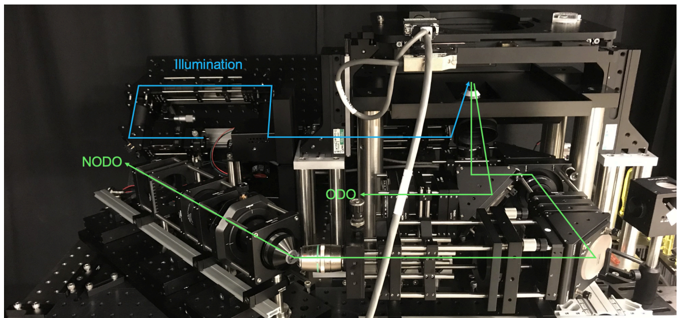
Supplementary Figure 15 | Hybrid OTLS system in practice. (a) Photograph of the hybrid OTLS system. The illumination optics (blue line) are housed on a single 18 x 36 in. breadboard angled at 45 deg. The NODO and ODO optics (green lines) are placed on flat breadboards. The NODO imaging optics are housed on a series of connected breadboards, which can be translated in one direction to adjust the distance between the imaging optics and the back focal plane (BFP) of the multi-immersion objective lens. This enables fine alignment when switching the immersion medium, as the axial position of the BFP of the objective lens is a function of refractive-index, n . The position of the BFP relative to the flange of the objective lens is approximately -11.75 \text{ mm} - 22.90 \text{ mm} \times n + 5.87 \text{ mm} \times n^2 . Finally, the remote objective lens, final tube lens, and sCMOS camera are all positioned atop another breadboard, which can be translated and rotated to align the remote imaging arm with respect to the remote focus.
