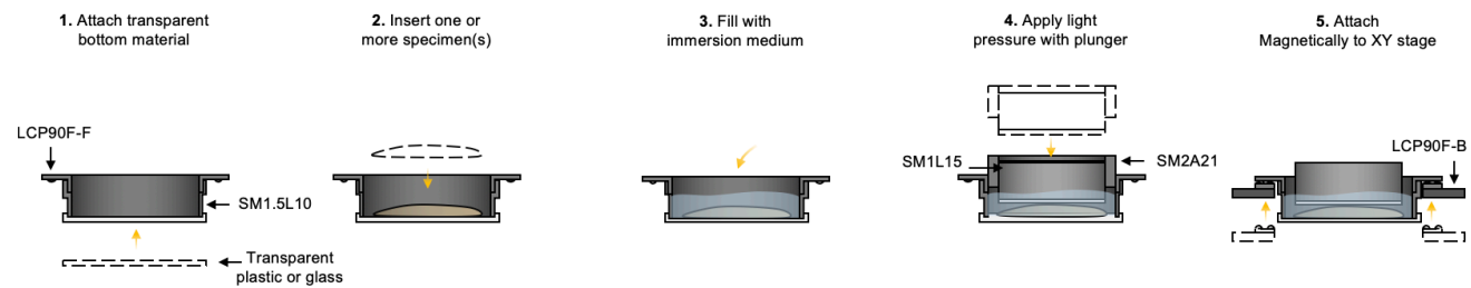
Supplementary Figure 8 | Specimen mounting for hybrid OTLS system. Our new hybrid OTLS system using an improved specimen holder and mounting procedure. The circular holder features a bottom thread, to which an interchangeable transparent bottom material can be attached. Specimens are then inserted into the holder from the top, and the holder is filled with an index-matching immersion medium. Light pressure is then applied to the top of the tissue using a plunger. The bottom surface of the plunger is the same transparent material as the bottom of the holder, which reduces back reflections when imaging the deepest surface of the specimen. Finally, the entire specimen holder is magnetically attached to the XY stage.
