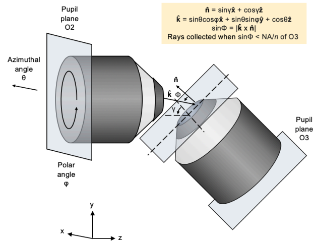
Supplementary Figure 20 | Numerical simulation geometry. Based on a spherical coordinate system, each ray exiting objective lens O2 can be described by an azimuthal angle, \theta , and polar angle, \phi . The direction of that light ray is then described as \hat{k} = \sin \theta \cos \phi \hat{x} + \sin \theta \sin \phi \hat{y} + \cos \theta \hat{z} . The surface normal from objective lens O3 is described by \hat{n} = \sin y \hat{x} + \cos y \hat{z} . Therefore, the angle of incidence of the ray on O3 is given by \sin \Phi = |\hat{k} \times \hat{n}| . The incident pupil plane from O2 can then be clipped by the NA of O3.
