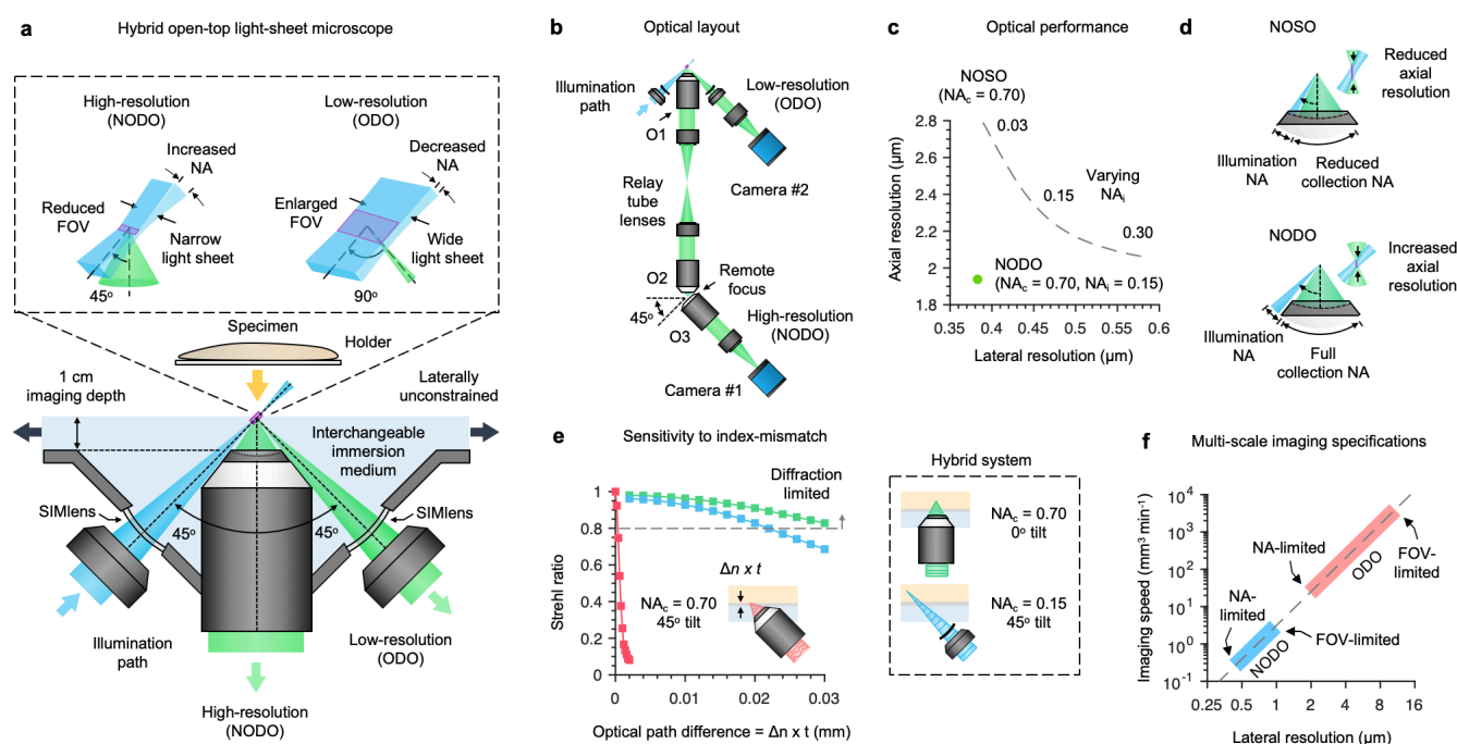
Fig. 2 | Hybrid open-top light-sheet (OTLS) microscope. (a) Light-sheet illumination (blue beam) is provided from an off-axis (45-deg) objective lens on the left. For high-resolution imaging, a vertically oriented objective lens images the fluorescence signal (green beam) from a small field of view (FOV) via a non-orthogonal dual-objective (NODO) configuration. For low-resolution imaging, a separate 45-deg off-axis objective lens (right side) images the fluorescence signal from a large FOV via an orthogonal dual-objective (ODO) configuration. The light-sheet illumination properties (thickness, width, depth of focus) are tuned for the NODO and ODO paths to enable multi-scale imaging. (b) The optical layout of the NODO configuration is inspired by a non-orthogonal single-objective (NOSO) light-sheet microscopy technique that has been gaining traction in recent years. Fluorescence is collected by the primary objective lens (O1) and is relayed to a remote focus using a pair of tube lenses and a second objective lens (O2). The final remote objective lens (O3) is oriented at 45 deg to re-image the tilted light sheet onto a camera. The ODO path simply images the light sheet from the illumination path directly onto a second camera. (c-d) An advantage of NODO is that the illumination and collection beams do not have to share one objective lens and can be oriented with a larger crossing angle, both of which enable superior axial and lateral resolution compared with NOSO, in which those parameters must trade off. (e) Furthermore, unlike ODO, which is extremely sensitive to refractive-index-mismatch at higher NAs (red curve), NODO uses a collection objective lens oriented in the normal (vertical) direction, which is much less sensitive to index-mismatch (green curve). The index-mismatch sensitivity for the low-resolution ODO collection path of the hybrid OTLS system is also shown (blue curve). Note that the index-mismatch is represented by the optical path difference, \Delta n \times t , where \Delta n is the refractive-index difference between the holder material and immersion medium/tissue, and t is the thickness of the holder. A Strehl ratio of >0.8 is often considered ideal “diffraction-limited” imaging. (f) Finally, our hybrid OTLS system allows the user to trade-off between imaging speed and resolution as shown in the plot, roughly corresponding to the resolution levels that are achievable by a standard widefield microscope with a turret of 2X to 40X objective lenses (volumetric imaging speeds of \sim 0.3 \text{ mm}^3 \text{ sec}^{-1} to 3000 \text{ mm}^3 \text{ sec}^{-1} ).
