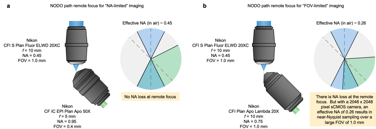
Supplementary Figure 6 | Remote-focus layout for NODO imaging. Our NODO imaging architecture enables the use of commercial air objective lenses at the remote focus, as opposed to bespoke objective assemblies (a) Using a crossing angle of 45 deg, the effective NA of the NODO imaging path is a lossless \sim 0.45 (in air) when using a 50x 0.95 NA air objective lens. This configuration provides NA-limited imaging (b) By switching to a 20x 0.75 NA remote objective lens, the effective NA is reduced to \sim 0.26 (in air). Despite the loss in effective NA, Nyquist sampling at this NA on a standard 2048 x 2048 pixel sCMOS camera yields a field of view of \sim 1.0 mm. Therefore, this configuration provides FOV-limited imaging.
