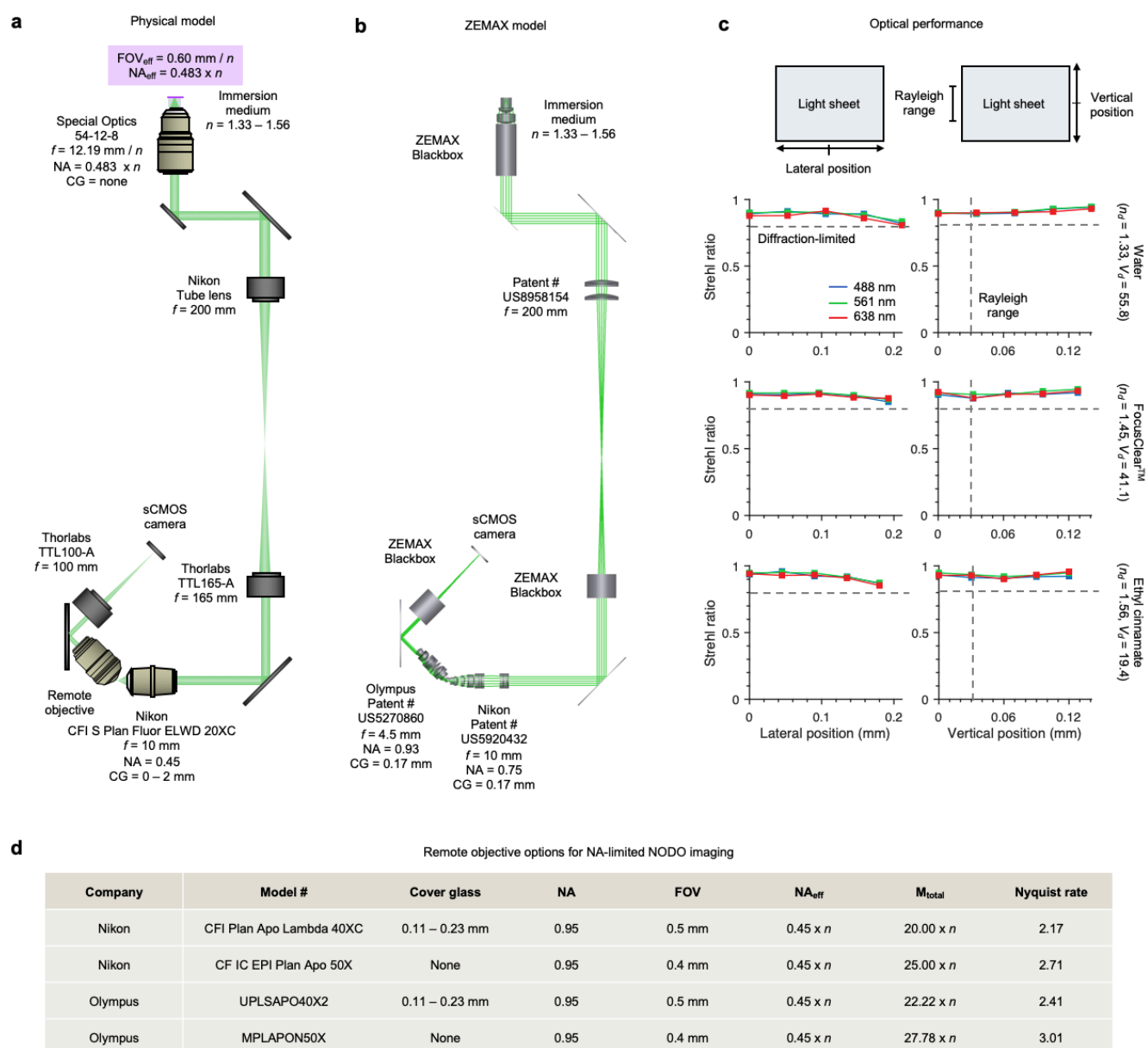
Supplementary Figure 10 | NA-limited NODO collection optics model. (a) The physical model of the NA-limited NODO collection optics within the hybrid OTLS system. Fluorescence is collected by a multi-immersion objective lens ( f = 12.19 / n ) and relayed to a remote focus using tube lenses ( f = 200 and 165 \text{ mm} ), and a 20X objective lens ( f = 10 \text{ mm} ). For aberration free imaging, the total magnification from the specimen to the remote focus should be equal to n . For the optics chosen, the total magnification is extremely close: \sim 0.994 n . The remote imaging arm is tilted by 45 deg and uses a remote objective lens and tube lens ( f = 100 \text{ mm} ) to image the remote focus onto a sCMOS camera. The effective numerical aperture of the multi-immersion objective lens is 0.45 \times n , with an effective FOV of 0.60 \text{ mm} / n . (b) Corresponding ZEMAX model. Lens prescriptions or blackbox files were available for all components, except for the remote imaging objective lenses. For these objective lenses, US Patent # 5920432 and #5270860 were used. (c) Results for the Strehl ratio as a function of lateral position across the width of the sheet (left) and along the length of the sheet (right). The three rows correspond to different immersion media, water ( n \sim 1.33 ), FocusClear™ ( n \sim 1.46 ), and ethyl cinnamate ( n \sim 1.56 ). The colored
