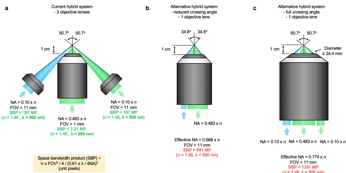
Supplementary Figure 18 | Alternative designs based on customized objective lenses. (a) The current hybrid OTLS system uses three objective lenses for illumination, high-resolution NODO imaging, and low-resolution ODO imaging. These objective lenses are all commercially available. (b) In theory, all three optical paths could be incorporated into a single objective lens. This theoretical objective lens would require an effective NA of 0.568 (in air) and a large 11 mm field of view (FOV). This NA would reduce the crossing angle of the illumination and collection beam paths but provide identical NAs to the current system. However, these specifications are extremely demanding, and would require a space bandwidth product (SBP) of ~ 991 megapixels (MP), which is far beyond any currently produced objective lenses. (c) Another alternative design would maintain the same crossing angles as the current system, instead delivering and collecting all beam paths through a single massive objective lens. The specifications for this objective lens would be even more demanding, with SBP ~ 1351 MP. These alternative designs are highly speculative, and it is not likely that these objective lenses would be technically or financially feasible to design and/or manufacture.
