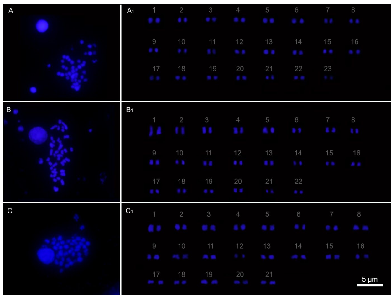
Figure 3: Representative metaphase and karyogram of (A and A1) T. tagusensis (2n= 46), (B and B1) T. coccinea (2n= 44), and (C and C1) Tubastraea sp. (2n= 42). Two metaphase plates of each morphotype were counted. Scale bar 5 μm.
