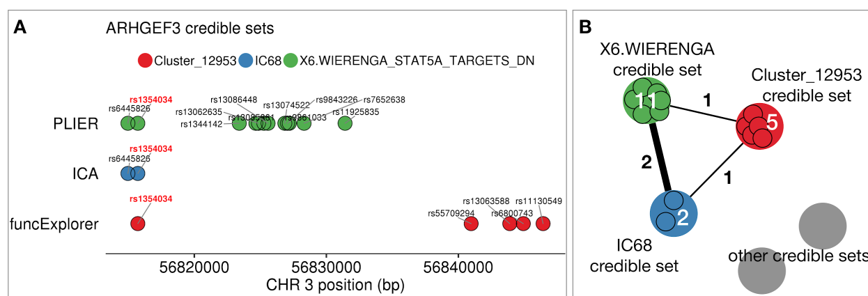
Figure S2. Aggregating fine mapping credible sets in the example of ARHGEF3 trans -eQTL locus. We performed fine mapping on the lead variants of every gene module to find corresponding credible sets (see “Methods”). A The figure shows an example of three credible sets on chromosome 3 for three gene modules: IC68 from applying ICA to integrated expression data; Cluster_12953 from funcExplorer and X6.WIERENGA_STAT5A_TARGETS_DN from PLIER, both applied to gene expression data from platelets. The associations shown here were detected in platelets. Each circle represents a variant belonging to the corresponding credible set and the different credible sets are distinguished by colors. B The credible sets are combined into a graph structure where every node is a credible set of variants and we define an edge between two nodes if they share at least one variant. Grey circles represent all the credible sets from other genomic regions. Here the number of shared variants is shown on the edges and the number of variants belonging to the credible set is shown on the nodes. We searched for connected components, grouped these credible sets together and defined a lead variant for every group based on the largest average posterior inclusion probability (PIP) value within the group. In this example, as all the credible sets share a single variant, rs1354034, then they are grouped together and the overlapping variant with largest PIP is rs1354034.
