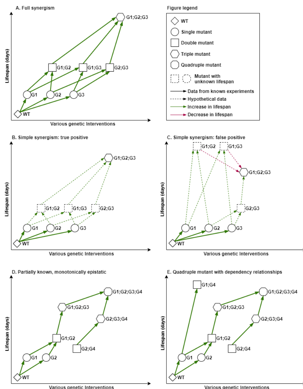
Fig. 2. Synergism and epistatic monotony. A. Example of “full” synergism shown for a 3-mutant. B. True positive example of “simple” synergism approximation, in which the synergistic combination is correctly inferred based on the available data. The missing data (dotted nodes and edges) would not contradict the prediction. C. False positive example for the “simple” synergism approximation. The example shows an “incorrectly inferred” synergistic combination which may be disproved later by data that is currently unknown (dotted nodes G1;G2 and G1;G3 are even longer lived than G1;G2;G3). In
