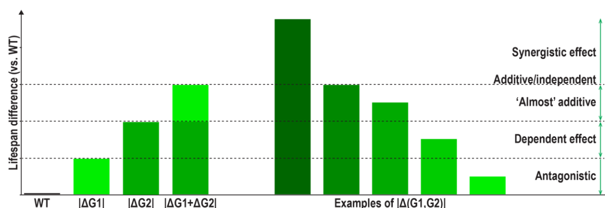
Fig. 1. Lifespan epistasis categories defined for combinations of two genetic interventions. Depicted are synergistic, additive, almost additive, dependent and antagonistic relationships, categorized based on the difference between the effect of the combination and the sum of the effects of individual genetic interventions. By these definitions, we are considering that individual gene interventions resulting in changes with opposite lifespan modulations cannot be directly assessed for epistasis.
