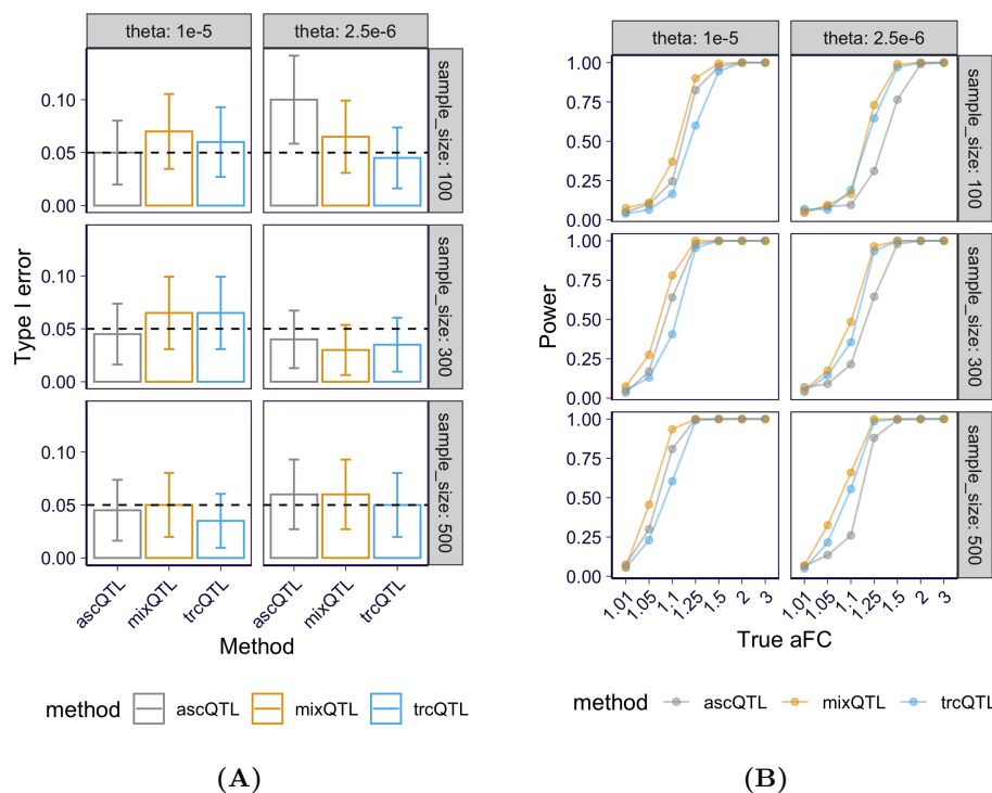
Figure 2: QTL mapping performance for mixQTL and approaches based on either total reads (trcQTL) or allele-specific reads (ascQTL) on simulated data. Each panel presents the results for two relative abundances of the gene, \theta , and three sample sizes. (A) Type I error (y-axis) at a 5% significance level across methods (x-axis). The dashed line represents the desired error rate under the null hypothesis. The error bar indicates the 95% confidence interval (CI) in observed error rate estimated from 200 replicates. (B) Power (y-axis) at a 5% significance level across methods under a range of true aFC values (x-axis). Power is defined as the fraction of eQTLs passing the significance threshold.
