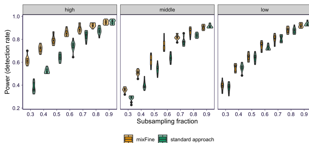
Supplementary Fig. S12. Performance of mixFine on GTEx v8 whole blood RNA-seq stratified by expression level. At each subsampling level (x-axis), the fraction of “consensus SNPs” being detected is shown on the y-axis. Each panel shows the results of genes stratified by expression level tertiles.
