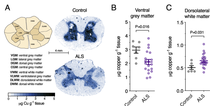
Figure 2. Copper in sporadic ALS-affected spinal cord relative to anatomical distribution. A , Schematic illustration of anatomical regions of interest in transverse plane of human spinal cord sections and representative anatomical heatmaps for copper as measured using laser ablation-inductively coupled plasma-mass spectrometry (LA-ICP-MS). B , Copper content in ventral grey matter region of interest in human spinal cord measured using LA-ICP-MS. C , Copper content in dorsolateral white matter region of interest in human spinal cord measured using LA-ICP-MS. Results for additional regions of interest are shown in Table 2. Symbols shown in B and C represent individual controls and ALS cases. Lines in B and C represent mean \pm S.E.M. P values represent significance.
