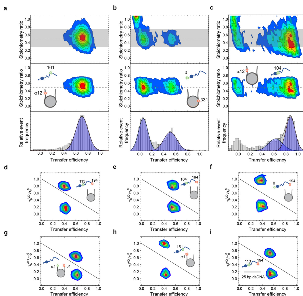
Supporting Information Figure 5 | Representative examples of stoichiometry measurements and fluorescence lifetime analysis of H1-nucleosome and H1-DNA complexes. a-c, 2D-histograms of stoichiometry ratio vs. transfer efficiency from intermolecular FRET between donor-labeled H1 and acceptor-labeled nucleosome using pulsed interleaved excitation. The labeling positions are indicated in the schematics above the graphs. The gray-shaded areas indicate the stoichiometry ranges used for filtering out donor-only fluorescence bursts. A 1:1 complex results in a stoichiometry ratio of 0.5 (dashed horizontal line). Most of the transfer efficiency histograms in Fig. 3 contain a single population, as in (a). In some cases, such as in (b), a clear second population is observed that is well separated from the donor-only population. In other cases, i.e. in (c), an additional residual population at a transfer efficiency close to zero can remain even after filtering due to a large signal from molecules lacking an active acceptor dye. d-i, Fluorescence lifetime analysis. Plots showing the fluorescence lifetimes of Alexa Fluor 488 ( \tau_D^D ) and Alexa Fluor 594 ( \tau_A^A ) normalized by the intrinsic donor lifetime ( \tau_D^0 ) as a function of transfer efficiency. If fluctuations in transfer efficiency occur on a timescale between the donor fluorescence lifetime and the burst duration ( \sim 4 ns-1 ms), the normalized donor and acceptor lifetimes cluster above and below the static FRET line (solid diagonal line) 70,71 , respectively. The substantial deviations from the diagonal indicate a broad distribution of distances in all samples, as previously observed for intrinsically disordered proteins 47,88 . d, H1 113-194 + unlabeled nucleosome; e, H1 104-194 + unlabeled nucleosome; f, H1 10-194 + unlabeled nucleosome; g, Nucleosome \alpha 1-\beta 1 + unlabeled H1; h, H1 151 + nucleosome \alpha 1 ; i, H1 113-194 + 25 bp dsDNA.
