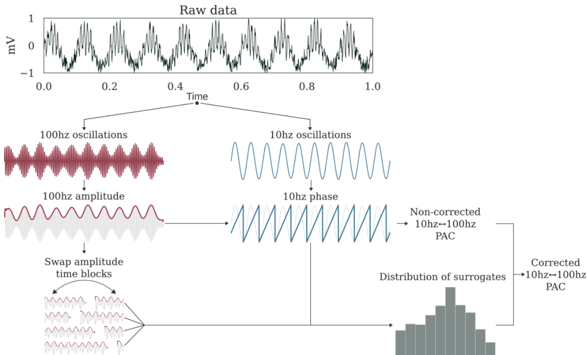
Figure 1 : Estimation process of a corrected 10->100 hz PAC. For illustration, here simulated raw data contains a coupling between a 10 hz phase and a 100 hz amplitude. First, the raw data is respectively filtered with bandpass filters centered on 100hz and 10hz. Then, the complex analytic form of each signal is obtained using the Hilbert transform. The phase is extracted from the 10Hz signal (angle of analytic signal) and power from the 100Hz signal (amplitude of analytic signal). An uncorrected PAC measure is obtained from these two signals. To estimate the null distribution of the measure in the absence of any genuine coupling, the amplitude signal is split into two blocks at a random time point and the temporal order of those two blocks is swapped. Then, the PAC is estimated using this swapped version of amplitude and the originally extracted phase. By repeating this process and cutting at a random point, for example 200 times, we can obtain a distribution of surrogate values for which there is no genuine coupling. Finally, a corrected PAC estimate is obtained through z-score normalization of the uncorrected PAC using this distribution.
