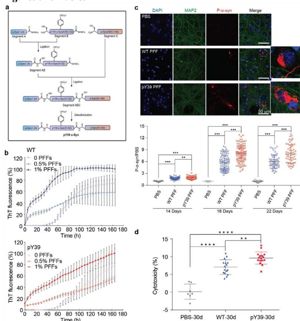
Fig. 1. pY39 \alpha -syn synthesis and pathology. (a) Workflow of the semi-synthesis of human pY39 \alpha -syn. (b) ThT kinetic assays of the WT and pY39 aggregation with or without the addition of PFFs. Mol% of added PFFs are indicated. Data shown are mean \pm s.d., n=3. (c) \alpha -Syn PFFs induce endogenous \alpha -syn aggregation in rat primary cortical neurons. Primary neurons were treated with 100 nM \alpha -syn PFFs at DIV8 for 14 days. Fixed neurons were stained for DAPI (blue), MAP2 (green) and pS129 \alpha -syn (red) and imaged by confocal microscopy. Measurement of the mean gray value of pS129 \alpha -syn was shown in below. The images were analyzed by Image J. The mean gray values of pS129 \alpha -syn were normalized to that of PBS. >10 images were randomly taken for each sample. >5 individual samples were analyzed for each time
