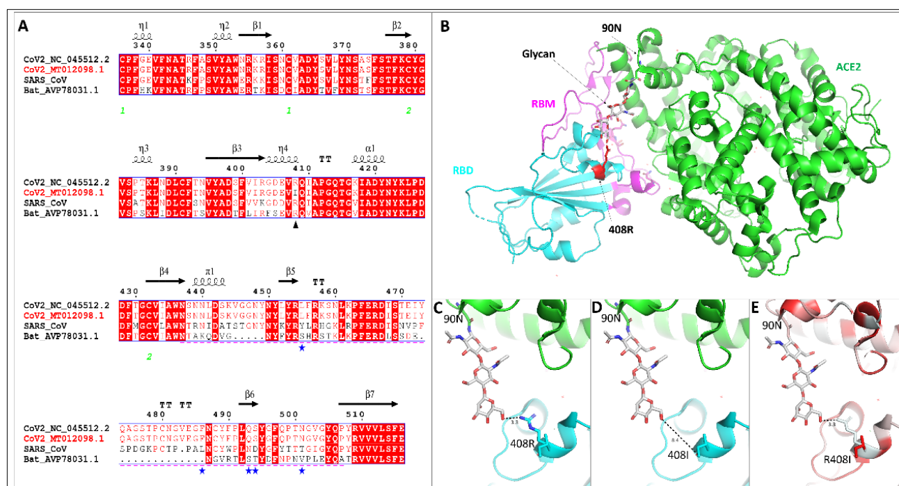
Figure 4. Sequence alignment and protein structural analyses of the mutation in RBD of SARS-CoV-2. A ) Sequence alignment of RBDs. ▲ : R408I mutation; --- : receptor binding motif (RBM); * : RBD-interacting sites. B ) Overall position of the identified mutation relative to: RBD (cyan), ACE2 (green) with RBM (pink) and Glycan (grey). C,D ) Display the disrupted hydrogen bond by the R408I mutation. “---”: distance in Å. E ) Hydrophobic profile changes due to R408I mutation, with red and white colours representing the highest hydrophobicity and the lowest hydrophobicity respectively. All amino acid number according to the S protein of SARS-CoV-2 (NC_045512.2) and human ACE2, respectively.
