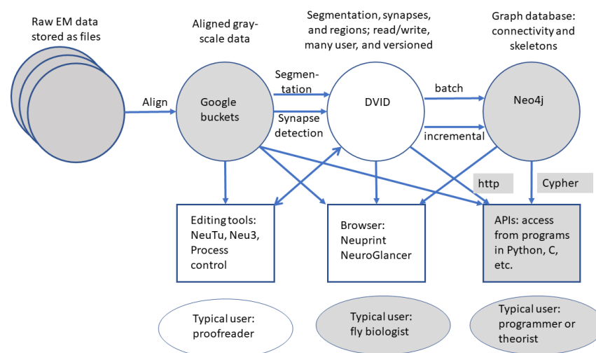
Figure 18. Overview of data representations of our reconstruction. Circles are stored data representations, rectangles are application programs, ellipses represent users, and arrows indicate the direction of data flow labeled with transformation and/or format. Filled areas represent existing technologies and techniques; open areas were developed for the express purpose of EM reconstruction of large circuits.
