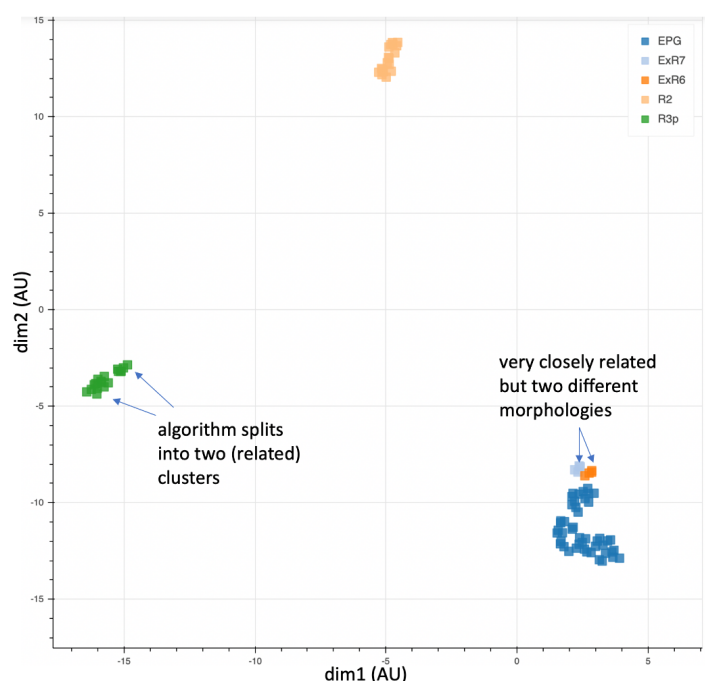
Figure 13. Cells of five types plotted according to their connectivities. Coordinates are in arbitrary units after dimensionality reduction using UMAP(McInnes et al. , 2018). The results largely agree with those from morphological clustering but in some cases show separation even between closely related types.
