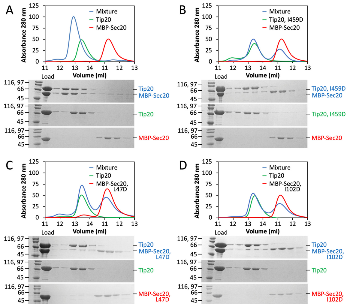
Figure 2. Structure-guided disruption of E. gossypii Tip20•Sec20 complex formation. A , Size exclusion chromatography demonstrates robust binding (blue) between wild-type E. gossypii Tip20 (green) and MBP-Sec20 NTD (red). B-D , Substitution of Tip20 Ile-459, Sec20 Leu-47, or Sec20 Ile-102 with aspartate abolishes binding of Tip20 to MBP-Sec20.
