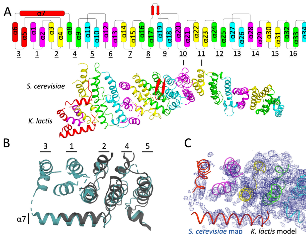
Figure S6. Additional N-terminal regions modeled for K. lactis Sec39. A , Above, topology of Sec39, with color-coding to illustrate the correspondence between individual \alpha -helices and hairpins. Below, S. cerevisiae and K. lactis Sec39 superimpose with an RMSD of 3.7 Å over 436 residues. Superimposition at the C-terminus shows that the two structures differ primarily due to bending between layers 10 and 11 (indicated). B , Four additional helices were modeled at the N-terminus of K. lactis Sec39 (cyan), representing hairpins 1 and 3. In addition, the N-terminus of \alpha 7 was extended relative to S. cerevisiae Sec39 (3K8P, gray). The two structures are superimposed at the N-terminus. C , Contoured at 1 \sigma , the S. cerevisiae 2Fo-Fc map (3K8P, blue mesh) contains weak density, not previously interpreted, corresponding to hairpins 1 and 3 as modeled in the K. lactis structure.
