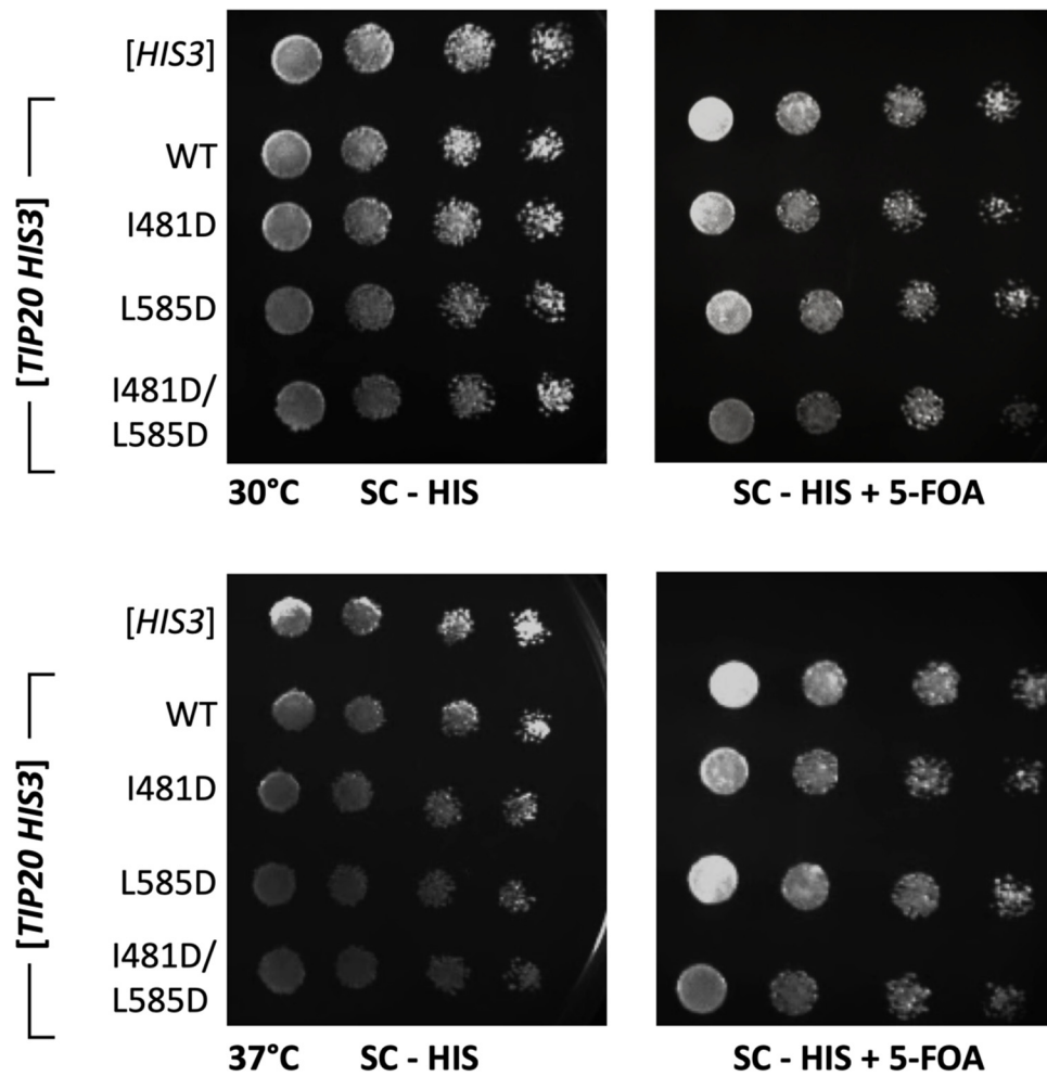
Figure S5. S. cerevisiae Tip20 interface mutants are viable. As in Figure 4, mutant alleles of S. cerevisiae Tip20, linked to His3, were tested for viability upon counterselection against a wild-type copy of Tip20, linked to Ura3. Although an empty His3 plasmid was not able to support viability, all alleles of Tip20 tested were viable, even at elevated temperature.
