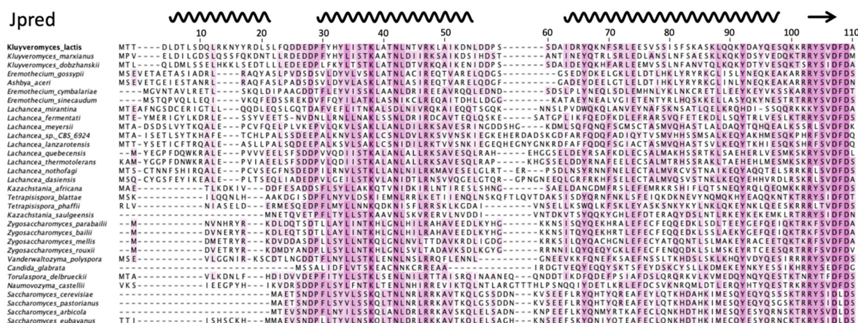
Figure S8. Secondary structure prediction suggests that the N-terminal domain of Use1 is \alpha -helical. Secondary structure prediction (61) identified three putative \alpha -helices in the N-terminal domain of K. lactis Use1. Because the first helix in the sequence is not conserved among some orthologues, including S. cerevisiae , it is possible that the long Ha helix observed in Use1 comprises the first two predicted helices. Sequence conservation is shown in purple.
