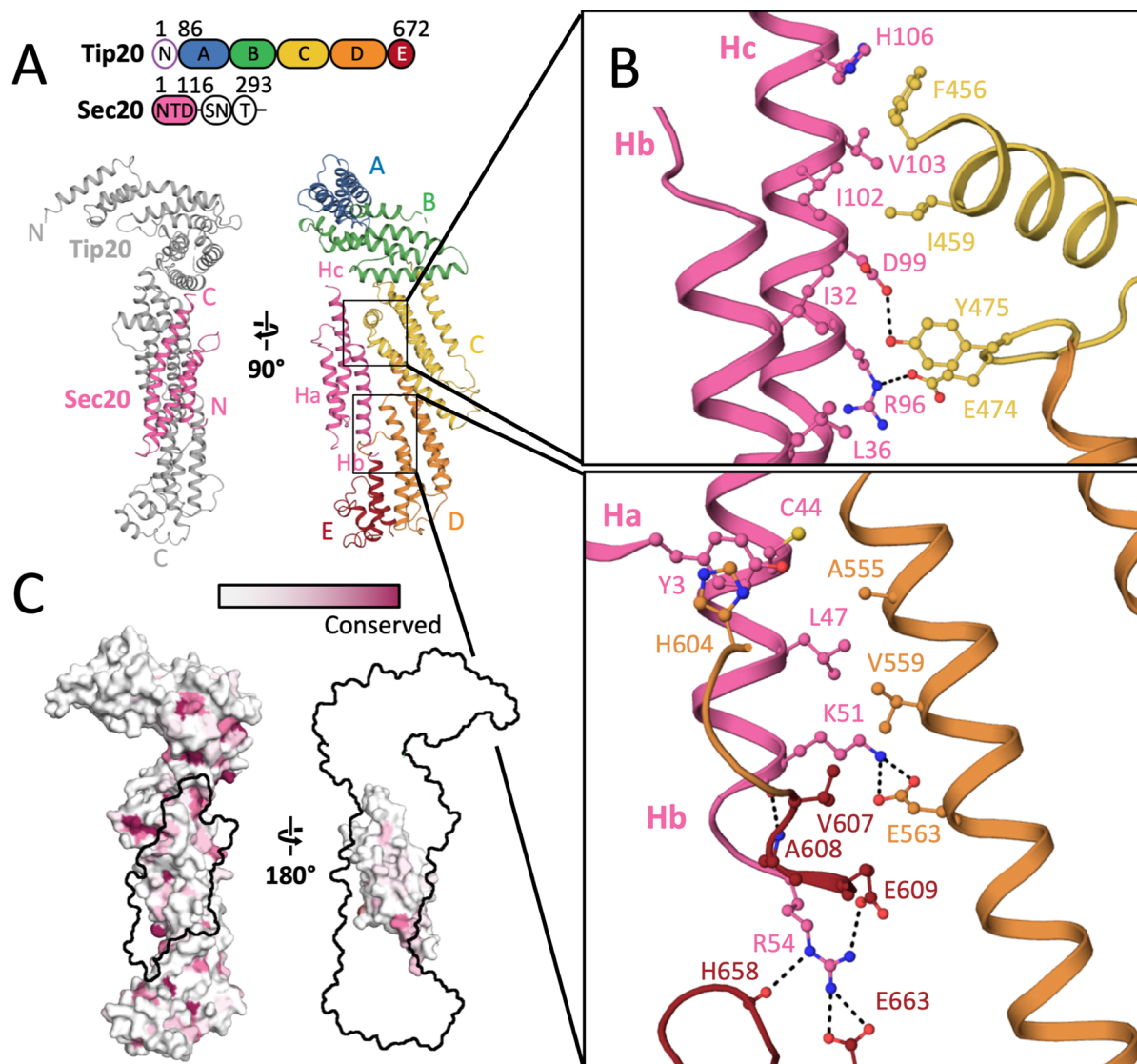
Figure 1. Structure of E. gossypii Tip20 A-E •Sec20 NTD complex. A , Sec20 NTD adopts an Habc fold, interacting with Tip20 domains C through E. The full domain architecture of the two proteins is cartooned above. The Dsl1 complex subunit Tip20 consists of an N-terminal Dsl1-interacting domain (N), followed by 5 CATCHR domains (A-E). The SNARE protein Sec20 consists of an N-terminal Habc domain (NTD), SNARE motif (SN), and transmembrane helix (T). B , Details of the Tip20•Sec20 interface. C , The interacting surfaces of Tip20 and Sec20 are not highly conserved.
