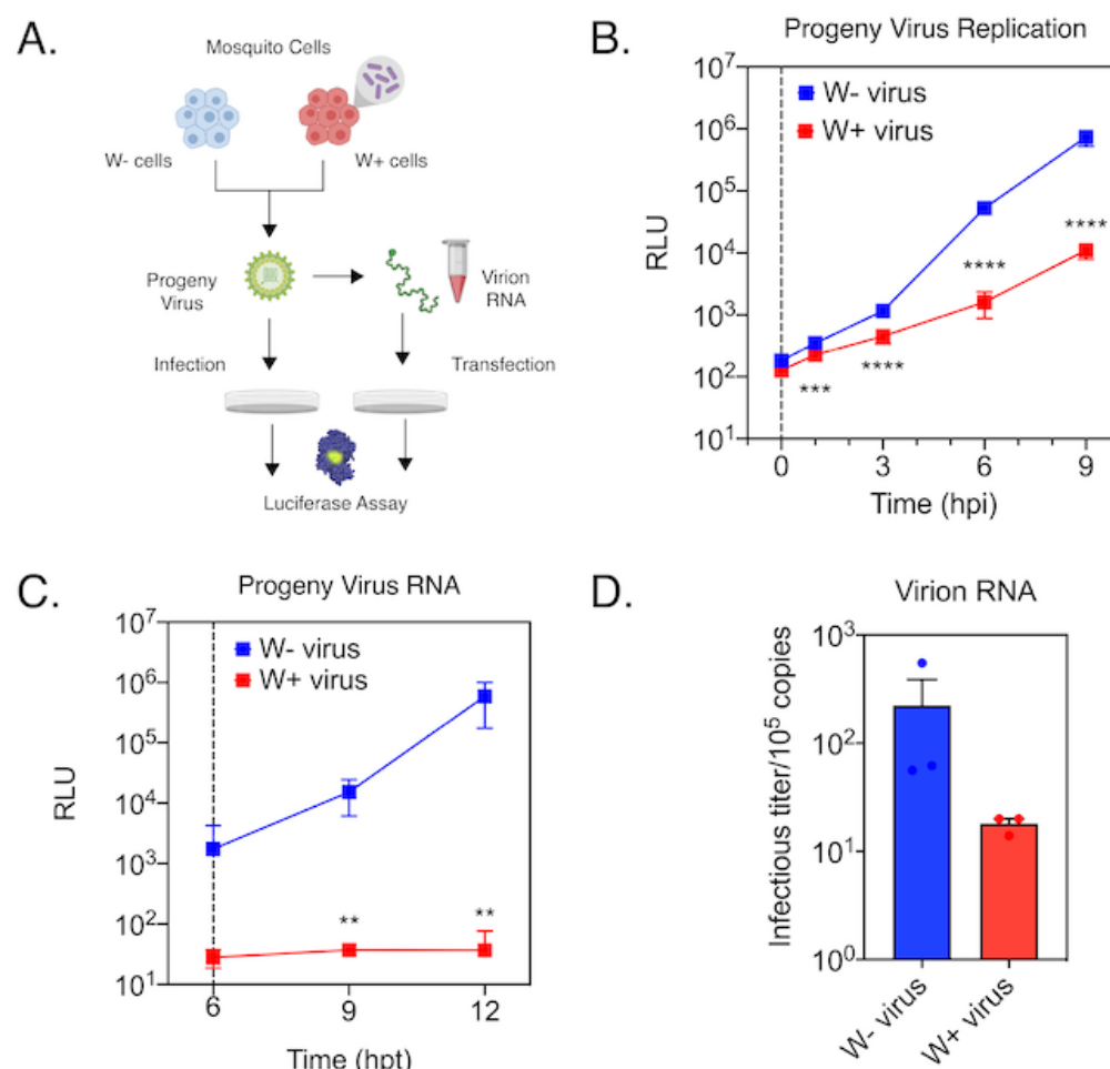
Figure 6. RNA encapsulated within progeny viruses derived from Wolbachia colonized cells are less infectious. (A) Sindbis viruses expressing nanoluciferase reporter gene (SINV-nLuc) were derived from RML12 mosquito cells with (W+ virus) or without (W- virus) Wolbachia (wMel) and were subsequently used to synchronously infect naïve BHK-21 cells at equivalent MOIs of 5 particles/cell. Cell lysates were collected at indicated times post infection and luciferase activity (RLU) was measured and used as a proxy to quantify viral replication. (B) Approximately 10 5 copies each of virion encapsidated RNA extracted from the aforementioned W+ and W- viruses were transfected into naïve BHK-21 cells and infectious titer was determined by the counting the number of plaques produced after 48 hours post transfection. (C) Replication kinetics of the previously isolated virion encapsidated RNA was determined by measuring luciferase activity following transfection into BHK-21 cells (RLU) as before. Error bars represent standard error of mean (SEM) of biological replicates (n=3). Student's t-test performed on log-transformed values. **P < 0.01, ***P < 0.001, ****P < 0.0001.
