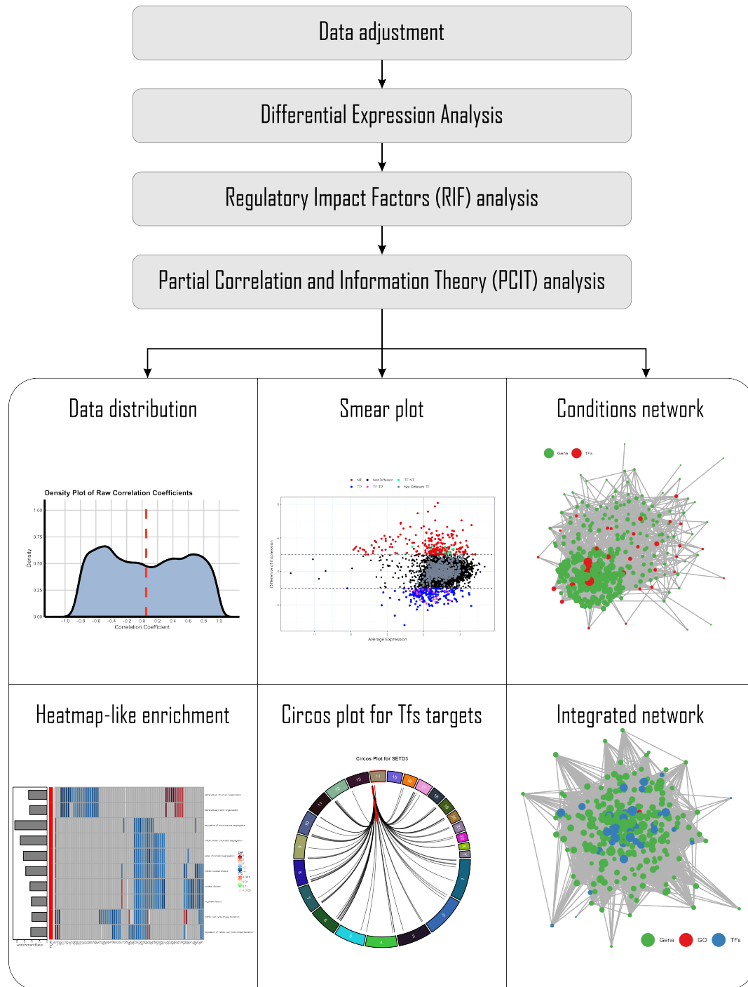
Fig. 1: Schematic of a CeTF workflow. The main functions of CeTF and their logical order are illustrated. Grey boxes signify the mandatory steps for the main analysis. The white box signifies the optional outputs from CeTF package, i.e. data distribution, smear plot, conditions network, heatmap-like enrichment, circos plot for TFs targets, integrated network, etc.
