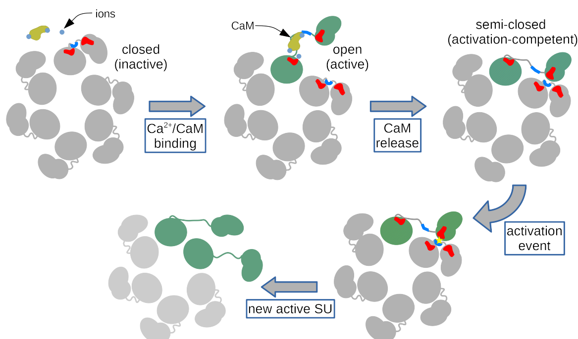
Figure 8: Steps in the activation of a CaMKII subunit. The first transition shows a closed (gray) SU (with negatively charged patches in red, and positively charged in blue) being affected by Ca 2+ /CaM (in yellow and light blue, respectively) and resulting in its opening (green SU). Once the complex is released, the SU is dynamically driven to a semi-closed conformation (green/white hatched SU), with its kinase domain getting close to a neighboring SU. The high negative charge of its kinase can interact with the high positive charge of the neighbor's linker, thus favoring a strong interaction that could lead to the phosphorylation of the latter (activation event). This newly phosphorylated SU, now with a partially neutralized linker, is not favored as before to stay in a closed conformation (the previous attraction hub-linker-kinase was weakened). Thus, the systems acquires a new active SU.
