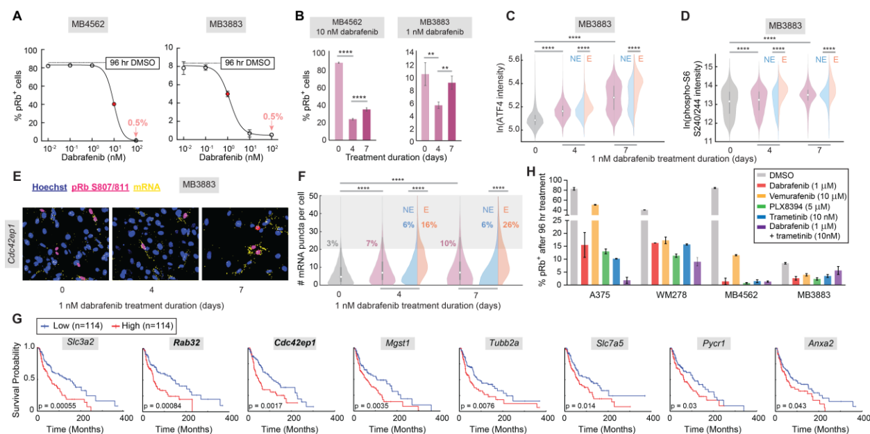
Fig. 3. Existence of escapees and upregulation of ATF4 target genes in clinical samples. (A) Dose response curves at 96 hr of treatment in two ex vivo patient cultures, noting a residual 0.5% of pRb + cells at the highest dose. IC 50 values used in further experiments are displayed as red dots. Error bars: mean ± std of 3 replicate wells. (B) Percentage of pRb + cells in the two patient samples treated with IC 50 dose of dabrafenib for 4 or 7 days. Error bars: mean ± std of 3 replicate wells. (C and D) Violin plots showing ATF4 and phospho-S6 (S240/244) levels by immunofluorescence in MB3883 patient cells treated with 1 nM dabrafenib for 0, 4, or 7 days. Escapees identified by phospho-Rb (S780) or EdU co-staining for ATF4 or phospho-S6, respectively. Each population value is pooled from 6 replicate wells. (E) RNA-FISH images for Cdc42ep1 with pRb (S807/811) and Hoechst staining, for MB3883 cells cultured in 1 nM dabrafenib for 0, 4, or 7 days. (F) Violin plot showing the number of Cdc42ep1 mRNA puncta in MB3883 cells. The percentage of cells with > 20 mRNA puncta is indicated on the plot. Each population value is pooled from 2 replicate wells. (G) Melanoma patient survival curves for 8 of 40 genes upregulated in escapees. (H) Percentage of pRb + cells in A375, WM278, and two ex vivo patient cultures treated with high doses of dabrafenib, vemurafenib, PLX8394, trametinib, or dabrafenib plus trametinib for 4 days. Error bars: mean ± std of at least 2 replicate wells.
