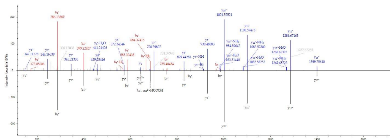
Figure 4. A mirror plot demonstrating the Prosit derived MS/MS spectra (bottom half) against the first known fragmentation pattern for this SARS-CoV-2 nucleocapsid peptide in the literature (top half)
