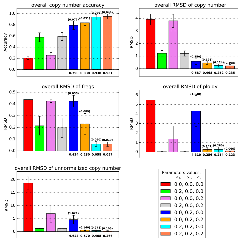
Fig. 1. Average accuracy and RMSD of the deconvolution without noise and without ploidy change (n=10). Each bar with different color represents a deconvolution model with different information. In the label table at the bottom right, the numbers represent the value of \alpha_f, \alpha_1, \alpha_2 , which are regularization terms for \|F - F'\| , J(S, C, C') and \|X^T C P - H'\| , respectively. 0.0 means the corresponding term is not included in the model. The number in parenthesis indicates the standard error of each model, the number under the bar indicate the mean of each model.
