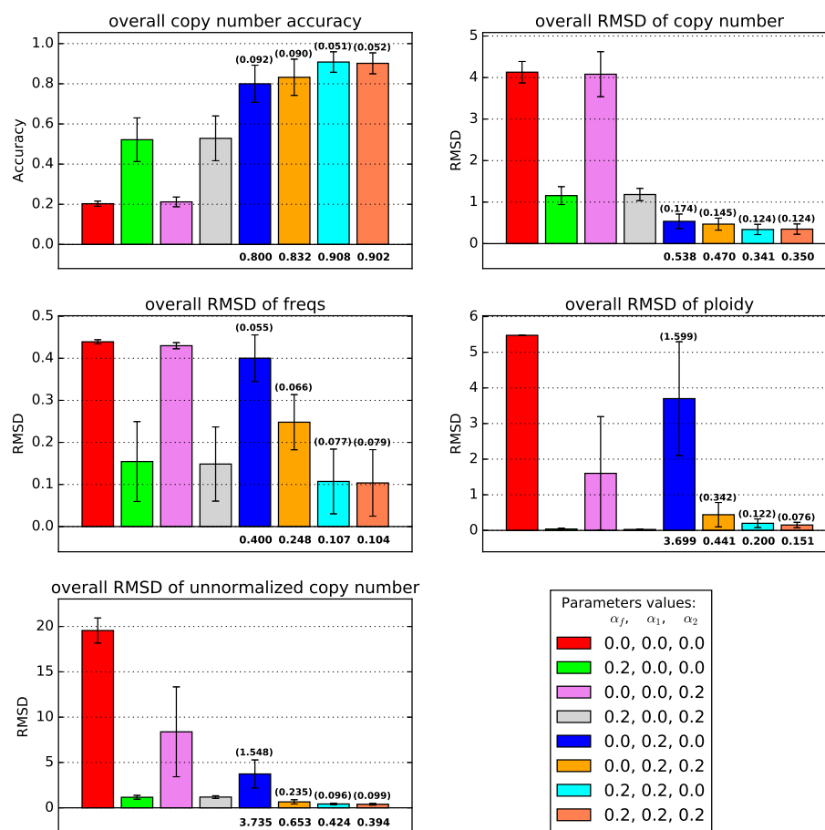
Fig. 2. Average accuracy and RMSD of the deconvolution with 10% noise and without ploidy change (n=10). Each bar with different color represents a deconvolution model with different information. In the label table at the bottom right, the numbers represent the value of \alpha_f , \alpha_1 , \alpha_2 , which are regularization terms for \|F - F'\| , J(S, C, C') and \|X^T C P - H'\| , respectively. 0.0 means the corresponding term is not included in the model. The number in parenthesis indicates the standard error of each model, the number under the bar indicate the mean of each model.
