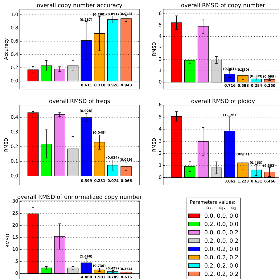
Fig.3. Average accuracy and RMSD of the deconvolution without noise and with ploidy change (n=10). Each bar with different color represents a deconvolution model with different information. In the label table at the bottom right, the numbers represent the value of \alpha_f, \alpha_1, \alpha_2 , which are regularization terms for \|F - F'\| , J(S, C, C') and \|X^T C P - H'\| , respectively. 0.0 means the corresponding term is not included in the model. The number in parenthesis indicates the standard error of each model, the number under the bar indicate the mean of each model.
