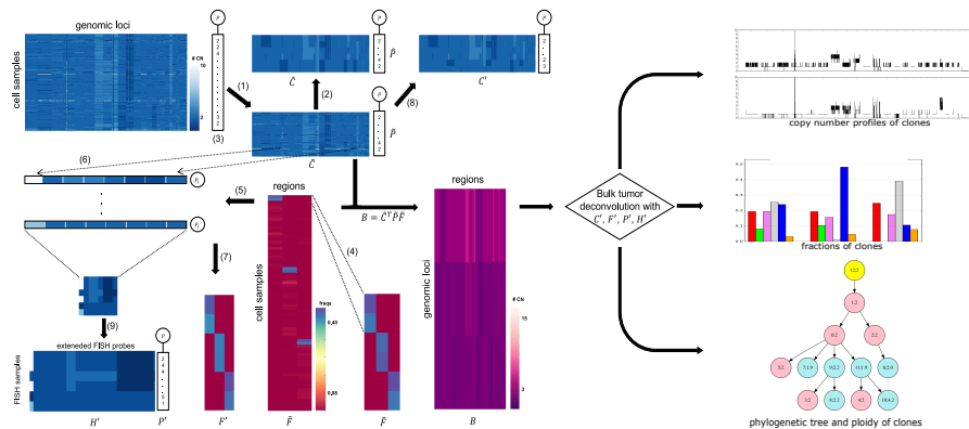
Fig.S2. Workflow of the simulation and deconvolution. The figure shows the process from real SCS data to select SCS clones, sample ploidies, simulate mixture fractions, simulate FISH and simulate bulk genomic data. We then deconvolve the bulk data into copy number profiles of a set of inferred clones each with a defined ploidy and set of mixture fractions across tumor regions, as well as a phylogenetic tree relating these clones. We then compare these outputs with the ground truth data to evaluate our model. Further methodological details are provided in the text. Note that the images in this figure are purely illustrative and do not show true data from any particular analysis.
