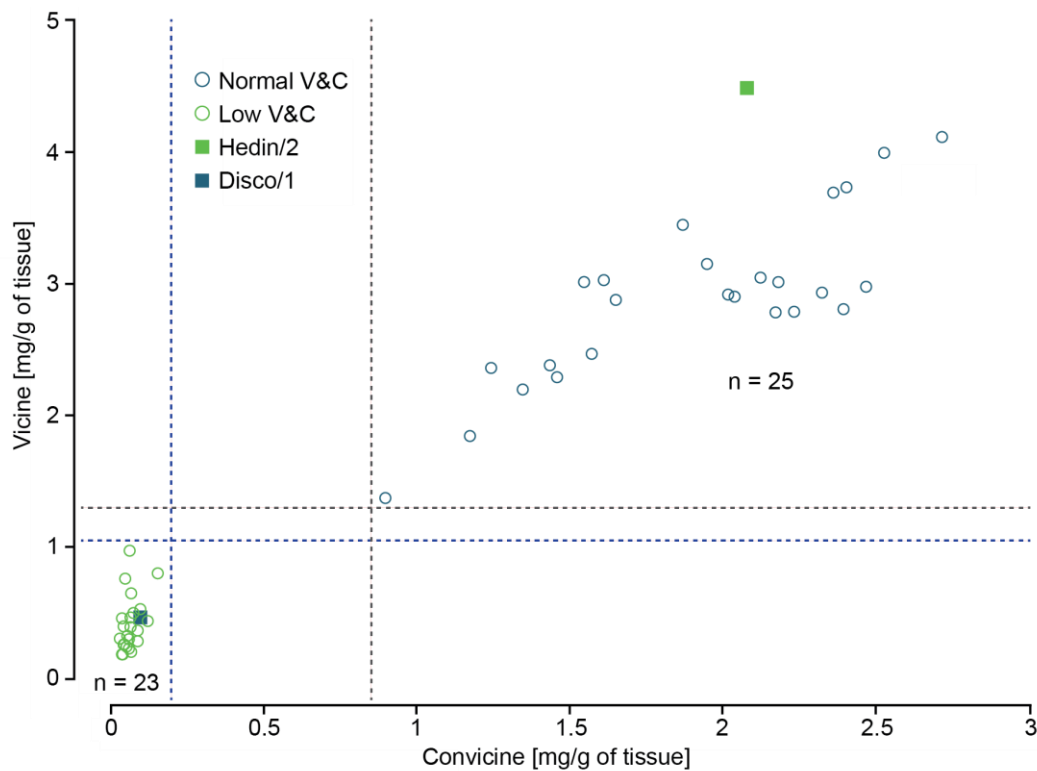
Extended Data Figure 2. Seed vicine and convicine phenotypes of Hedin/2 x Disco/1 pseudo-F2 recombinants within the vc^- interval. Recombinants are classified as Normal (blue open circles) where vicine levels are >1.3 mg/g and convicine levels are >0.85 mg/g or as Low (green open circles) where vicine levels are <1.05 mg/g and convicine levels are <0.2 mg/g. Parental means are shown as squares for Hedin/2 (green) and Disco/1 (blue).
