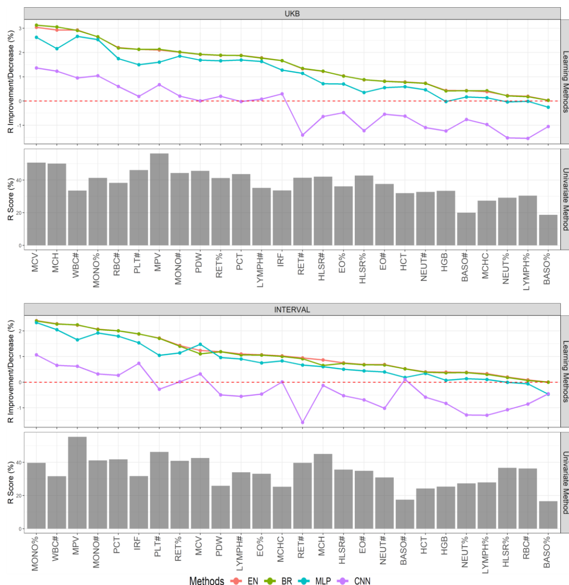
Figure 4. Performance comparison of different learning methods with the univariate method. Pearson r score performance of the UNI method for PGS construction of 26 blood cell traits are presented in testing on UKB or INTERVAL. Relative to the UNI method, performance of the four learning methods: EN, BR, MLP and CNN, are presented for each blood cell trait in descending order left to right according to EN (largest Pearson r increases on left). Given a particular method, a trait and a cohort, the averaged r performance of the 5 trained models, corresponding to the 5 different training-testing data partitions, is shown.
