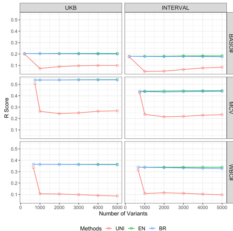
Figure S2. Performance of UNI, EN and BR methods on different sets of variants. Using CA variants as a base set, we increasingly add in the top significant variants by the step of 1000 (based on the GWASs on the UKB cohort) to form different sizes of variants sets, in which the CA variants are removed from the top significant variants list. It means the starting point of each curve is the r performance of the corresponding method on the CA variants set of a trait. We then observe the performance of BR, EN and UNI on different variants sets. Similarly, five models were trained corresponding to the five partitions of the UKB samples for each learning method, each trait and each variants set, whose r measurements are averaged in the figure. The results indicate that BR and EN are robust to redundancy in variants which appear to be through two different avenues: effect sizes of the CA variants generated by the two methods are very similar; however, EN tends to make the effect sizes of those non-contributing variants as zeros due to the use of L1 norm, while BR tends to make their effect sizes very small or can cancel each other due to the use of the L2 norm.
