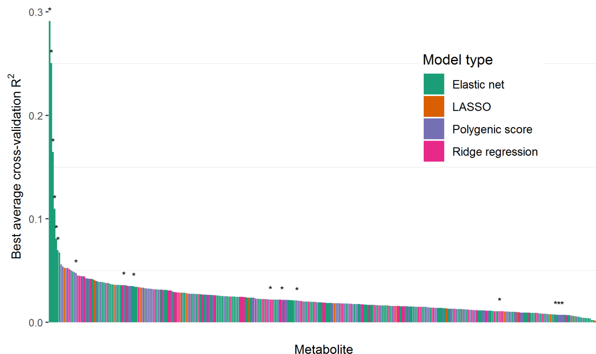
Figure 2. Metabolite prediction model performance. The prediction performance of the best model for each metabolite is shown arranged in order of decreasing R^2 . Metabolites with a significant locus from the GWAS meta-analysis are denoted with an asterisk.
