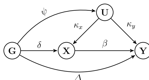
(b) Violations to IV assumptions
