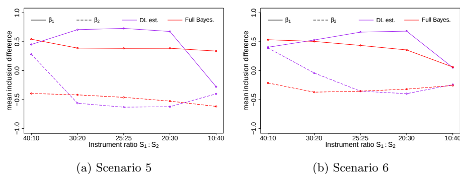
Fig. 3: Mean difference in inclusion probability between S_1 and S_2 as a function of the true ratio S_1:S_2 for Scenario 5 (a) and Scenario 6 (b).
