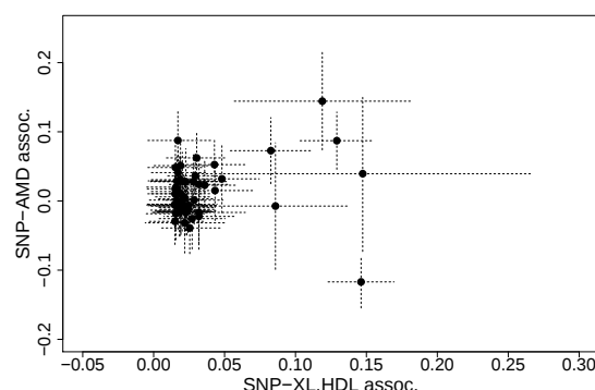
Fig. 4: AMD and HDL: Scatter plot of the relationship between SNP-outcome and SNP-exposure association.
