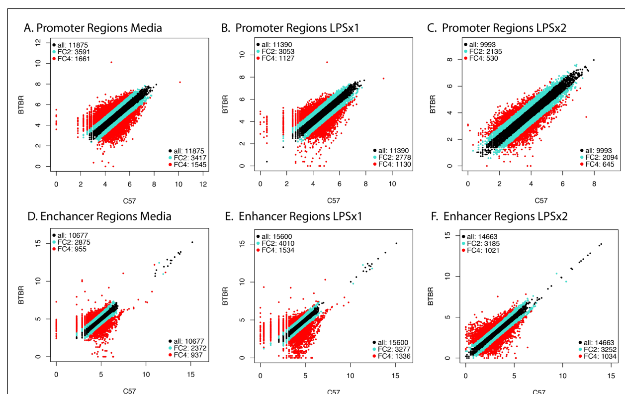
Figure 3. Correlation of quartile normalized ATAC-seq signal for all consensus peaks between strains. A. Promoter regions for C57 versus BTBR media peaks. B. Promoter regions for C57 versus BTBR LPSx1 peaks. C. Promoter regions for C57 versus BTBR LPSx2 peaks. D. Enhancer regions for C57 versus BTBR media peaks. E. Enhancer regions for C57 versus BTBR LPSx1 peaks. F. Enhancer regions for C57 versus BTBR LPSx2 peaks. For all panels, promoter regions were defined as within +/- 3kb of the nearest gene TSS. Enhancer regions were all other non-promoter regions. Fold change (FC) > +/-2 is highlighted teal and FC > +/-4 is highlighted red.
