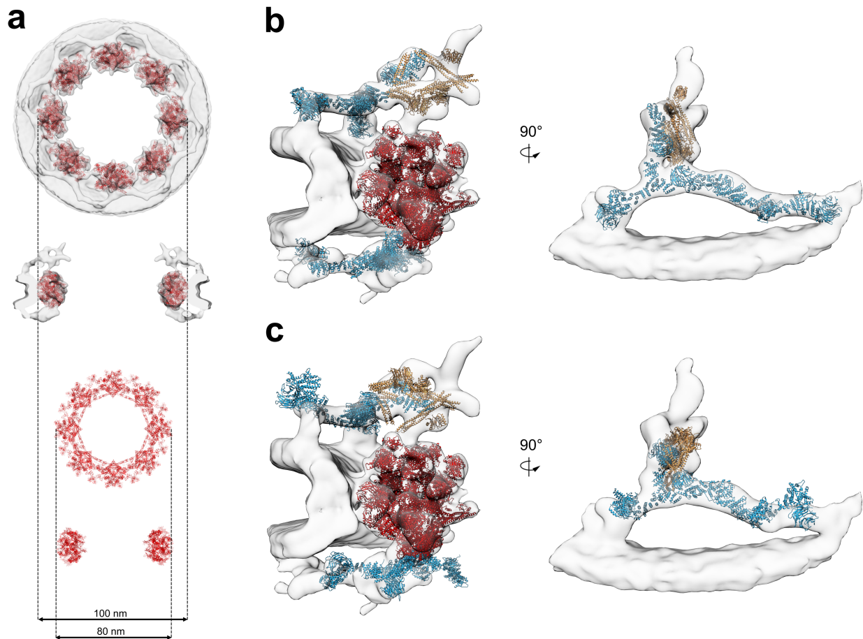
Extended Data Fig. 3: Architectural model of ScNPC. a , Comparison of fitted (to the cryo-ET map from this study, depicted in gray) integrative Inner Ring complex (IRC) models (red ribbons) from 13 with 20 nm diameter difference. b , Representative structural models of CR and NR Y-complex (blue ribbons), P-complex (yellow ribbons) and IR (red ribbons) built in this work (see Methods). The Y-complexes are more extended as compared to reference 13 version by ~40 Å. c , Representative integrative structural models of CR and NR Y-complex (blue ribbons), P-complex (yellow ribbons) and inner ring complex (red ribbons) from 13 fitted to cryo-ET map (grey density) from this study, with respect to spatial reference frame from 13 .
