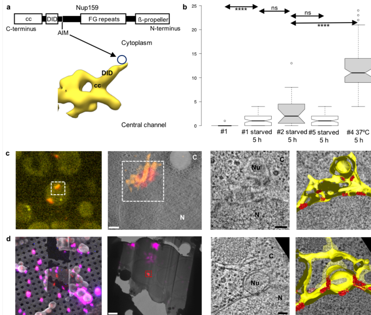
Fig. 3: Cellular visualization of Nup159-Atg8 interaction by CLEM. a , Domain structure of Nup159 with corresponding map showing the position of the Atg8 interacting motif (AIM) (Lee et al). b , Box plot (median, 1st quartile) showing the number of herniae (see Methods) in S. cerevisiae strains before and after starvation according to Extended Data Table 1 (#1 control cells; #2 Nup159-Atg8-splitVenus, Nup170-Mars, nup120Δ cells; #4 nup116Δ cells; #5 atg8Δ cells). nup116Δ cells (#4) were shifted to the non-permissive Temperature of 37°C; herniae are induced (**** p < 0.0001 ; Mann Whitney, two-sided). c , On section CLEM of strain #2 after 5.5h of starvation. The left panel shows the light microscopy signal on plastic section. SplitVenus signal arising from the interaction of Nup159 with Atg8 is shown in yellow. Nup170-Mars is shown in red. The second panel zooms in the area of interest (white dashed square in the previous panel) showing the overlay of the fluorescent signal on the tomographic EM slice. Scale bar: 200 nm. The framed area is shown as tomographic slice and segmented on the right (N nucleus; C cytoplasm; Nu nucleoplasm; scale bar: 100 nm; NPCs in red; membranes in yellow). d , 3D cryo-CLEM of strain #2 after 5.5 h of starvation. SEM top view of a lamella with overlaid fluorescent signal. Red is NPC signal; magenta is fiducial-bead signal. Second panel: cryo-TEM overview (~2
