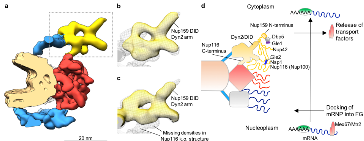
Fig. 2: Nup159 complex architecture. a , Individual spoke of the ScNPC (color-code as in Fig. 1). Nup159 complex is highlighted with a dotted frame. b , Nup159 complex region of the in cell ScNPC map (gray mesh) superimposed with the top scoring systematic fit (see Methods) of the negative stain map of the Nup159 complex 4 (yellow surface). c , Same as b but superimposed with the in cell ScNPC map of a nup116Δ strain grown at permissive temperature (yellow surface). d , Spatial model of how mRNA export is accommodated by the orientation of the Nup159 complex. A poly-A mRNA with transport factors Mex67/Mtr2 (red) and proteins that protect the poly-A tail from degradation (light green) docks to the unstructured region of the basket Nups 5 (grey box with blue filaments). Nup159 N-terminal domain that mediates the release of the transport factors from the mRNA 7 is anchored at the cytoplasmic side.
