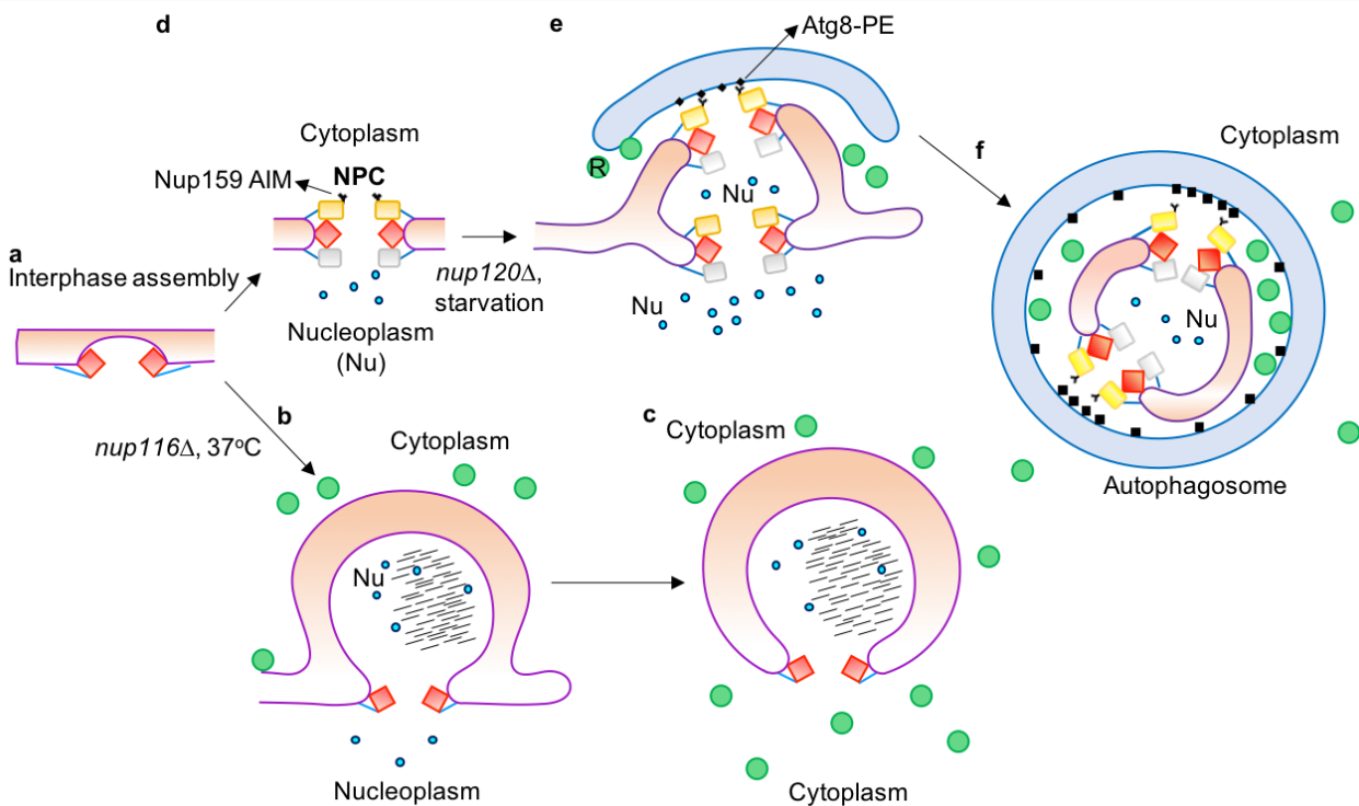
Fig. 4: Cartoon model of membrane remodeling during NPC turnover by selective autophagy. a , Inside-out assembly intermediates 34 or inner nuclear membrane evaginations (Extended Data Fig. 6d) progress into b , NE herniae as in the nup116Δ strain at non-permissive temperature (Extended Data Fig. 6a); or mature into d , fully assembled NPCs. e , When autophagy is triggered by Nitrogen starvation (or NPC clustering), NPCs are cytoplasmically exposed at the herniations by membrane remodeling (Fig. 3 c-d, Supplementary Video 1). Nup159 AIM interacts with Atg8 and double membranes are recruited to the nuclear envelope. c , If hernia accumulation is enforced in nup116Δ cells at non permissive temperature, nuclear vesicles are observed in the cytosol. e , f , If autophagy is triggered, nuclear vesicles are engulfed by double membranes (Extended Data Fig. 7c) and, as shown by Lee et al, ultimately end up in the lysosome (Extended Data Fig. 9g). Color-code as in Fig. 2d. R is ribosome depicted as a green circle; black lines represent dark densities visible in the cryo-tomograms.
