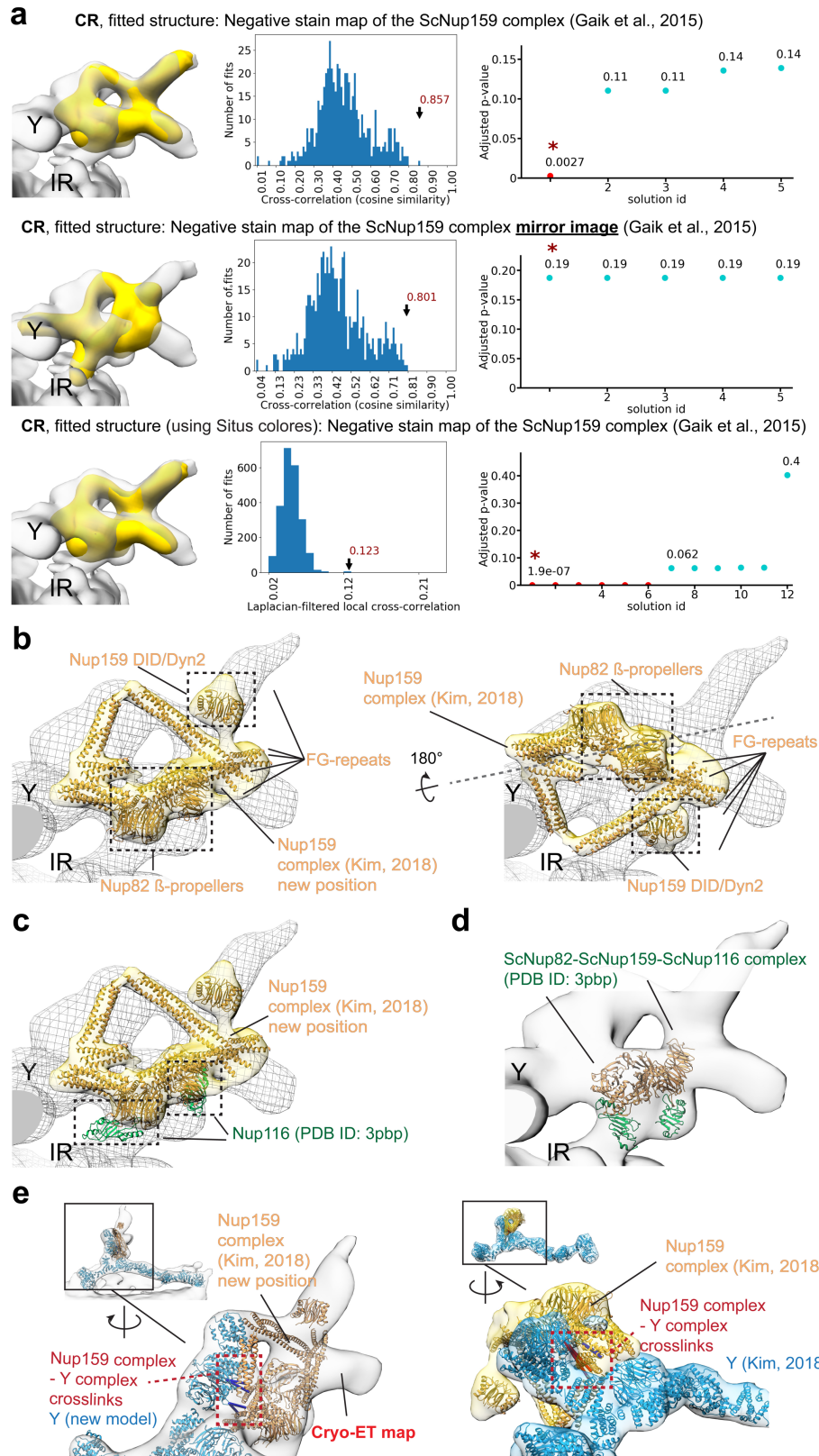
Extended Data Fig. 4: Validation of the orientation of the Nup159 complex. a, Systematic fitting of the negative stain map of the Nup159 complex into the ScNPC map using UCSF
