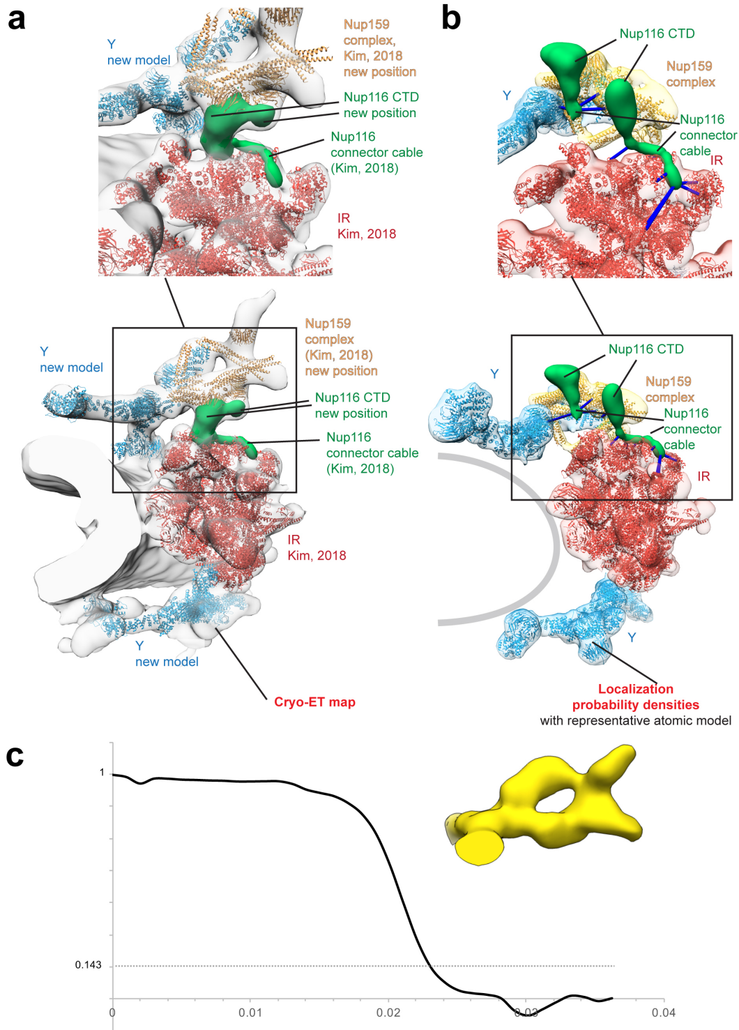
Extended Data Fig. 5: Nup116 positioning. a , New positioning of the Nup116 (left) versus previously published integrative model (PDB DEV ID: 00000010 from 13 , right). The two Sc NPC models were superimposed such that the IRs are aligned to the same reference frame. The Nup116 position is shown either as the density assigned to Nup116 based on the Nup116 knock-out structure (left) or as localization probability densities retrieved from reference 13 model (right). The
