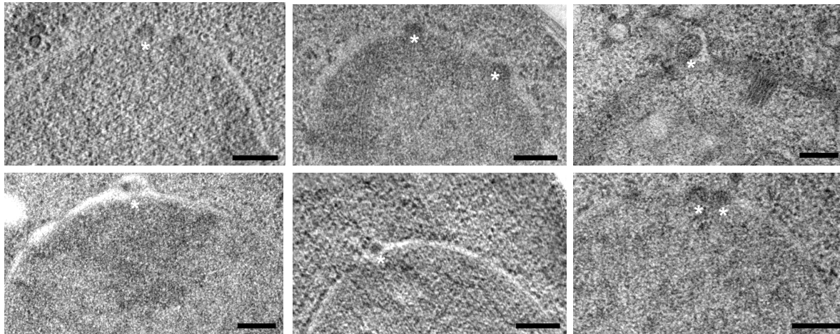
Extended Data Fig. 8: Herniations under atg8Δ conditions after 5h of nitrogen starvation. Small herniations appears in the nuclear envelope and are marked with *. Statistics in Figure 3b. Scale bar: 200 nm.
