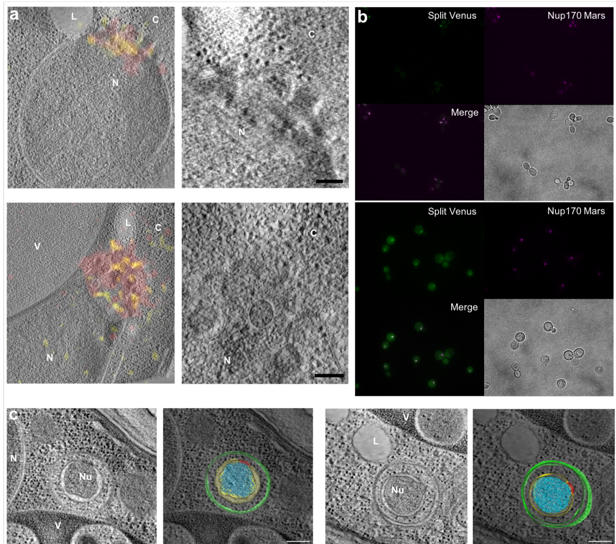
Extended Data Fig. 7: Snapshots of selective autophagy at the nuclear envelope. a , Gallery of tomographic slices overlaid with fluorescence images as obtained by on section-CLEM of Nup170-Mars, Nup159-Atg8-SplitVenus cells. The Nup159-Atg8 interaction is observed as the yellow SplitVenus signal, Nup170-Mars is shown in red. In the right panel, zoomed views of the same tomographic slices are shown, emphasizing the clustering of herniae and nuclear vesicles arising through further membrane remodeling (See also Fig. 3 c-d and Supplementary Video 1). N is nucleus, V is vacuole, L is lipid droplet, C is cytoplasm. Scale bar: 100 nm. b , Fluorescence and phase contrast microscopy images of Nup170-Mars (magenta), Nup159-Atg8-SplitVenus (green) cells before (top) and after 5.5h of nitrogen starvation (bottom). Upon starvation, Nup159-Atg8-SplitVenus signal increases and co-localizes with Nup170-Mars (white dots). c , tomographic slice (left) as well as the corresponding segmentation and isosurface rendering (right) of NPC-containing nuclear vesicles (~340 nm in diameter) observed in the cytoplasm. They are surrounded by cytosol content (ribosomes) and another two membranes (~540 nm in diameter). Sce atg15Δ
