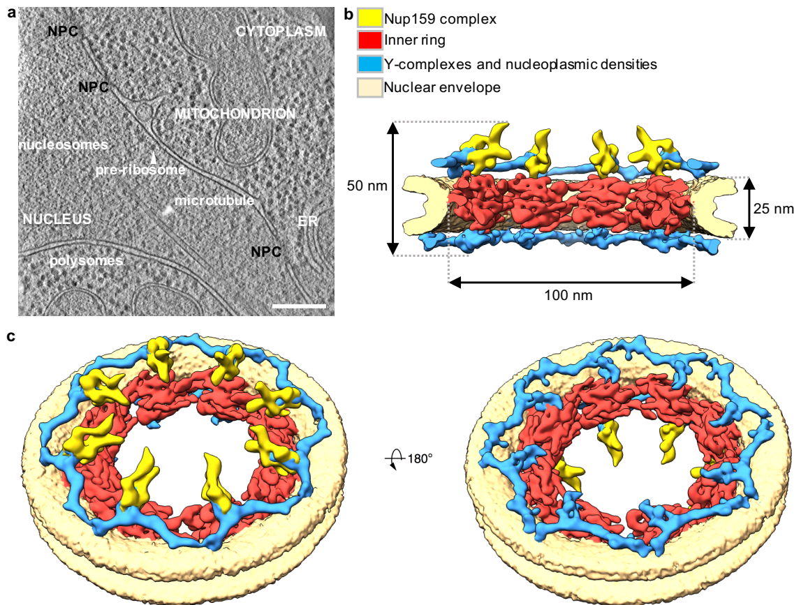
Fig. 1: In cell structure of S. cerevisiae NPC. a , Tomographic slice of a S. cerevisiae cell during division. Scale bar 200 nm. b , Segmentation of the cryo-EM map of the ScNPC cut in half. c , Tilted view of the entire NPC showing both the cytoplasmic (left) and the nucleoplasmic (right) face.
