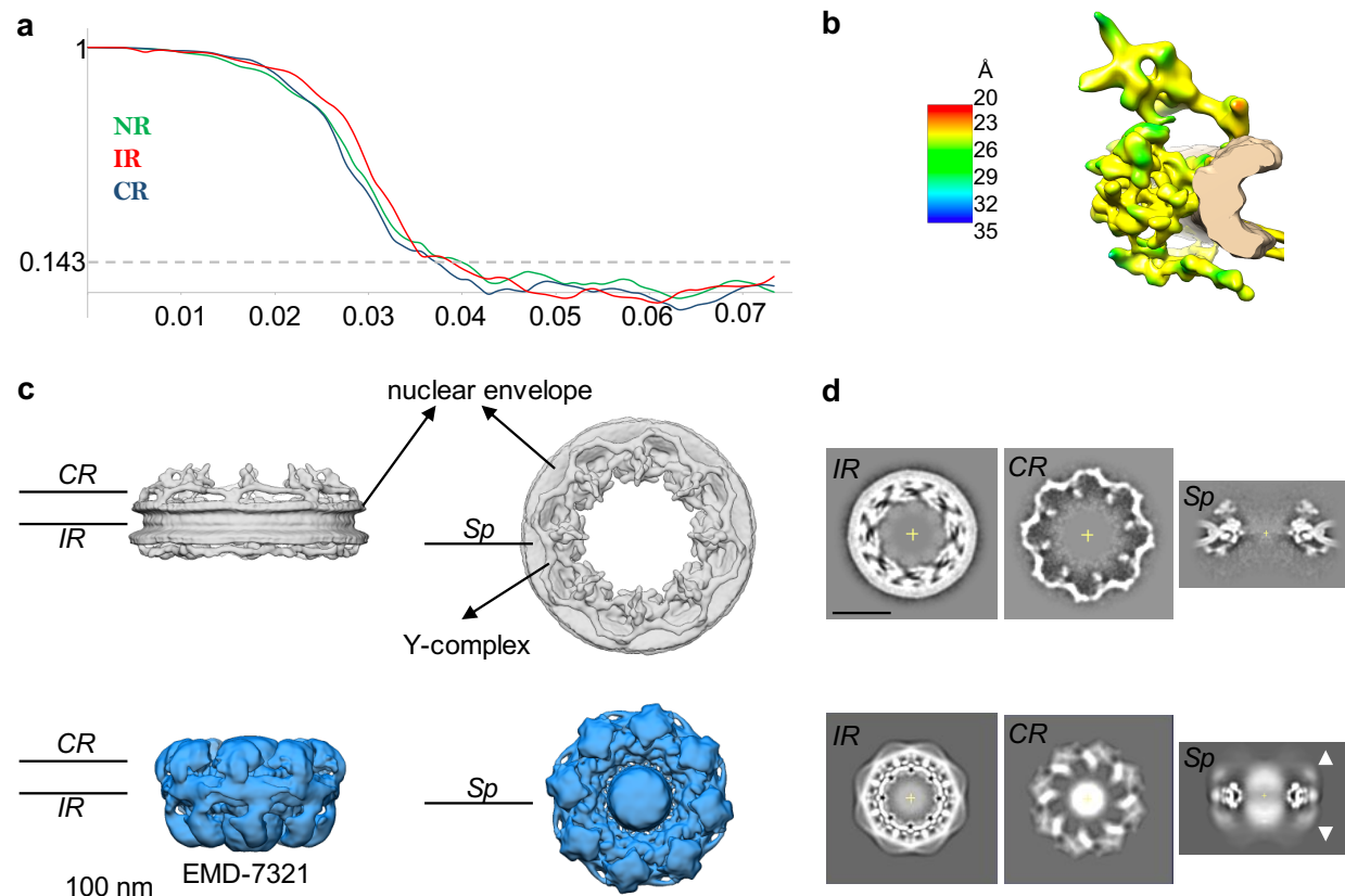
Extended Data Fig. 1: In cell structure of the ScNPC vs detergent-extracted ScNPC (EMD-7321). a , Gold standard FSCs of in cell cryo-EM map of the ScNPC. All the curves (nuclear ring NR, cytoplasmic ring CR, inner ring IR) intersect the 0.143 criterium at around 25 Å resolution. b , Local resolution analysis 51 with color-coded bar. c , In cell cryo-EM map (gray) in comparison to cryo-EM map of detergent-extracted ScNPCs (blue, EMD-7321 at the suggested contour level) show significant differences in diameter and in interpretable features. The nuclear membranes and the Y-complexes are clearly discerned in the in cell cryo-EM map, in contrast to EMD-7321. d , Slices through the maps at the level of the cytoplasmic (CR) and inner rings (IR) and an individual spoke (Sp). Lines in c indicate slicing position shown in d . Arrowheads indicate blurred features in the outer rings. Scale bar: 50 nm. See also: Source Data 1 attached for review process.
