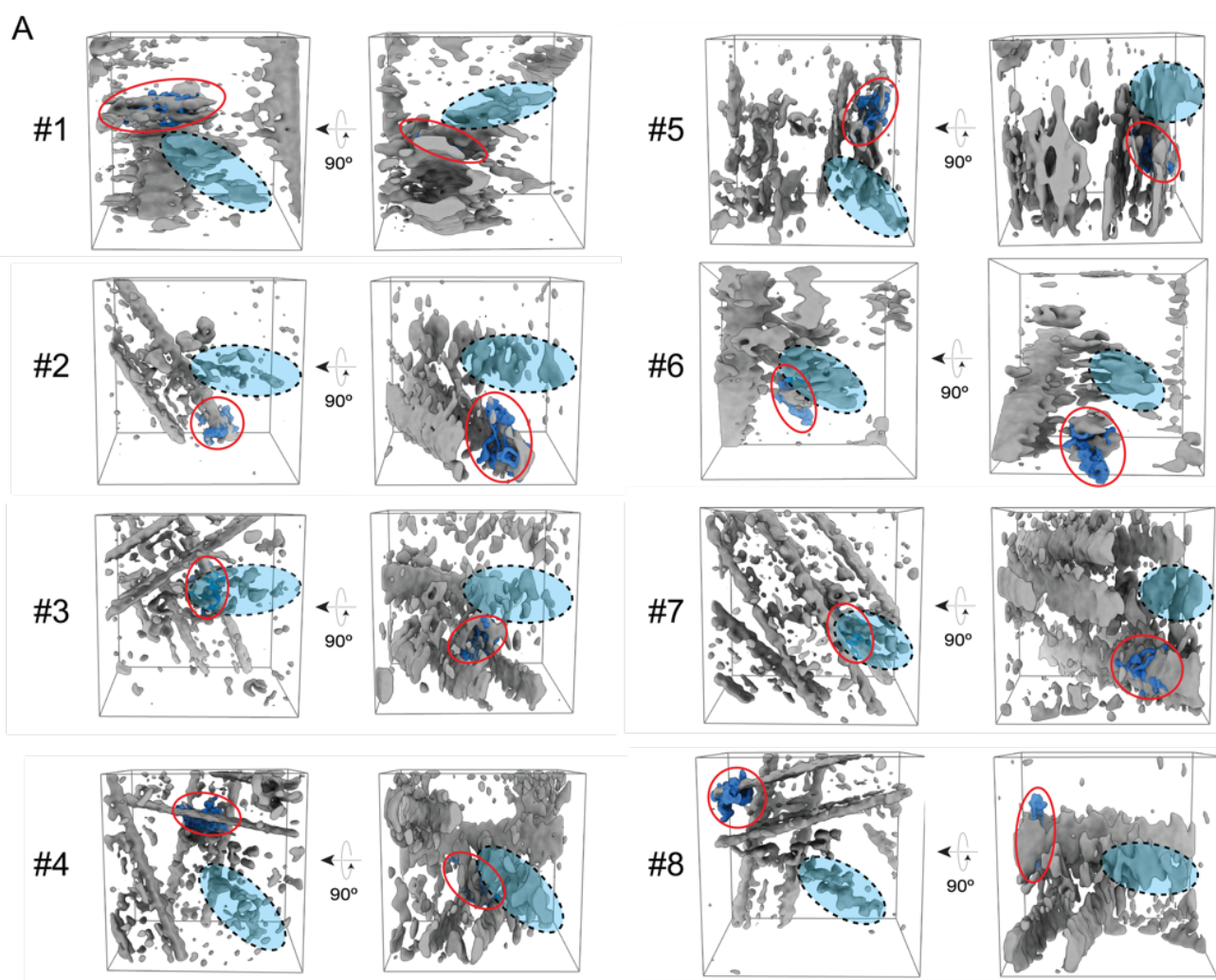
Figure 6. Failed attempts to automate docking of reference structure. A. Representative subvolumes (#1-8, in gray) with the position of the dynactin portion of the dynein-dynactin complex highlighted with a light blue oval outlined in black dashed lines. Red circles indicate the position of the guide structure (EMD-2860, dark blue) with the highest cross-correlation score docked in the subvolume, as determined by the UCSF Chimera “Fit in map” program. In all cases, the position with the highest cross-correlation score (red circle) does not overlap with the correct position of dynactin within the guide structure (light blue oval outlined in black dashed lines), demonstrating the difficulty in utilizing automated approaches to manually dock in guide structures into extracted subvolumes of the dynein-dynactin complexes. Due to this low success rate of correctly docked structures using this approach, initial manual docking of reference structure into extracted subvolumes was used for successful execution of the guided approach for dynein-dynactin complex.
