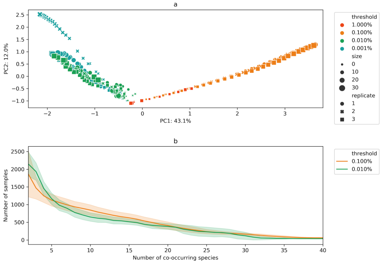
Supplementary Figure 2: a) Principal component analysis of co-occurring communities computed using different abundance thresholds. Marker size indicates co-occurring community size (up to 30 species) and marker shapes indicates independent runs of the algorithm (3 runs for each threshold); b) Average number of samples where all species in a co-occurring community can be found together as a function of community size (computed for the threshold values used in this work).
