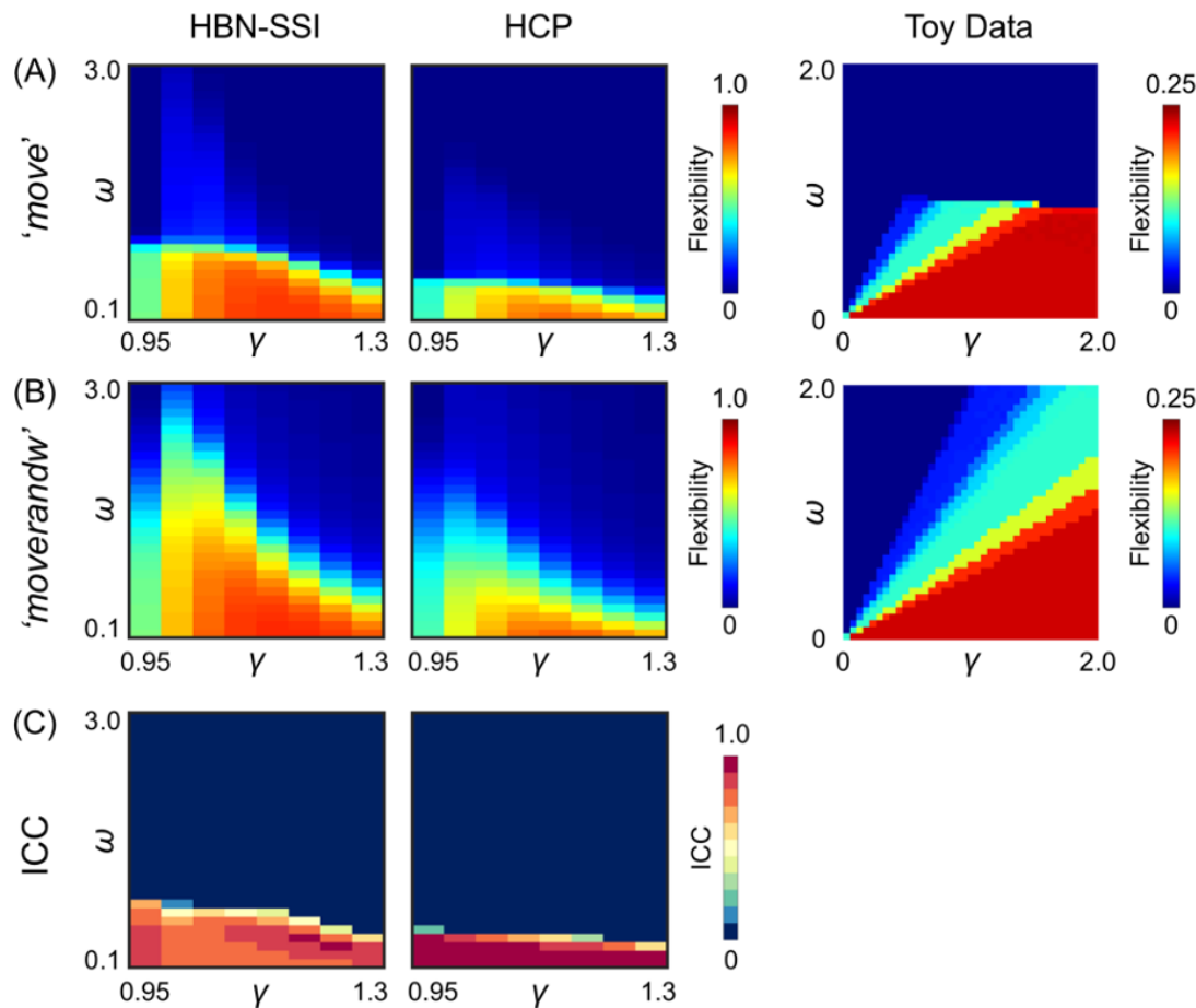
Figure 1. The impact of GenLouvain method ( ‘move’ vs ‘moverandw’ ) on estimated values of flexibility. When the default option ‘move’ was used (A), there was a drop-off in flexibility values in the 2-dimensional \gamma - \omega parameter space. This apparent discontinuity was observed on flexibility values in two independent human brain imaging datasets, Healthy Brain Network-Serial Scanning Initiative (HBN-SSI) and Human Connectome Project (HCP), as well as in toy data. The issue was mitigated by the added option ‘moverandw’ (B). Reliability between the two randomization options quantified using intra-class correlation coefficients (ICCs) was high before the apparent discontinuity and was near zero above the discontinuity (C). ICCs for HBN-SSI and HCP were evaluated based on 60 minutes of resting state data.
