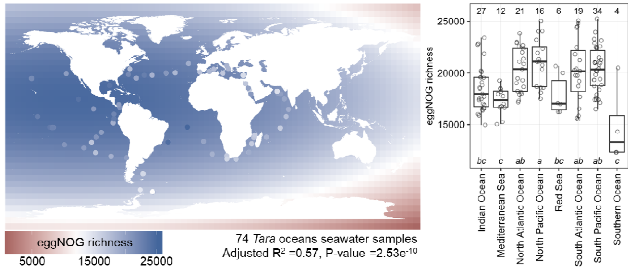
Figure 2: Global distribution of functional richness as eggNOG gene families from metagenomes in 20L seawater samples from 68 locations waters across to globe using non-parametric smoothing for 1x1 grid cells by additive second-degree polynomial models for latitude, longitude, temperature, concentration of nitrate, oxygen and phosphate, and generation time. Including nitrate concentration (AIC =1,138.6) showed the lowest AIC compared to the basic model with latitude and longitude (AIC =1,360.4) and the model with all environmental variables (AIC =1,115.7). The additive pairing of first- or second-degree polynomial terms for latitude, longitude and nitrate concentration showed the lowest AIC value when a first-degree polynomial term is used for nitrate concentration combined with second-degree polynomial terms for latitude and longitude (AIC =1,136.7). The functional richness is also shown based on the region of the different waters with the number of samples as numbers. Groups followed by the same letter are not significantly different according to the HSD test (P-value >0.05).
