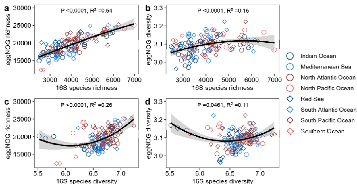
Figure 1: The relationships as smoothed averages between species richness and diversity from 16S metabarcoding and functional richness or diversity of eggNOG functions from metagenomes in 20L seawater samples from 68 locations waters across to globe. The adjusted coefficient of determination ( R^2 ) is given for the best fitting model for each equation: quadratic (a), logarithmic (b), quadratic (c) and linear (d). The P-value was determined by Spearman's rank correlation.
